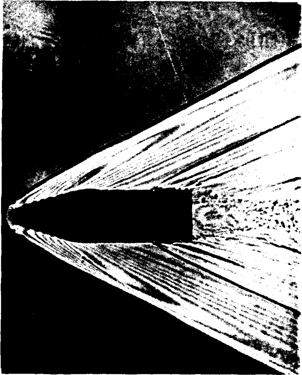
Figure 22. Dark Central Ground Interferogram
