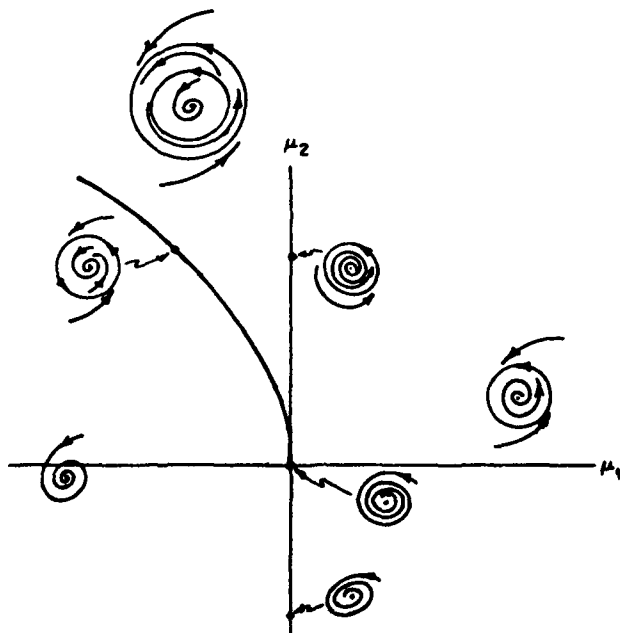
fig. 11 - The generalised Hopf bifurcation, a_2 < 0 case.
