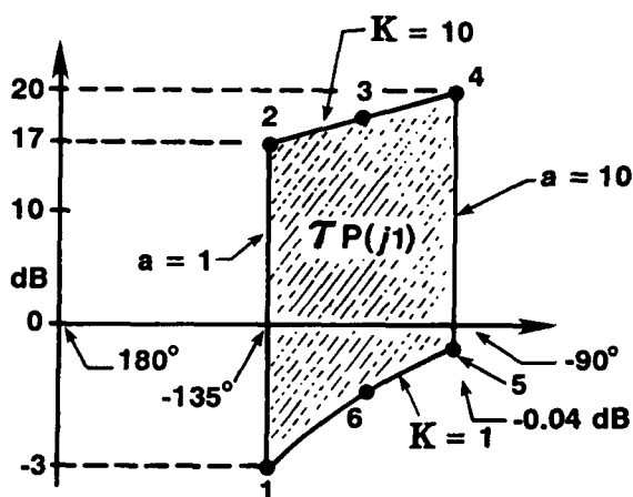
Fig. 8 The template TP(j1)
