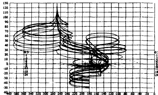
Fig. 25 L_{1i}(j\omega) plots for 36 cases and M_L -contour
