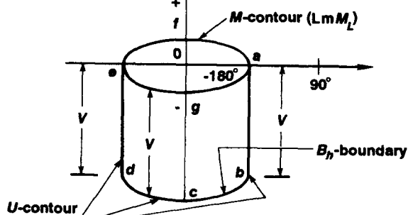
Fig. 9 U-contour construction
