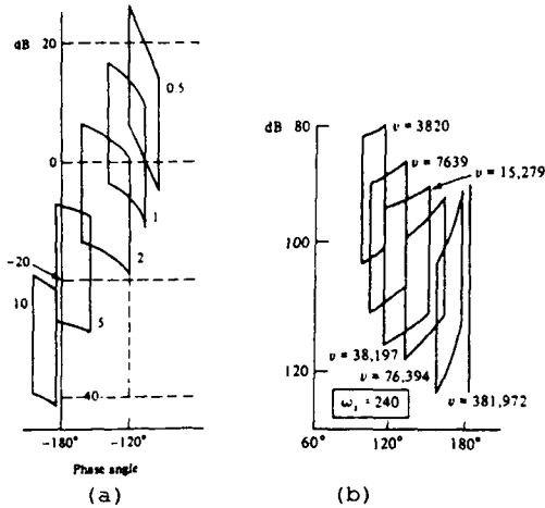
Fig. 16 w-domain plant templates
