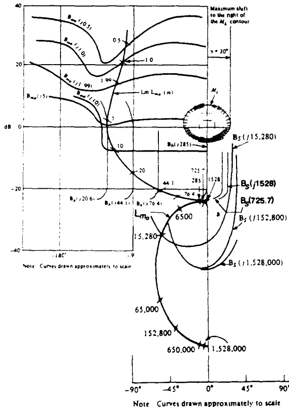
Fig. 17 A satisfactory design: L_{mo}(jv) at \omega_s = 240 .
