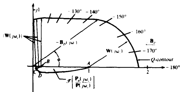
Fig. 10 Graphical evaluation of B_D(j\omega_i)
