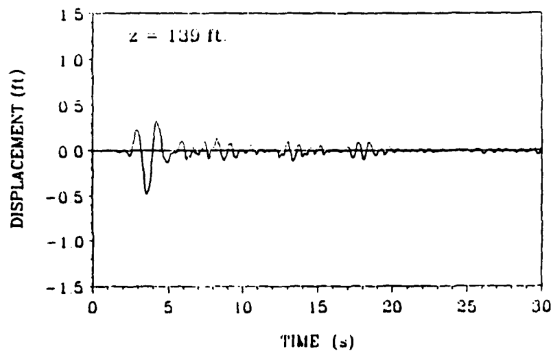
Figure 6.2 Case 2: Displacement time histories at various elevations within the dam 92
