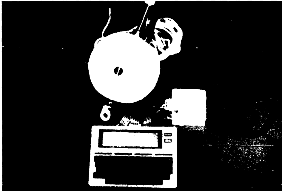
Figure A5. InterOceans S-4 current meter
