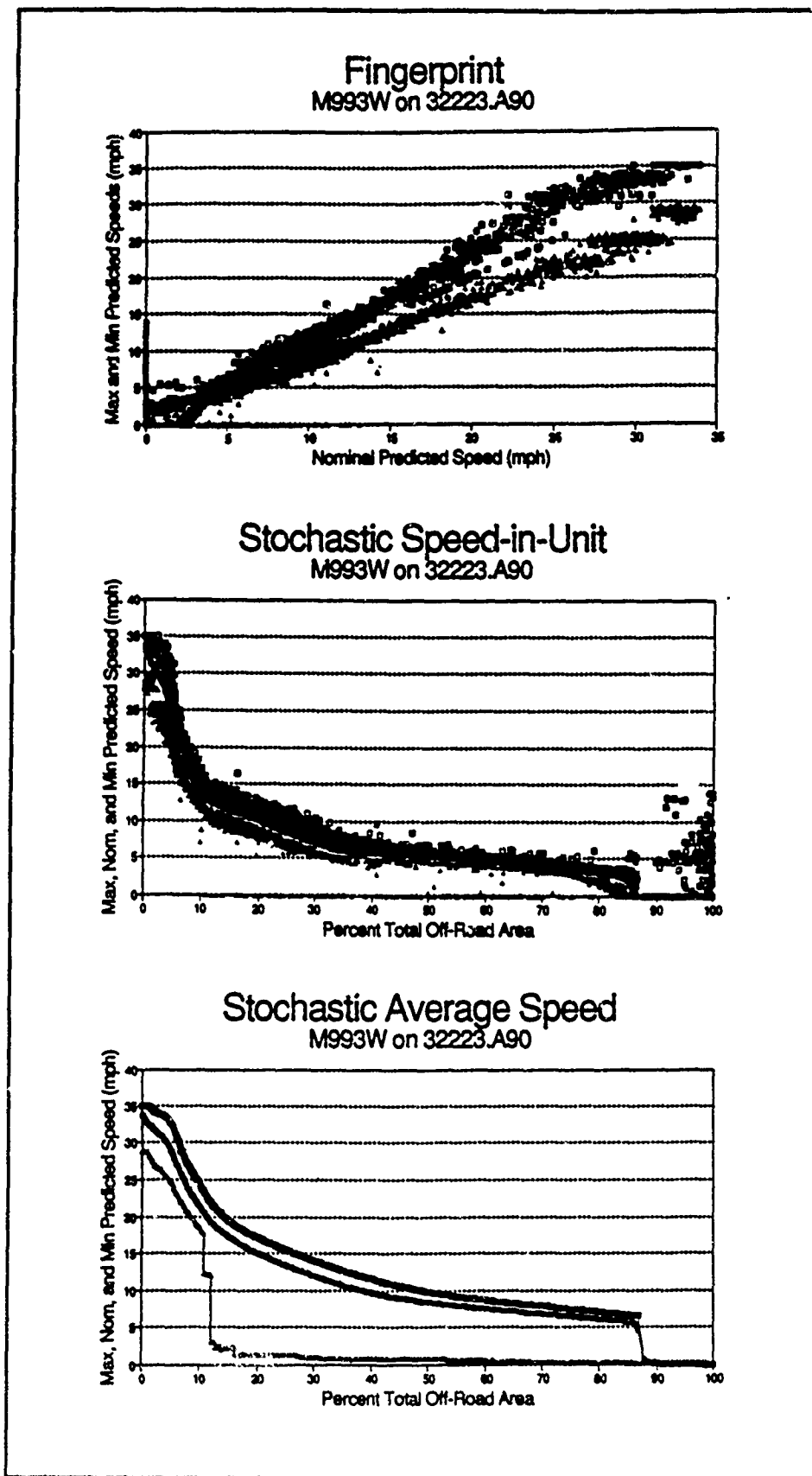
Figure 87. Fingerprint and profiles for M993 on ROK off-road
