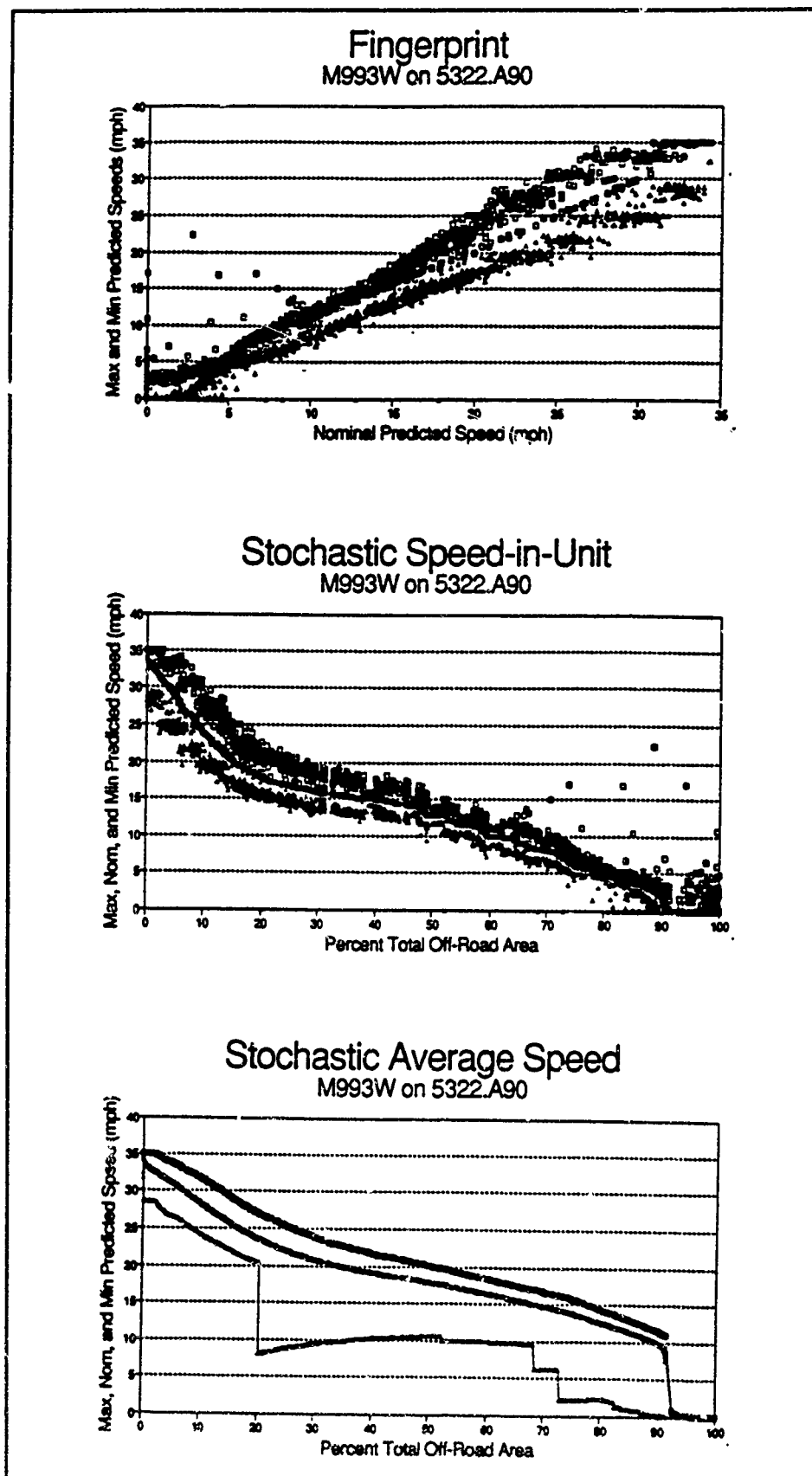
Figure 59. Fingerprint and profiles for M993 on WGe off-road
