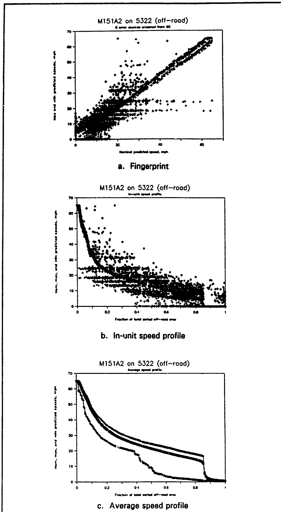
Figure 31. Fingerprints and speed profiles for M151 on Lauterbach
