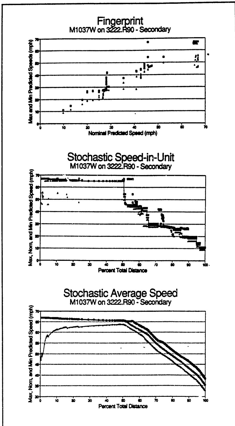
Figure 101.Fingerprint and profiles for M1037 on ROK secondary roads
