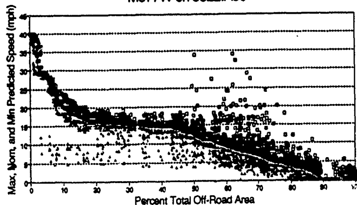
Figure 63. Fingerprint and profiles for M977 on WGe off-road
