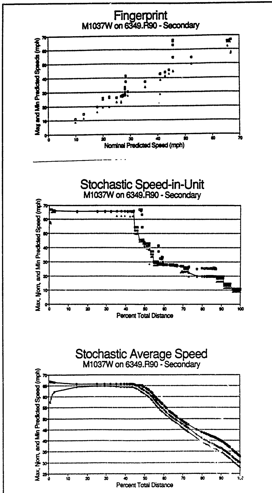
Figure 85. Fingerprint and profiles for M1037 on SWA secondary roads
