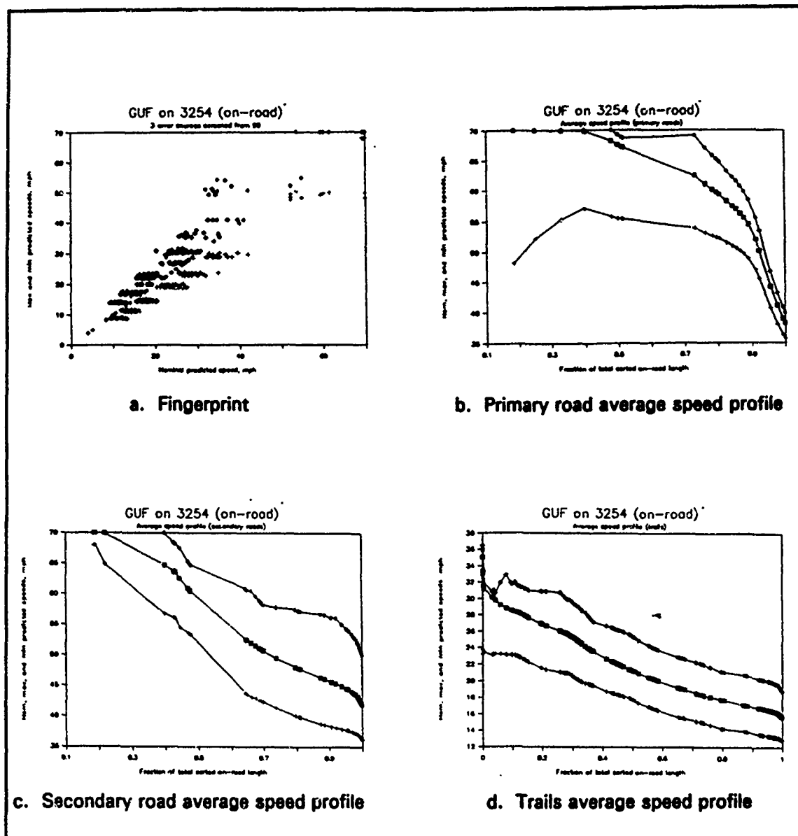
Figure 26. Fingerprint and speed profiles for GUF on Az Zarqa
