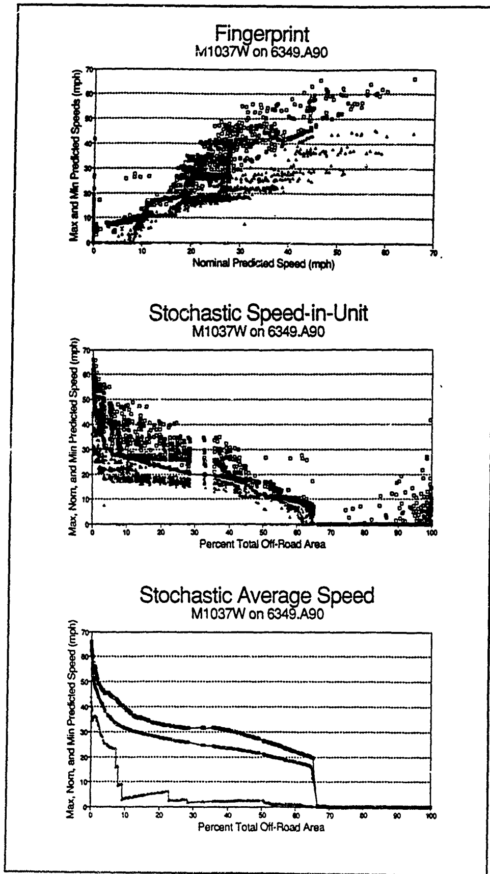
Figure 84. Fingerprint and profiles for M1037 on SWA off-road
