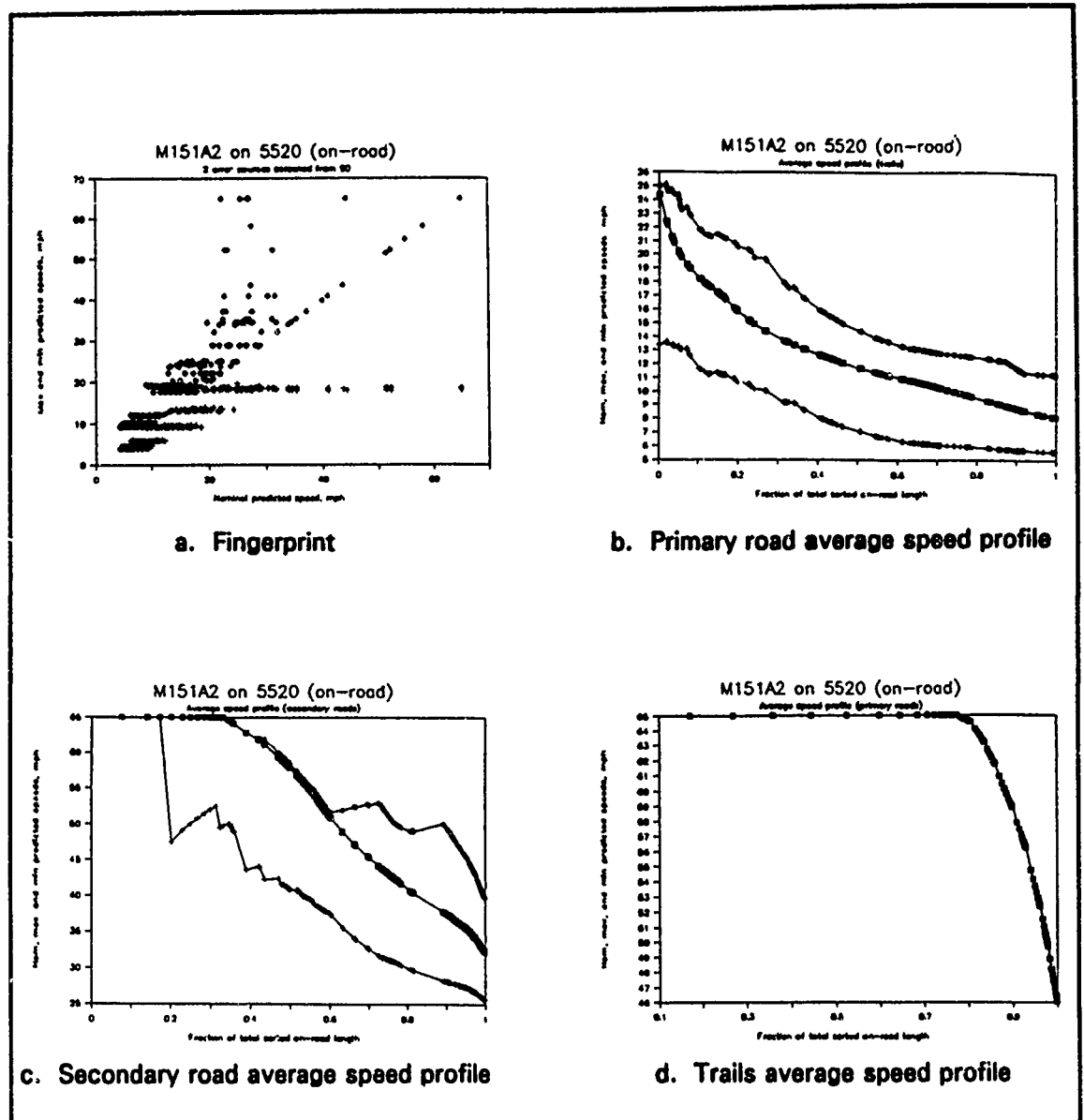
Figure 32. Fingerprint and speed profiles for M151 on Schotten
