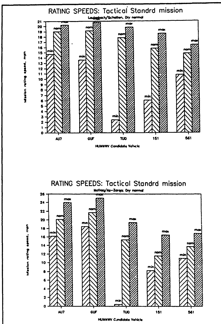
Figure 40. Mission rating speeds for the Tactical Standard mission
