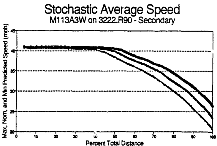
Figure 9/. Fingerprint and profiles for M113A3 on ROK secondary roads
