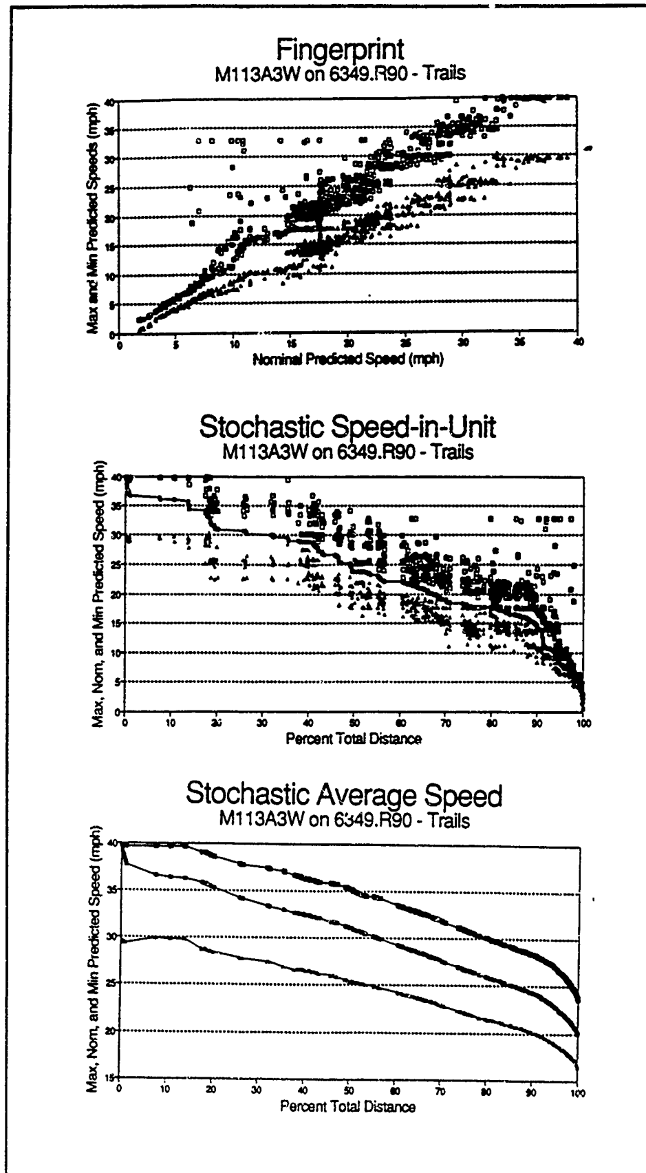
Figure 83. Fingerprint and profiles for M113A3 on SWA trails
