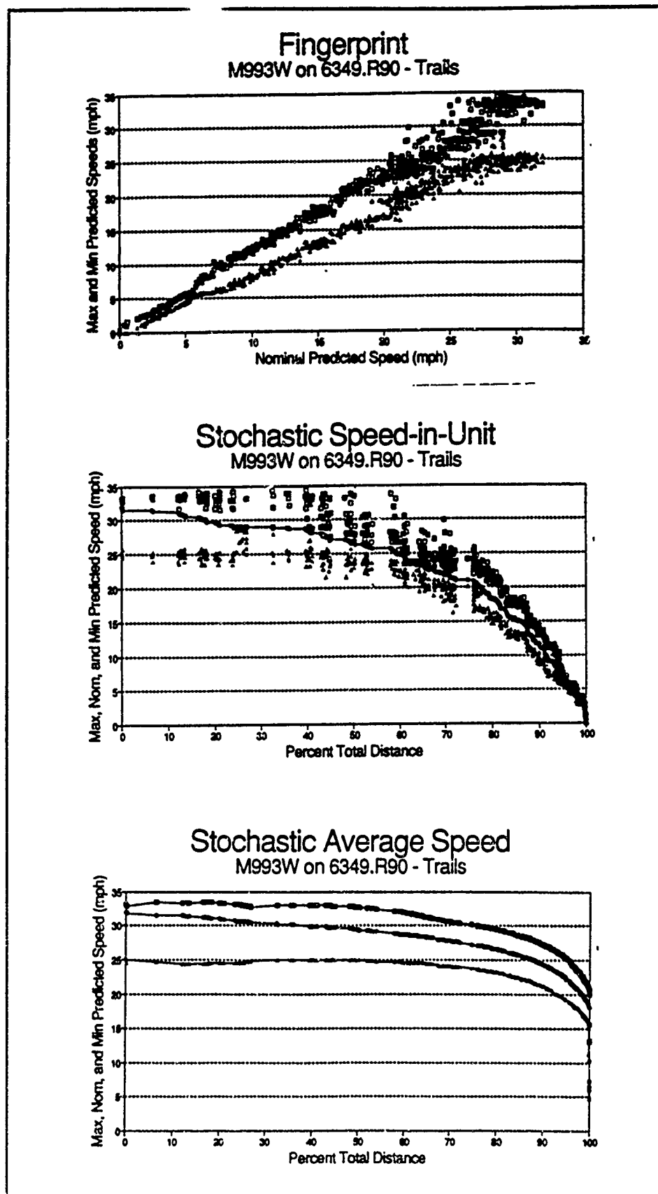
Figure 77. Fingerprint and profiles for M993 on SWA trails
