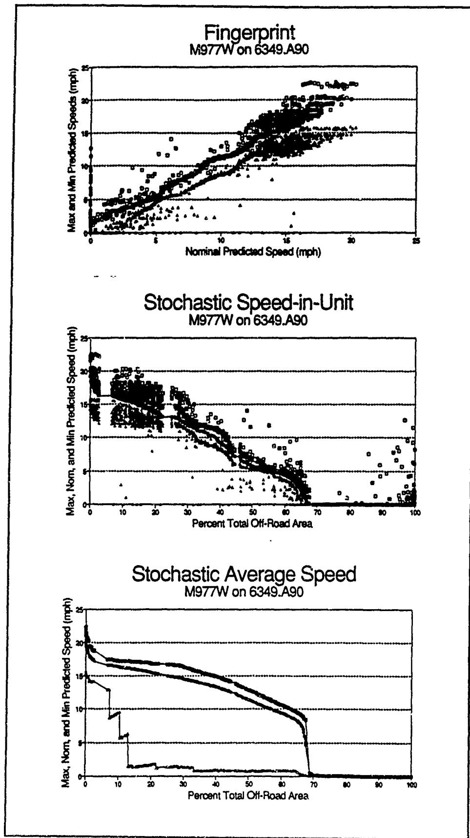
Figure 78. Fingerprint and profiles for M977 on SWA off-road
