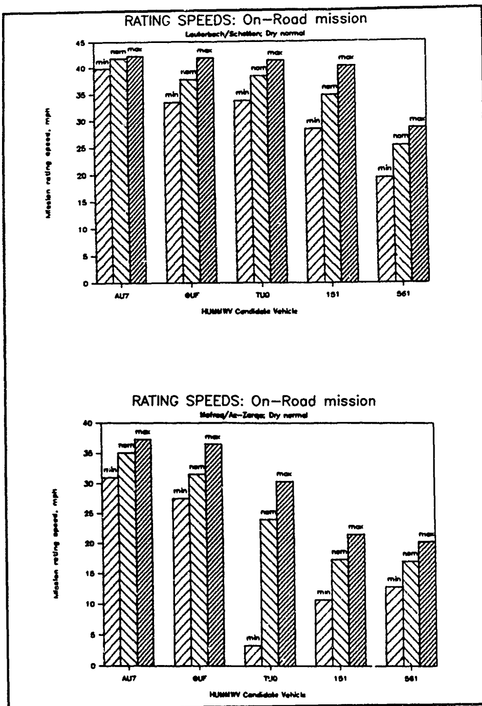
Figure 42. Mission rating speeds for the On-Road mobility mission
