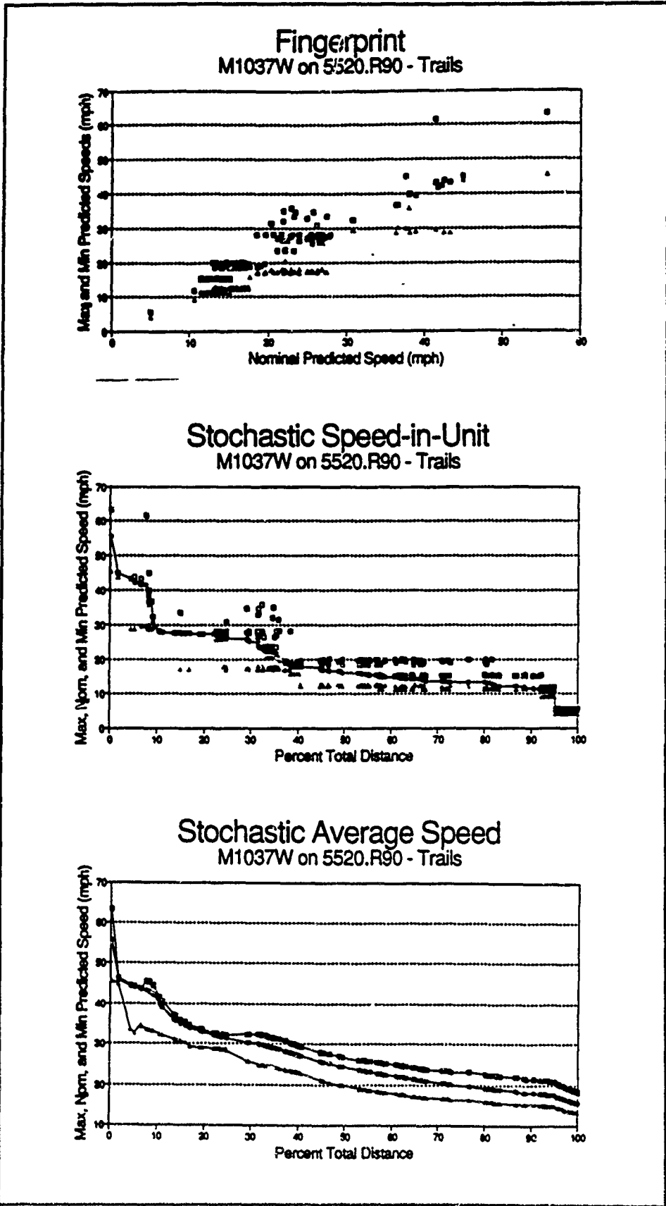
Figure 74. Fingerprint and profiles for M1037 on WGe trails
