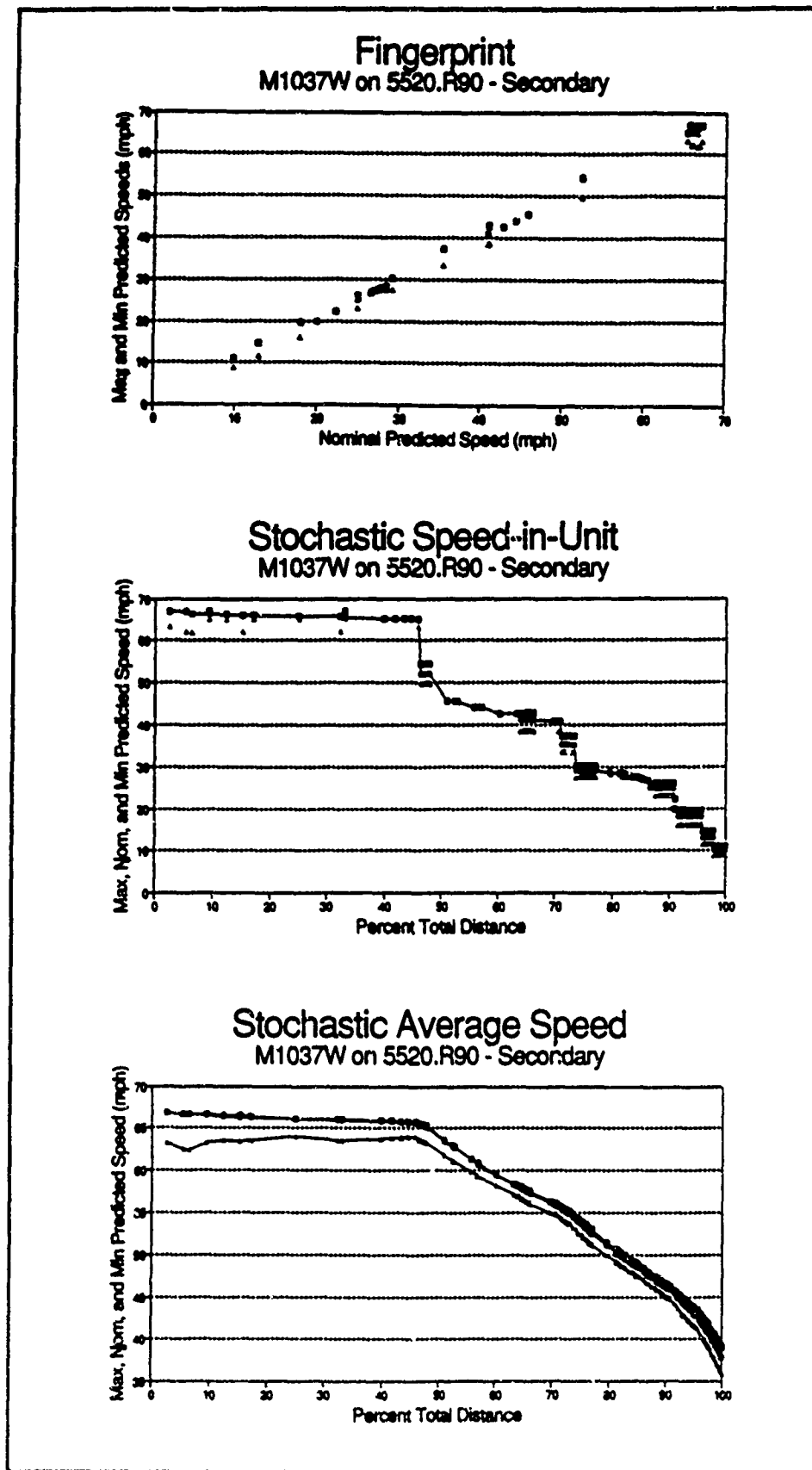
Figure 73. Fingerprint and profiles for M1037 on WGe secondary roads
