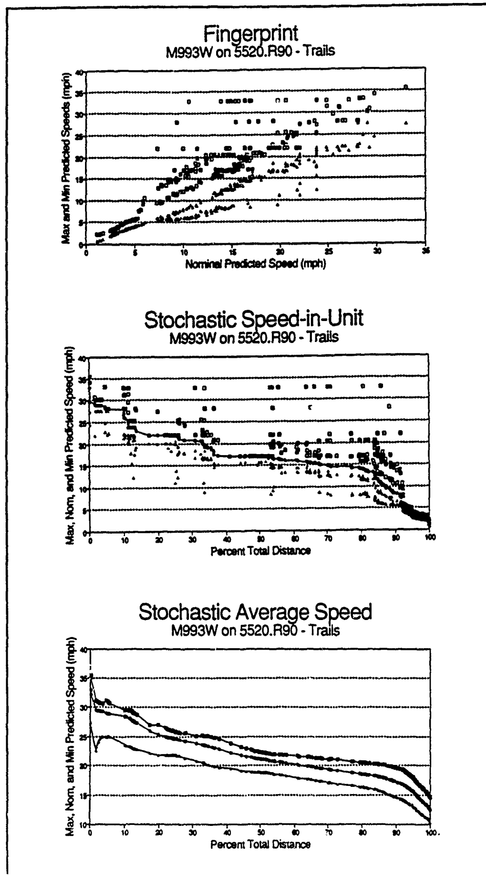
Figure 62. Fingerprint and profiles for M993 on WGe trails
