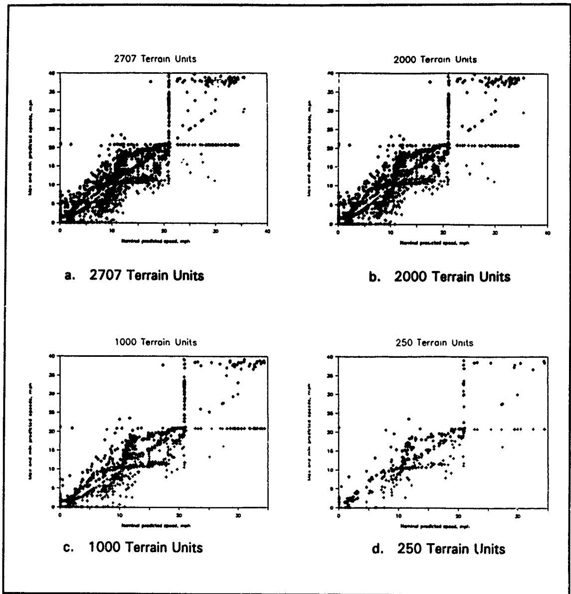
Figure 7. Reduced-dataset fingerprints
