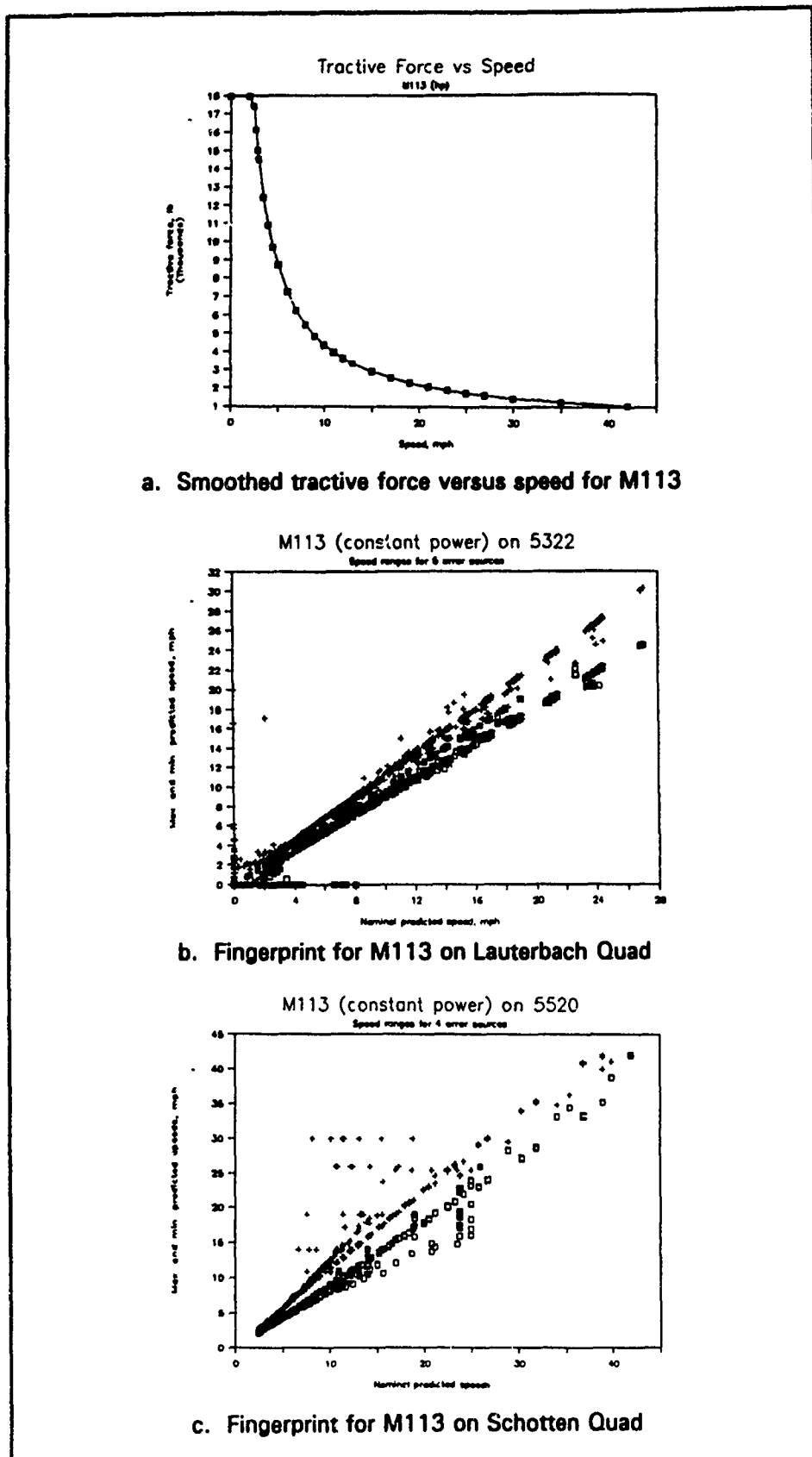
Figure 4. Elimination of most fingerprint anomalies for M113
