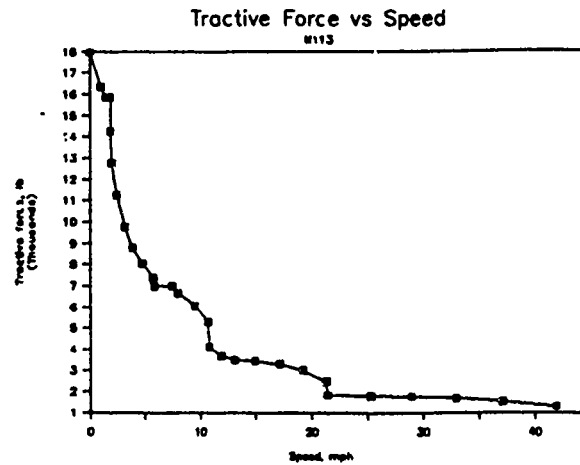
a. Traction force versus speed for M113
