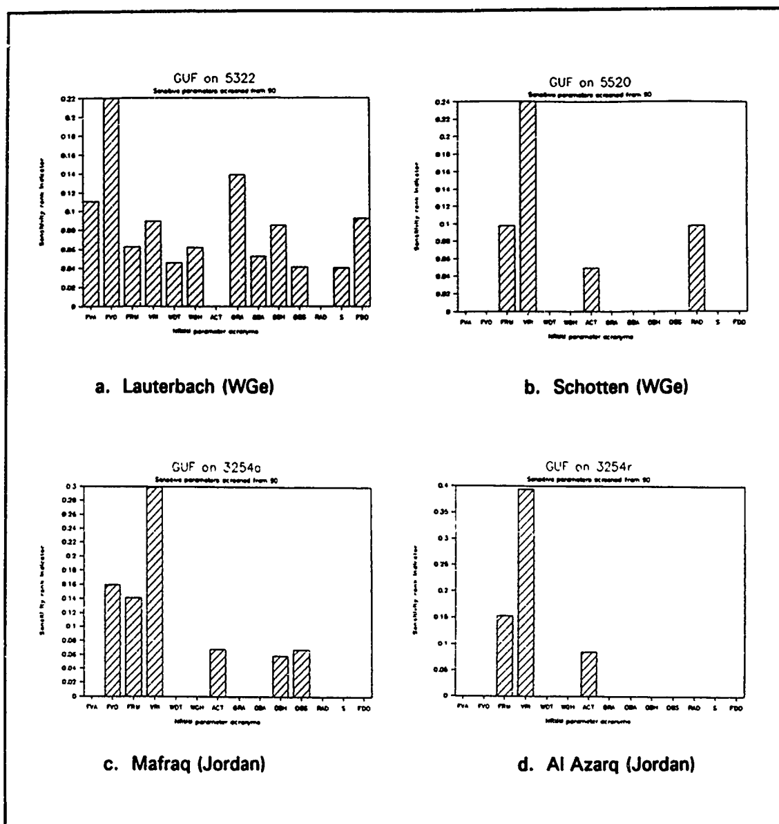
Figure 15. Parameter sensitivity of GUF in four terrains
