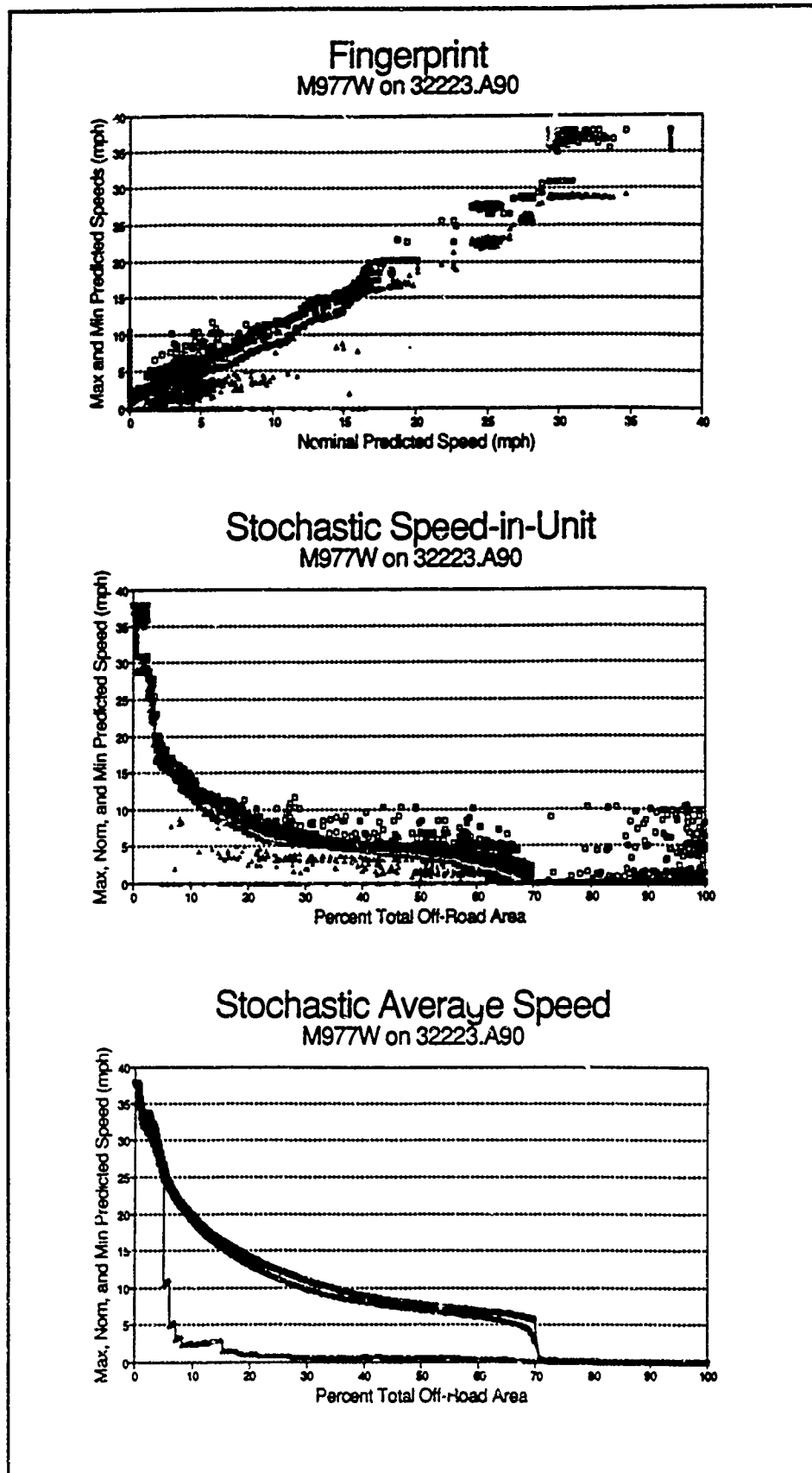
Figure 91. Fingerprint and profiles for M977 on ROK off-road
