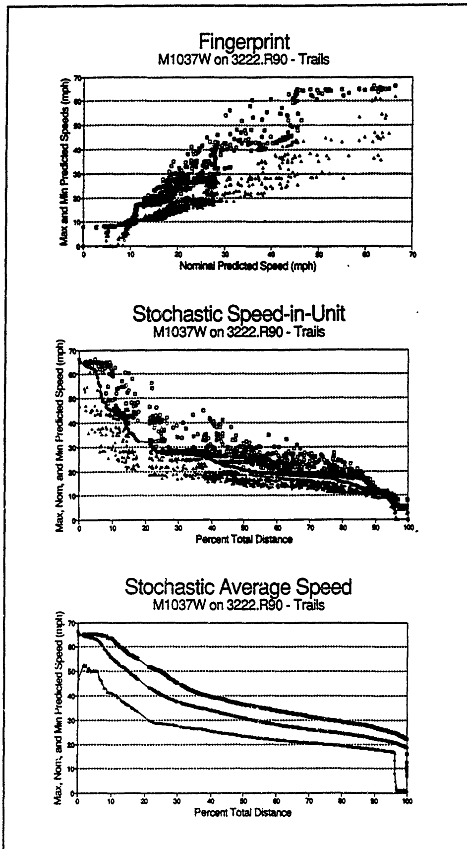
Figure 102. Fingerprint and profiles for M1037 on ROK trails
