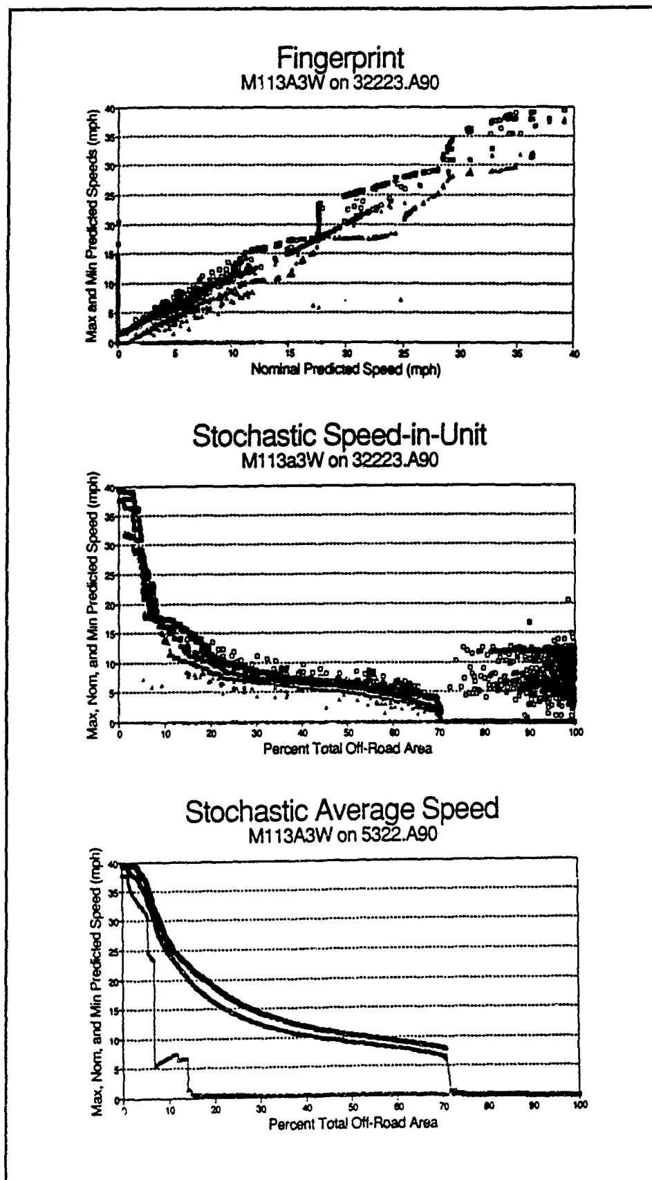
Figure 95. Fingerprint and profiles for M113A3 on ROK off-road
