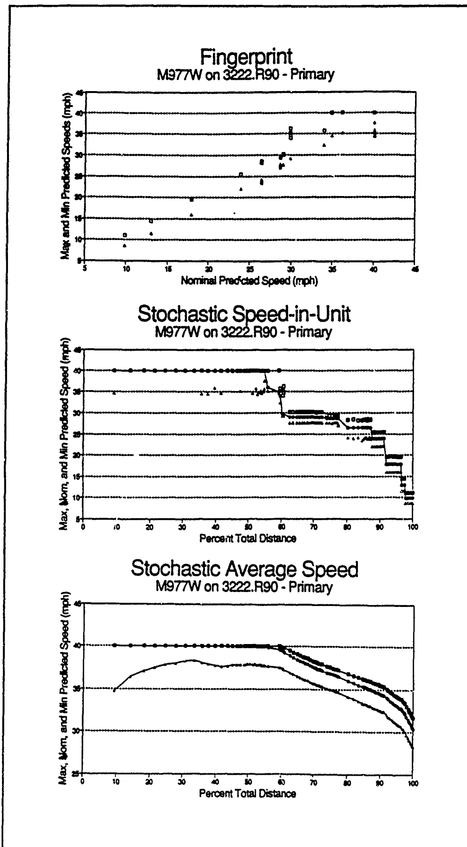
Figure 92. Fingerprint and profiles for M977 on ROK primary roads
