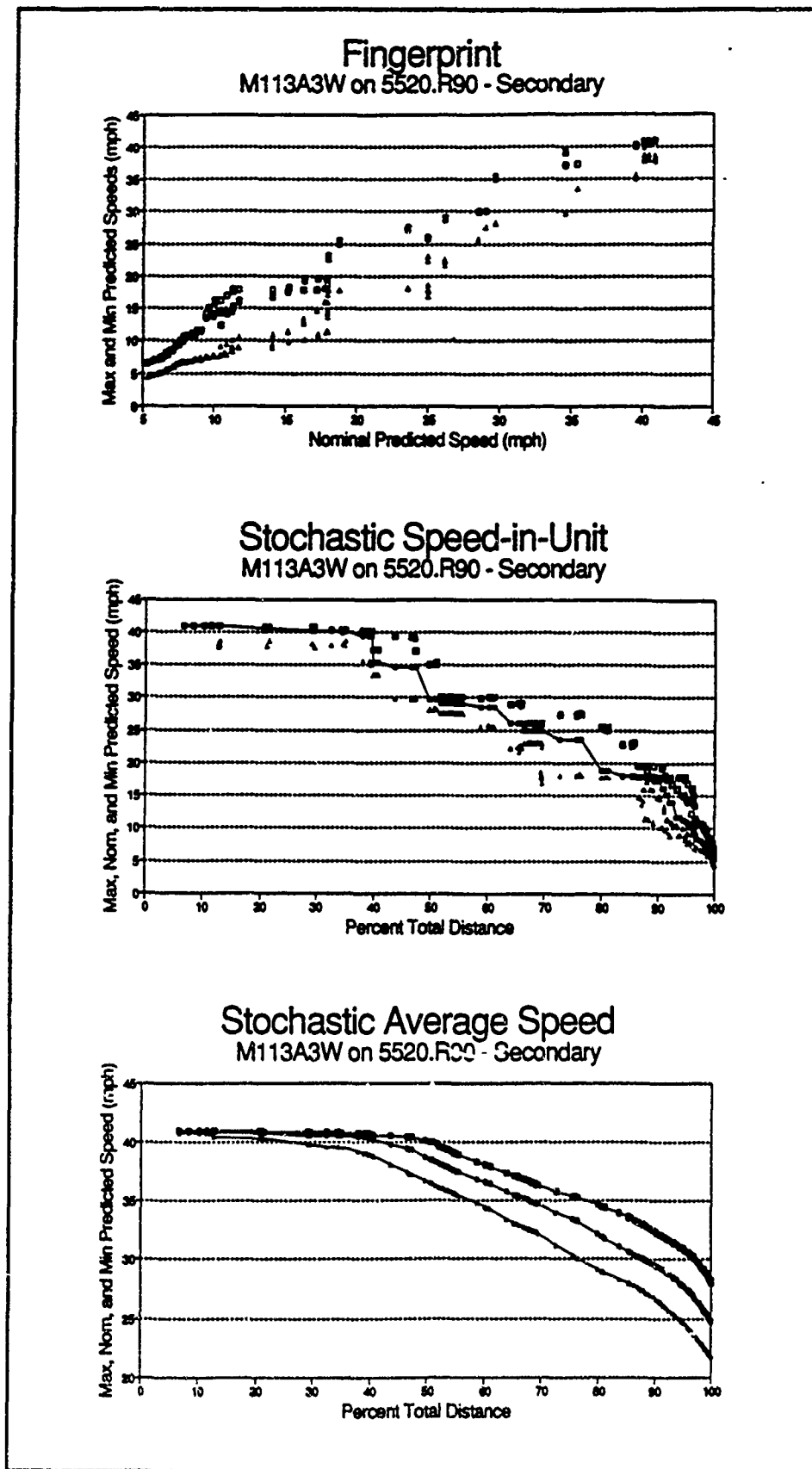
Figure 69. Fingerprint and profiles for M113A3 on WGe secondary roads
