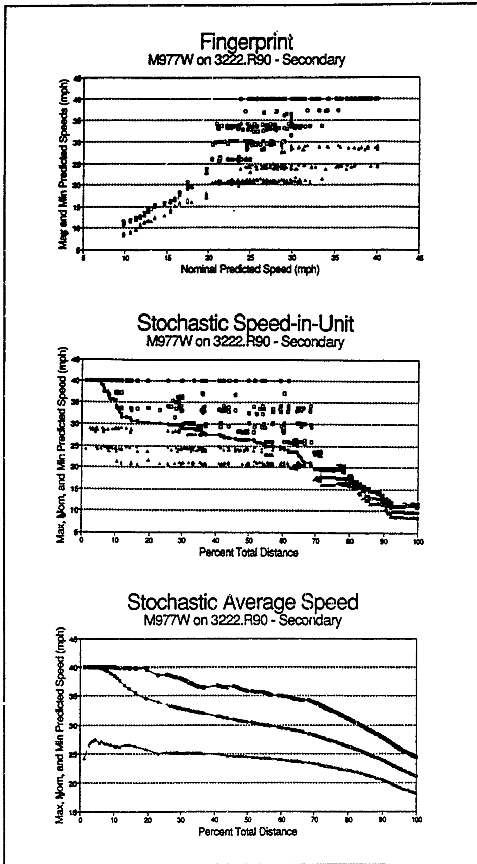
Figure 93. Fingerprint and profiles for M977 on ROK secondary roads
