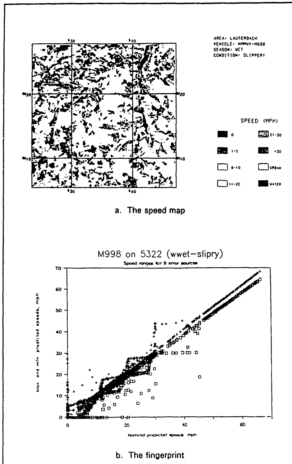
Figure 1. The speed map and the fingerprint
