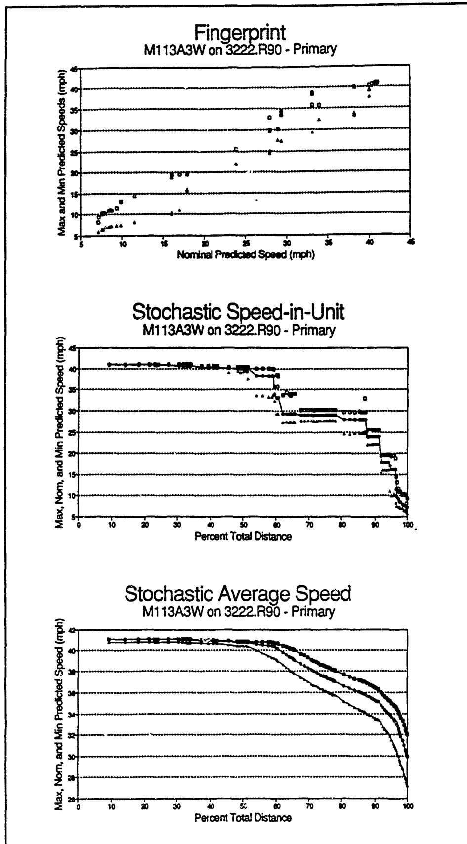
Figure 96. Fingerprint and profiles for M113A3 on ROK primary roads
