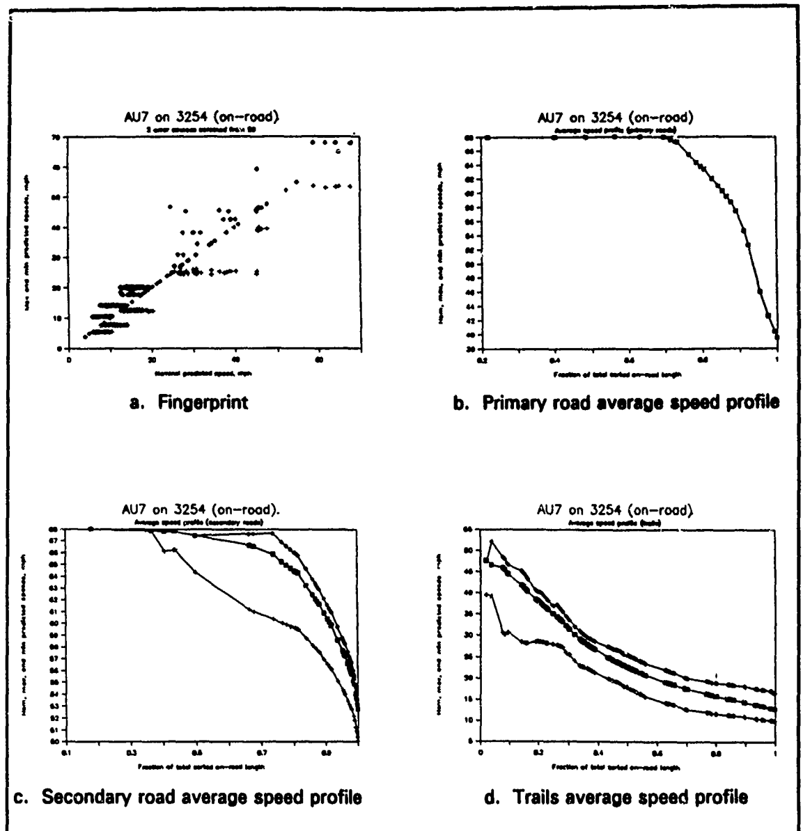
Figure 22. Fingerprint and speed profiles for AU7 on Az Zarqa
