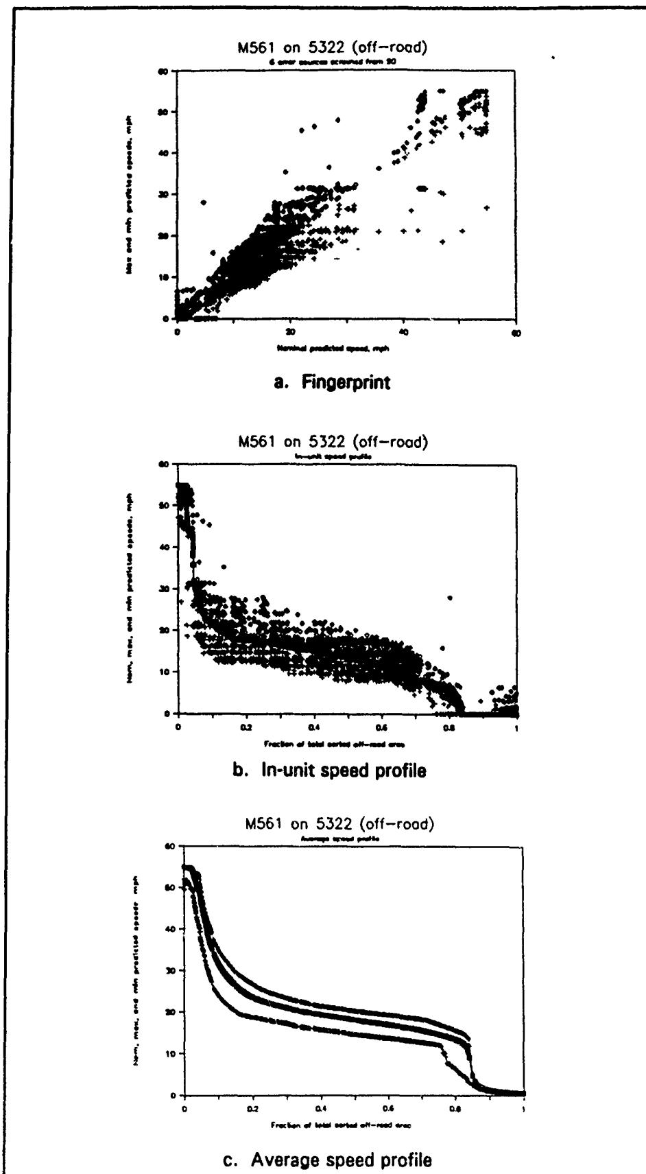
Figure 35. Fingerprints and speed profiles for M561 on Lauerbach
