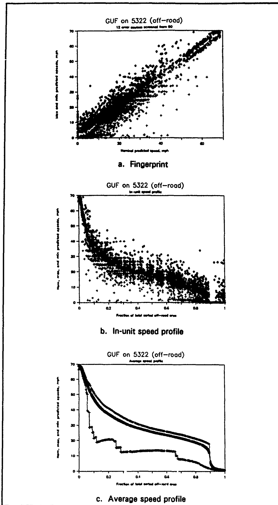
Figure 23. Fingerprints and speed profiles for GUF on Lauterbach
