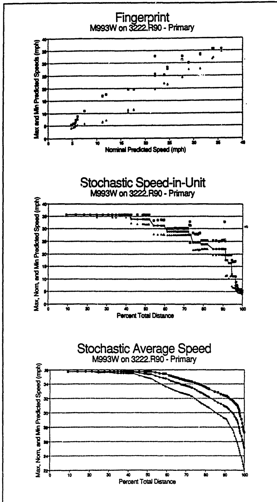
Figure 88. Fingerprint and profiles for M993 on ROK primary roads
