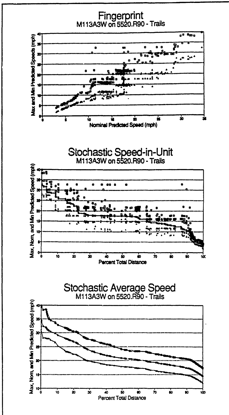
Figure 70. Fingerprint and profiles for M113A3 on WGe trails
