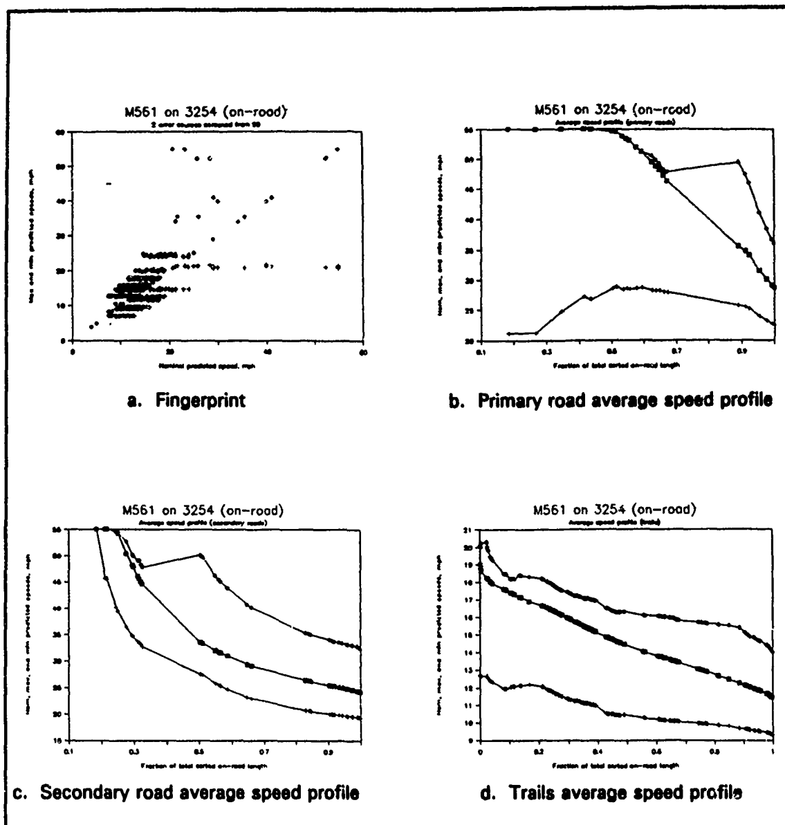
Figure 38. Fingerprint and speed profiles for M561 on Az Zarqa
