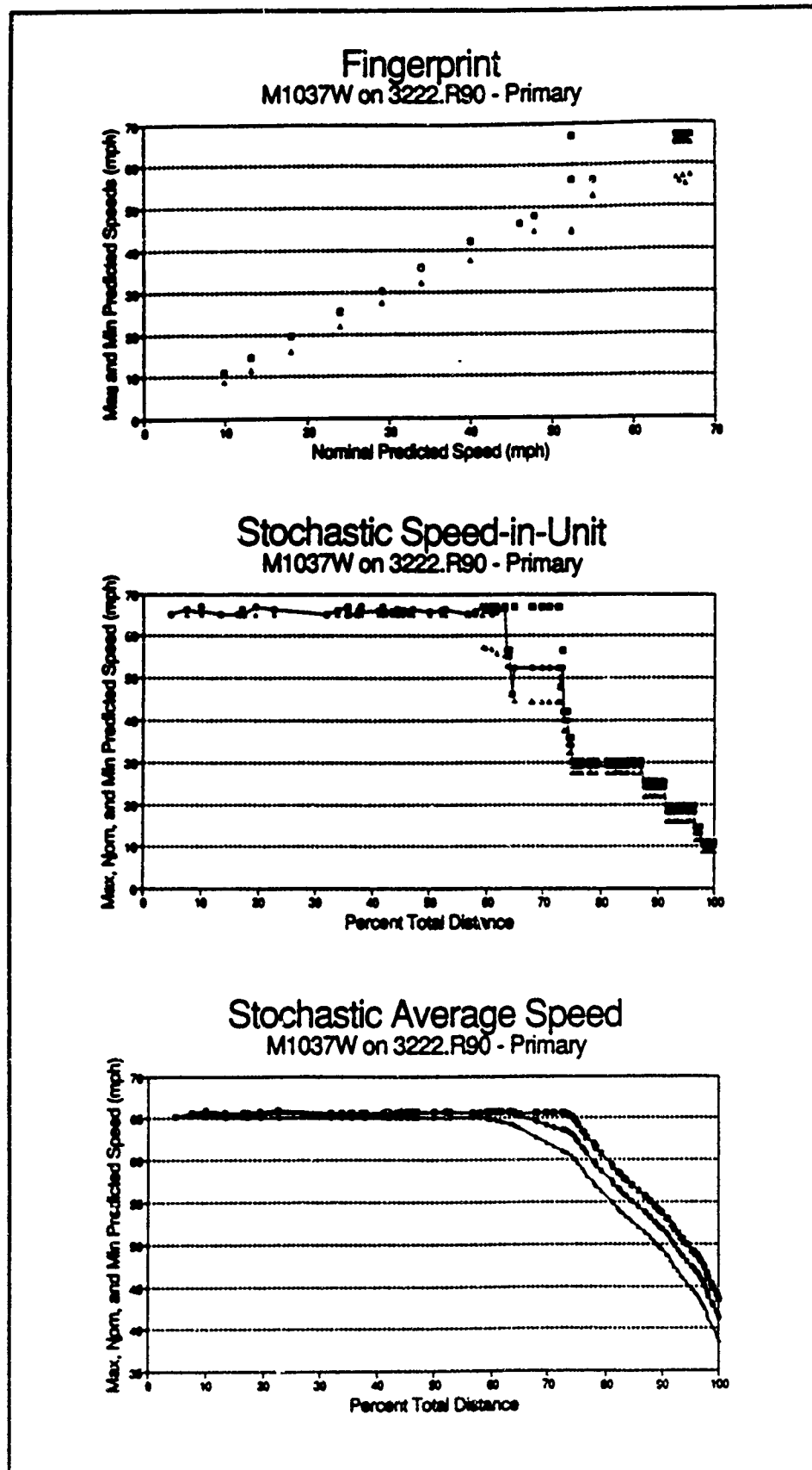
Figure 100. Fingerprint and profiles for M1037 on ROK primary roads
