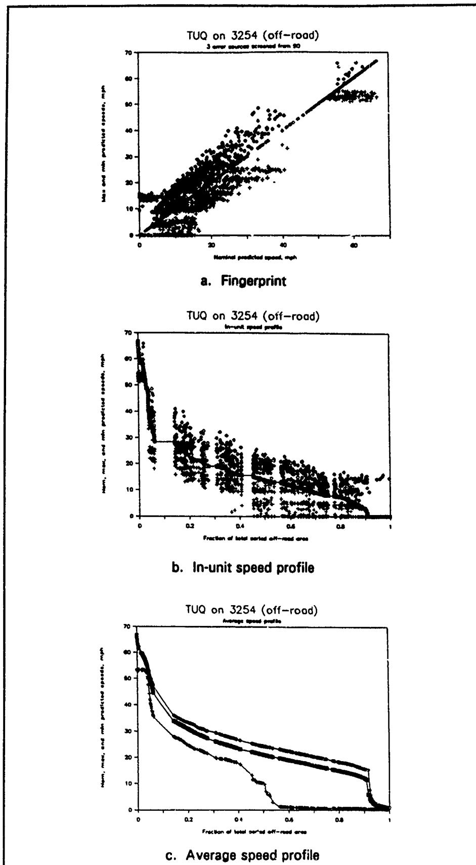
Figure 29. Fingerprints and speed profiles for TUQ on Mafrag
