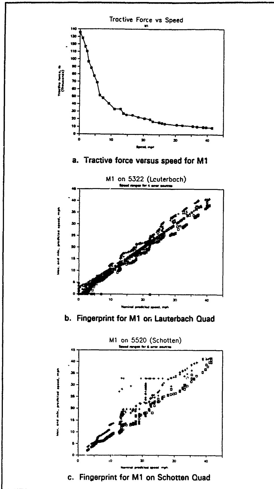
Figure 5. Clustering anomalies in M1 fingerprints
