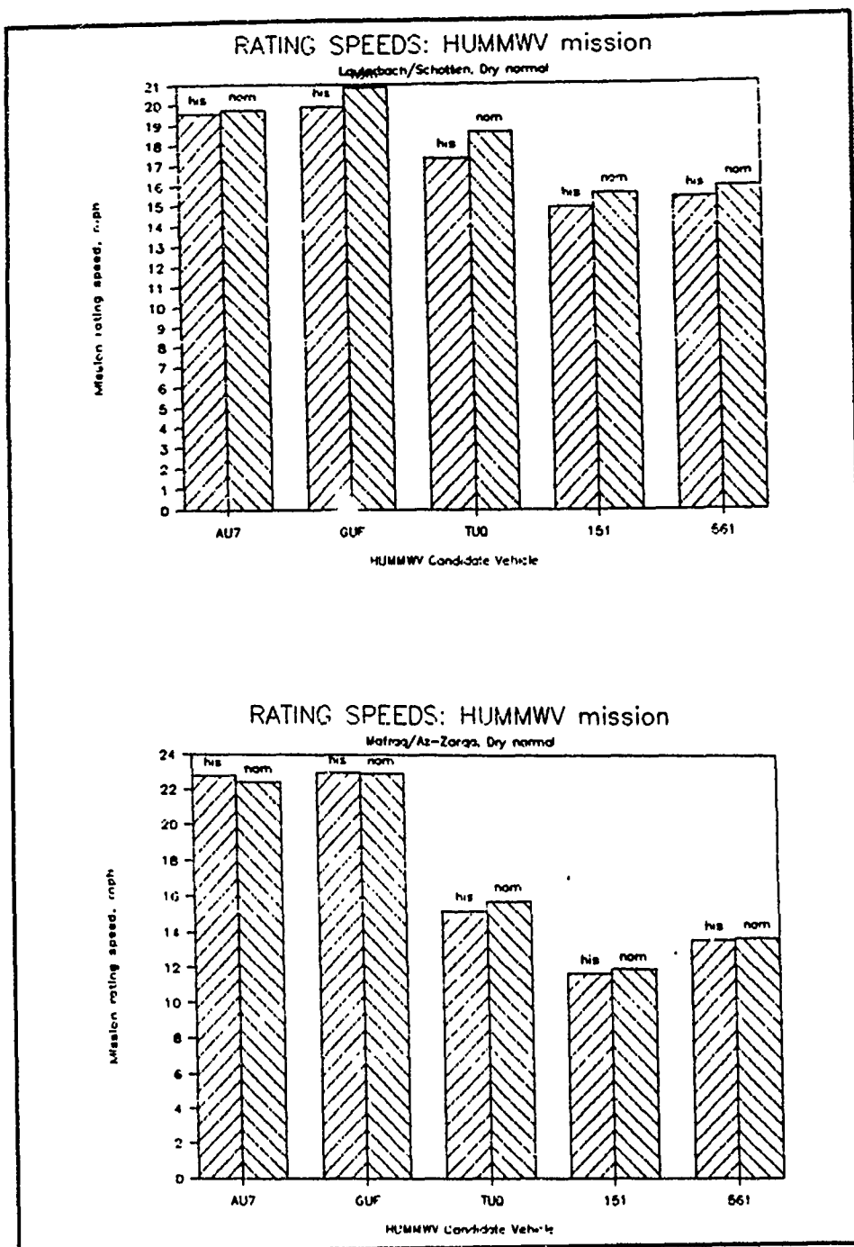
Figure 44. Comparison of historic ("his") and stochastic nominal ("nom") mission rating speeds for the HUMMWV mission
