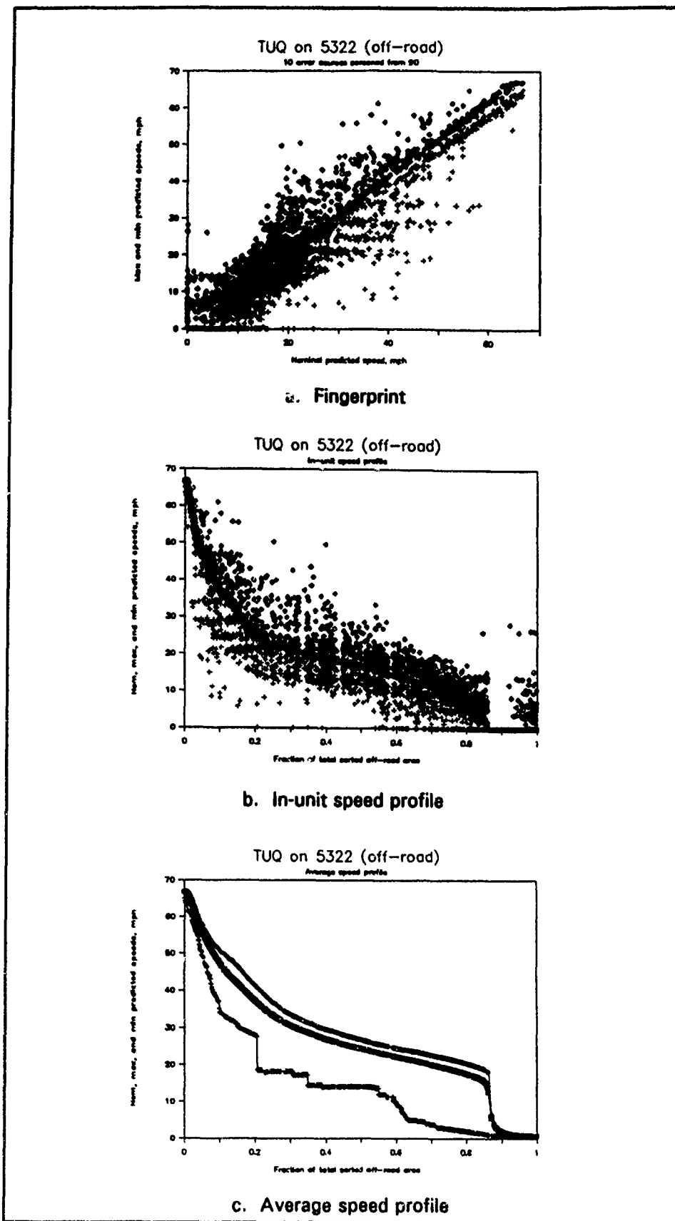
Figure 27. Fingerprints and speed profiles for TUQ on Lauterbach
