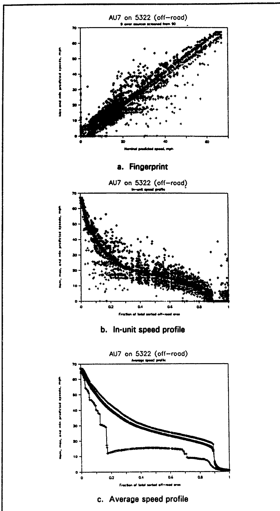
Figure 19. Fingerprints and speed profiles for AU7 on Lauterbach
