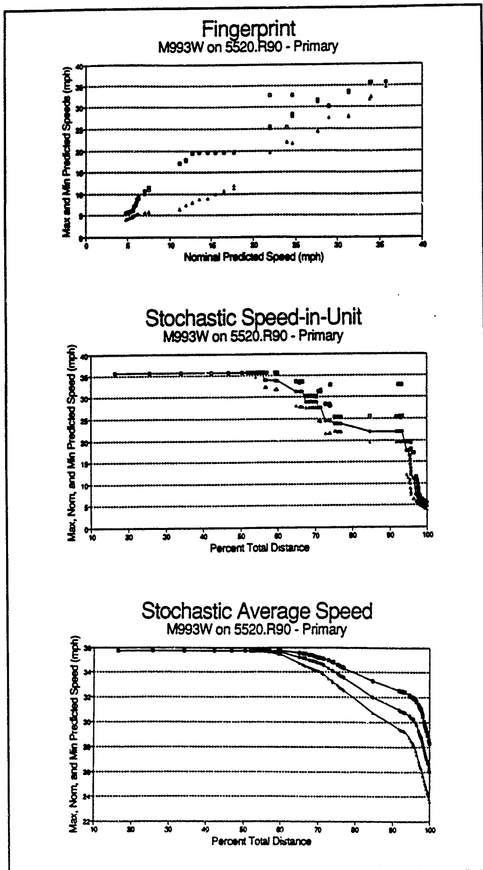
Figure 60. Fingerprint and profiles for M993 on WGe primary roads
