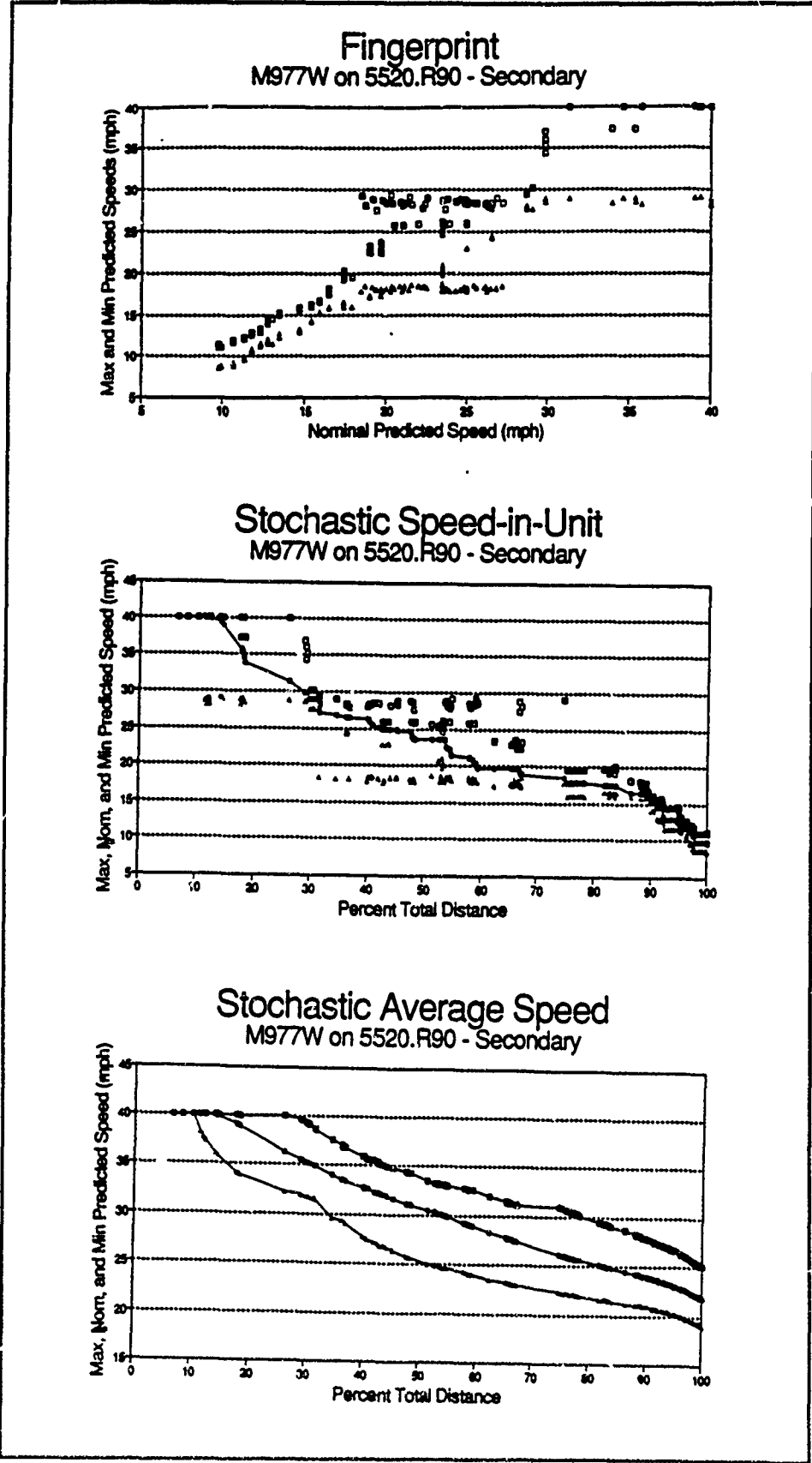
Figure 65. Fingerprint and profiles for M977 on WGe secondary road
