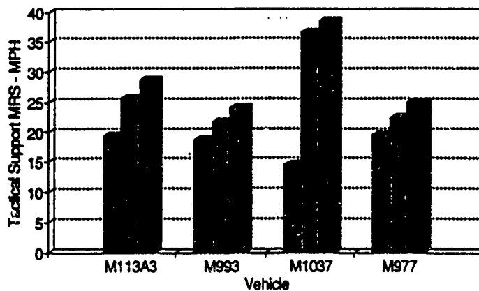
Figure 103. Mission rating speeds for WGe
