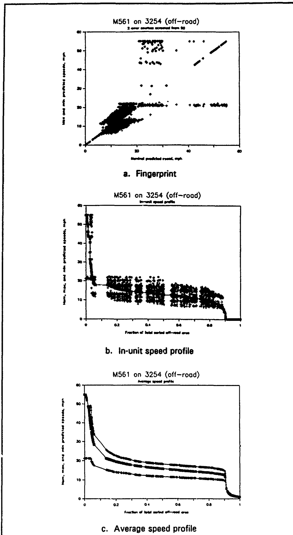
Figure 37. Fingerprints and speed profiles for M561 on Mafrq
