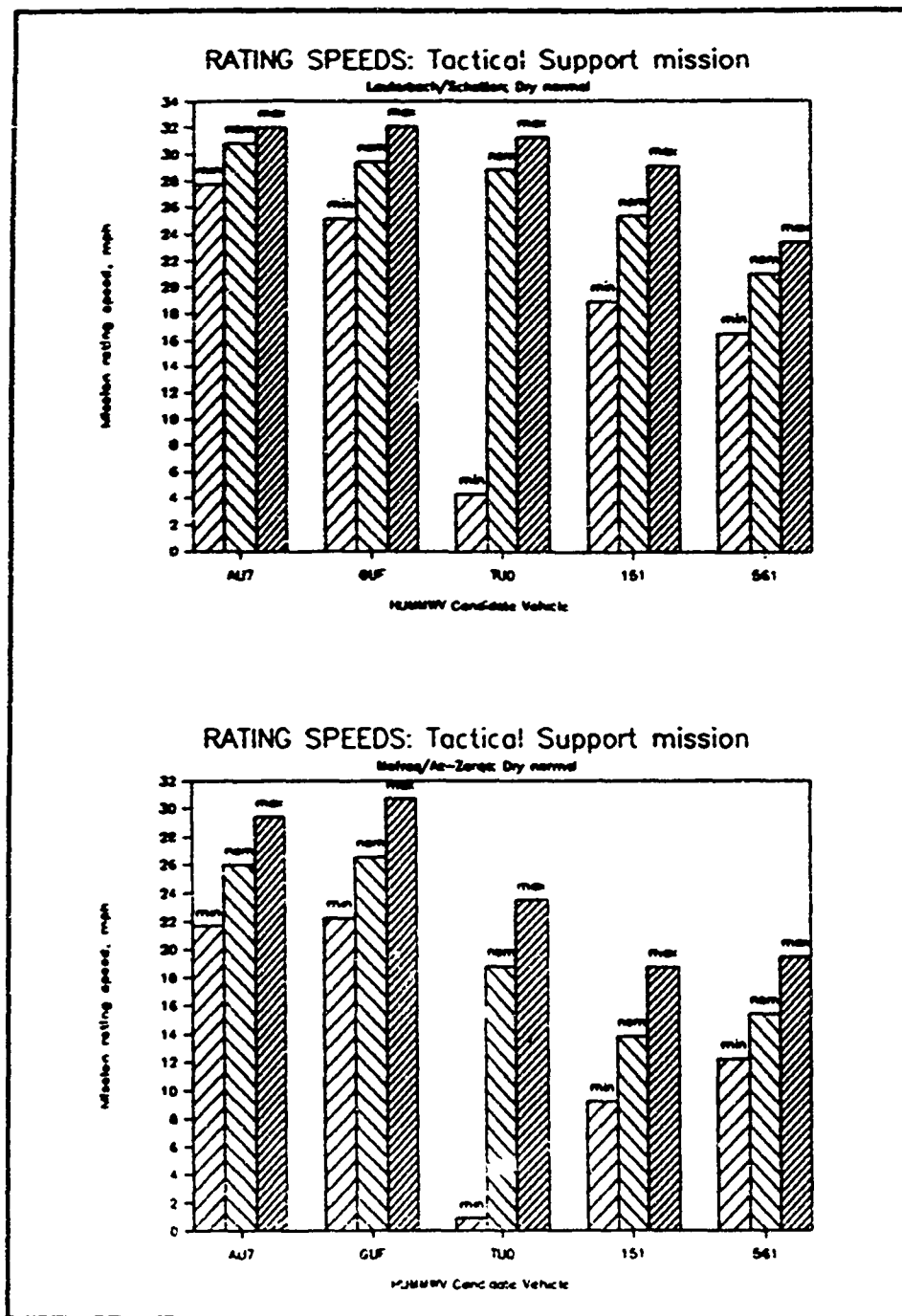
Figure 41. Mission rating speeds for the Tactical Support mission
