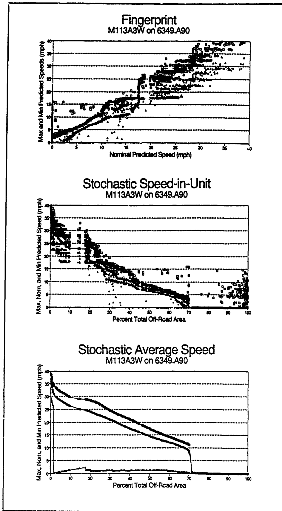
Figure 81. Fingerprint and profiles for M113A3 on SWA off-road
