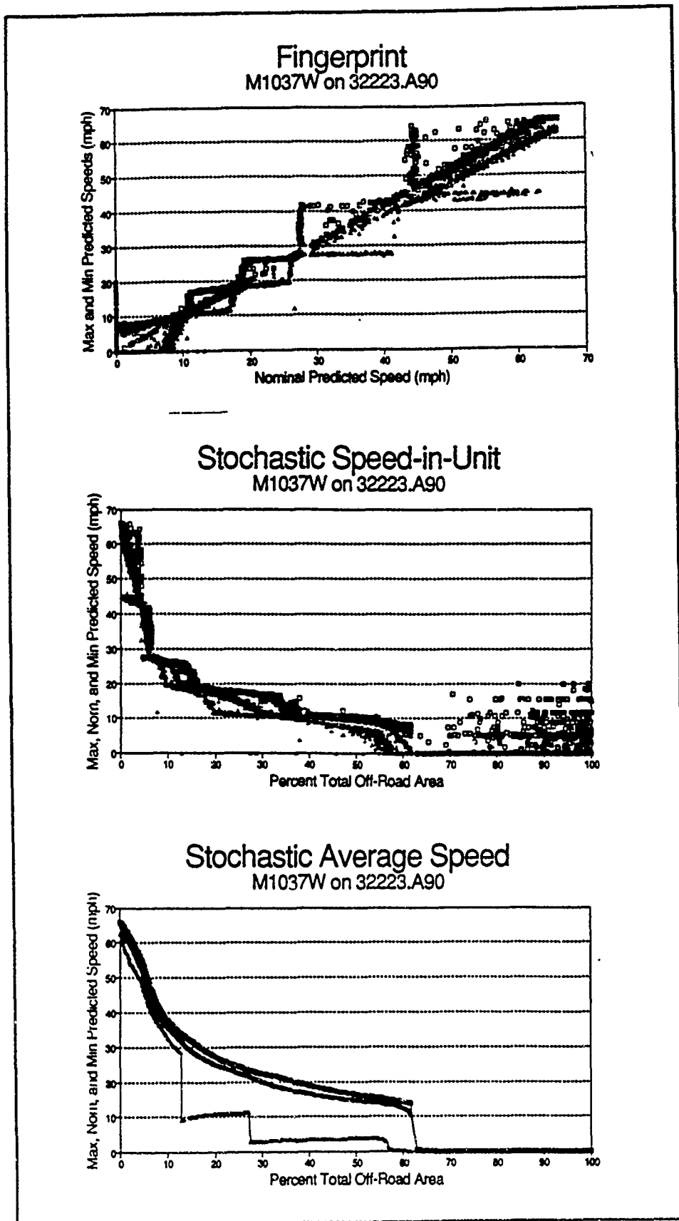
Figure 99. Fingerprint and profiles for M1037 on ROK off-road
