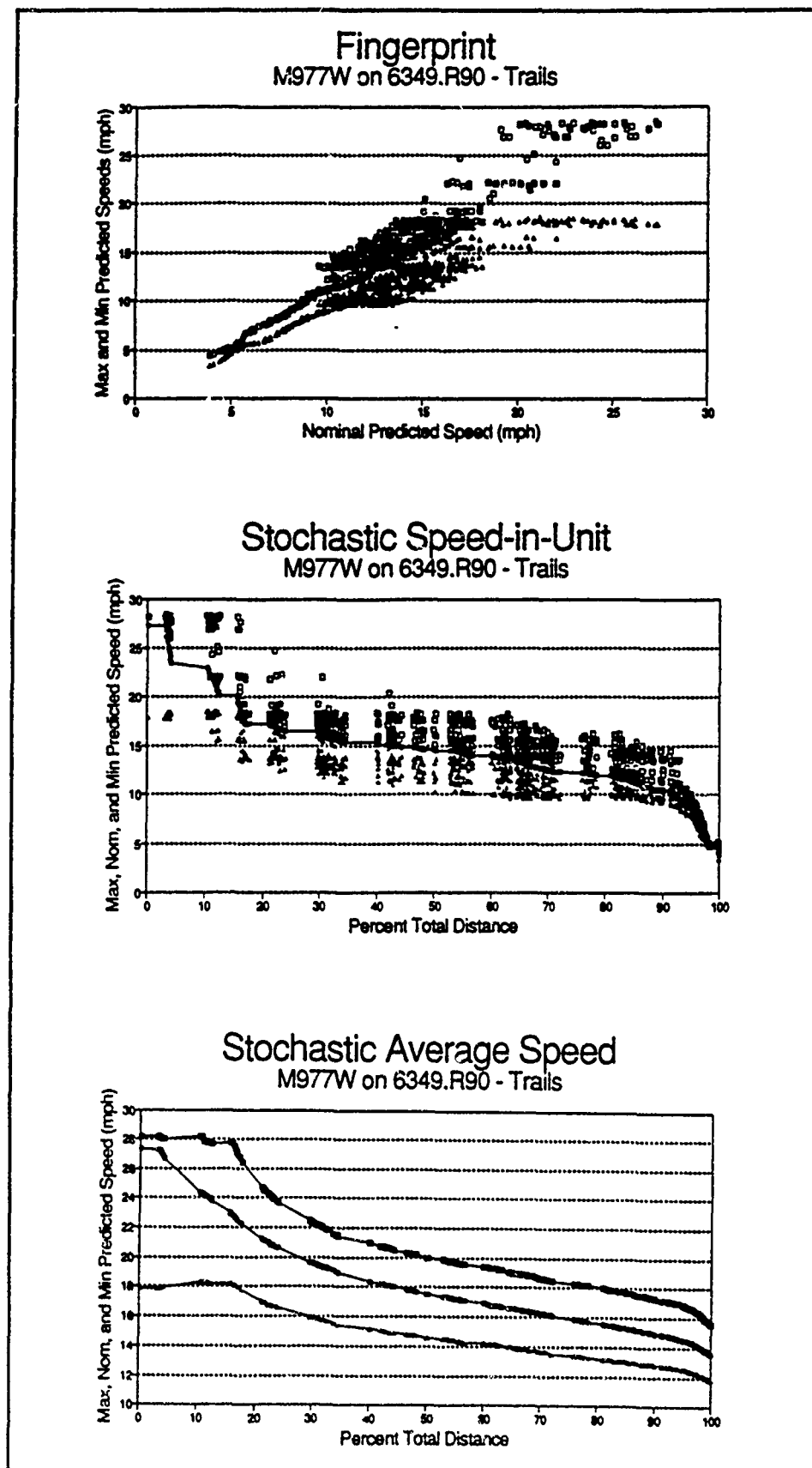
Figure 80. Fingerprint and profiles for M977 on SWA trails
