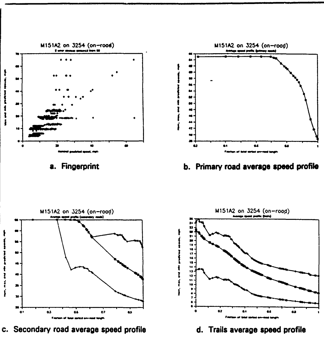
Figure 34. Fingerprint and speed profiles for M151 on Az Zarqa
