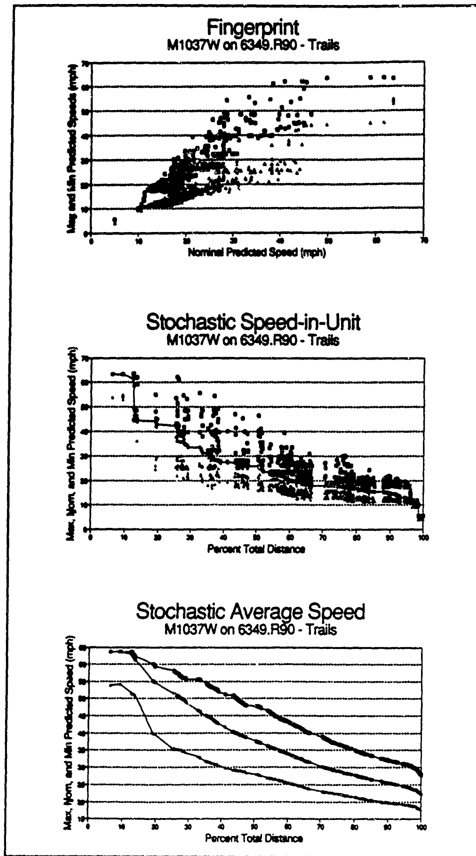
Figure 86. Fingerprint and profiles for M1037 on SWA trails
