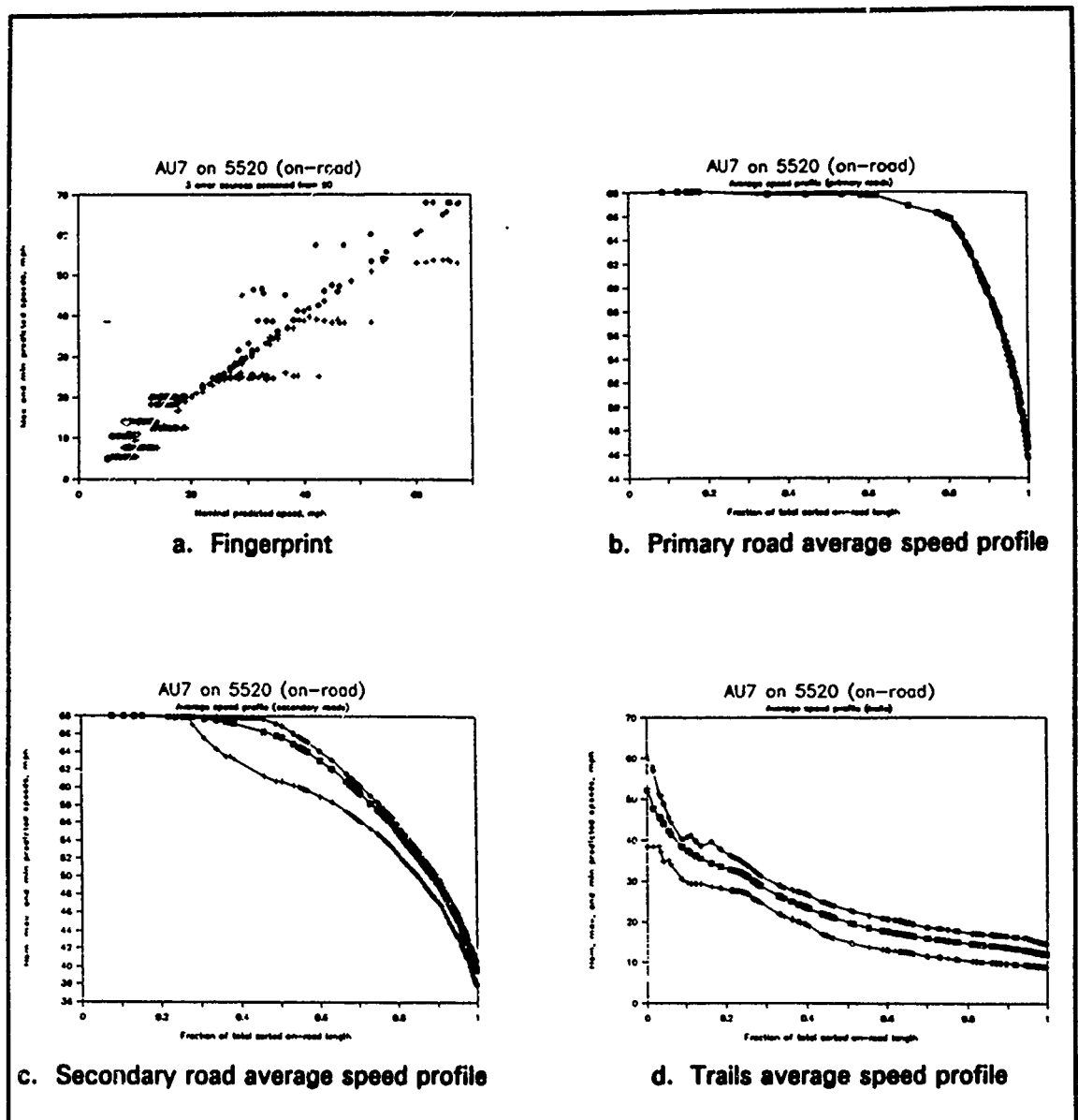
Figure 20. Fingerprint and speed profiles for AU7 on Schotten
