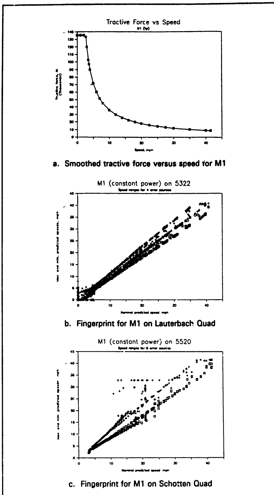
Figure 6. Elimination of most fingerprint anomalies for M1
