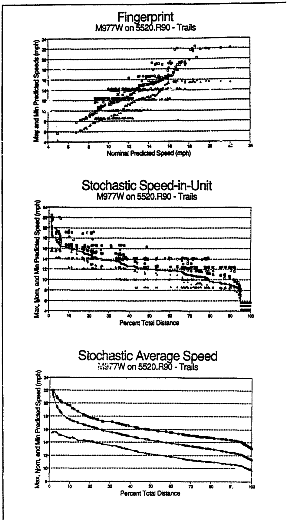
Figure 66. Fingerprint and profiles for M977 on WGe trails
