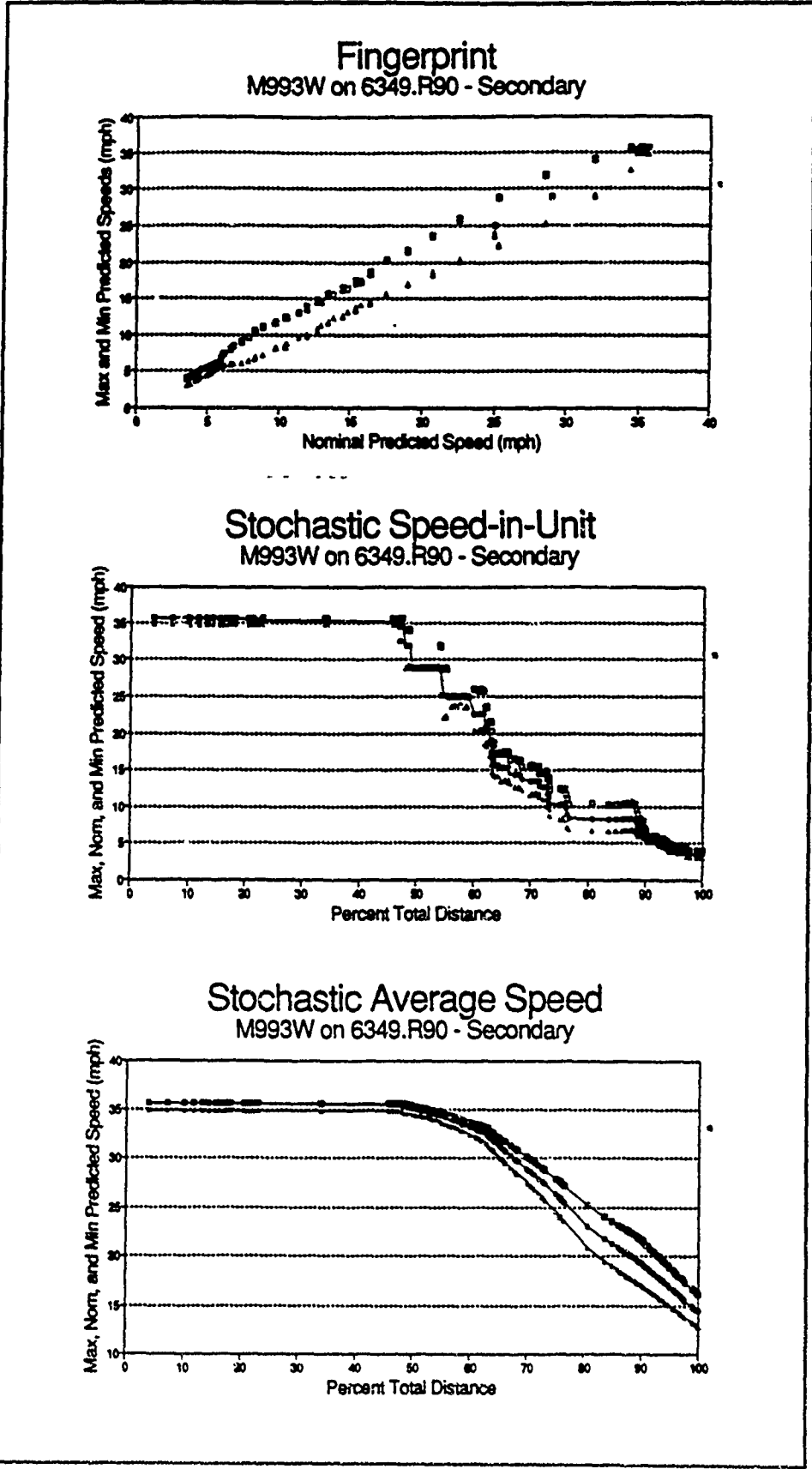
Figure 76. Fingerprint and profiles for M993 on SWA secondary roads
