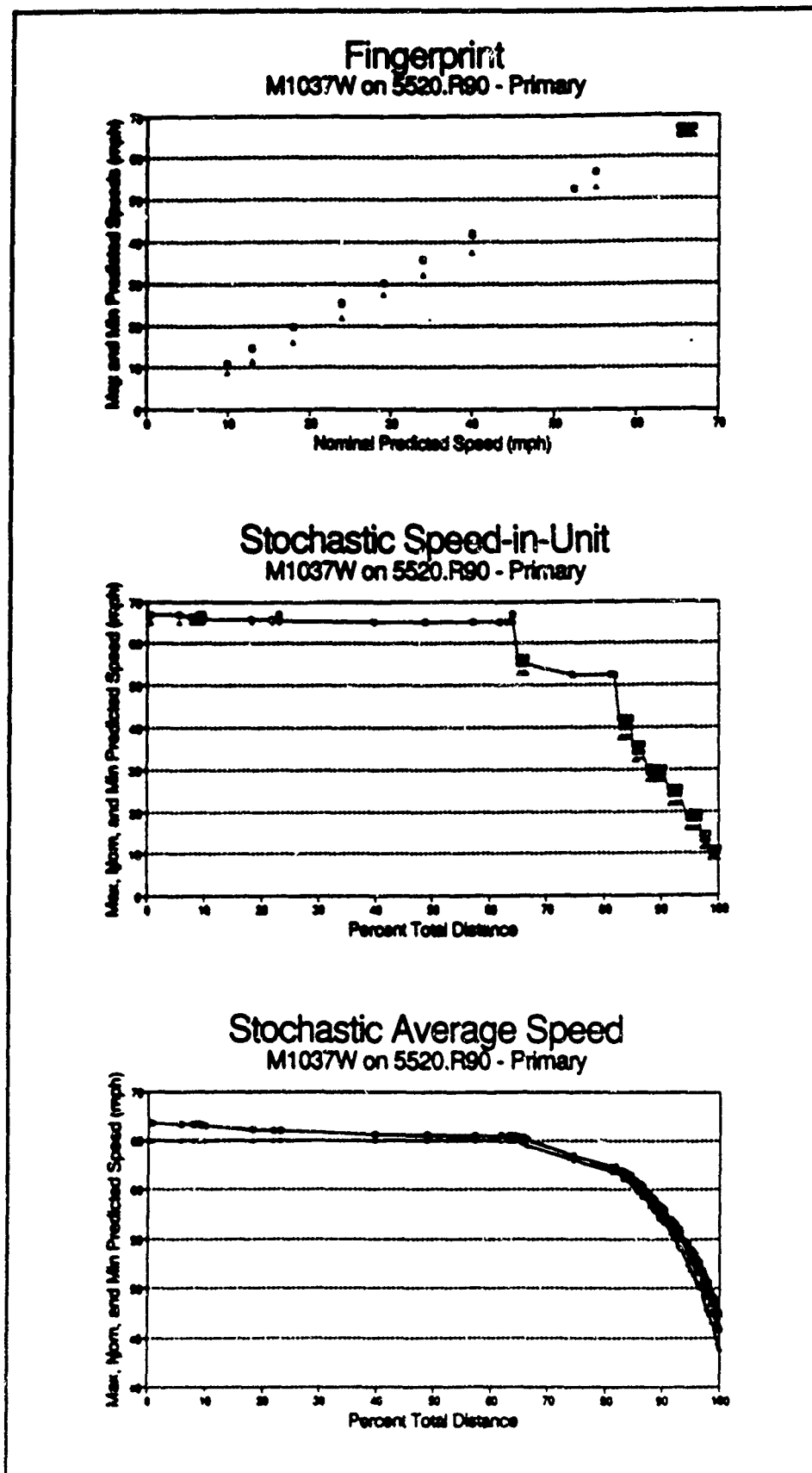
Figure 72. Fingerprint and profiles for M1037 on WGe primary roads
