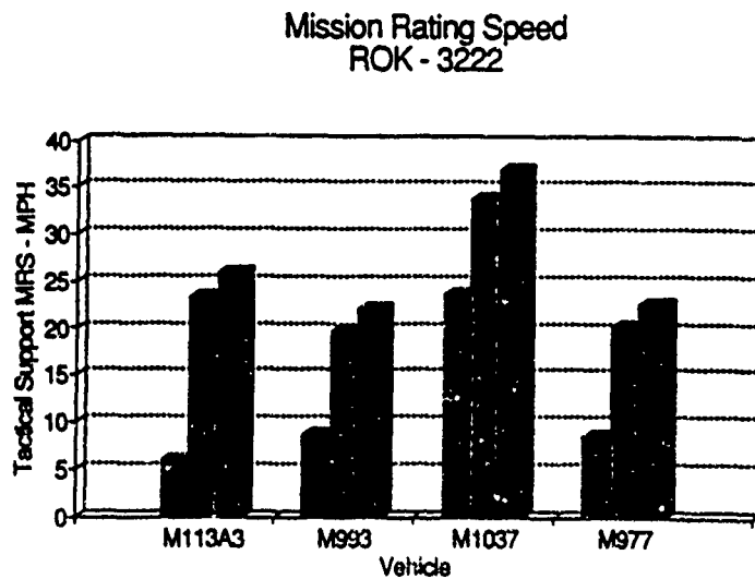
Figure 105. Mission rating speeds for ROK
