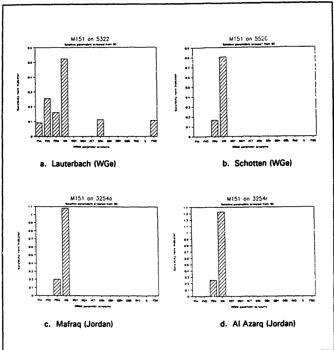
Figure 17. Parameter sensitivity of M151 in four terrains
