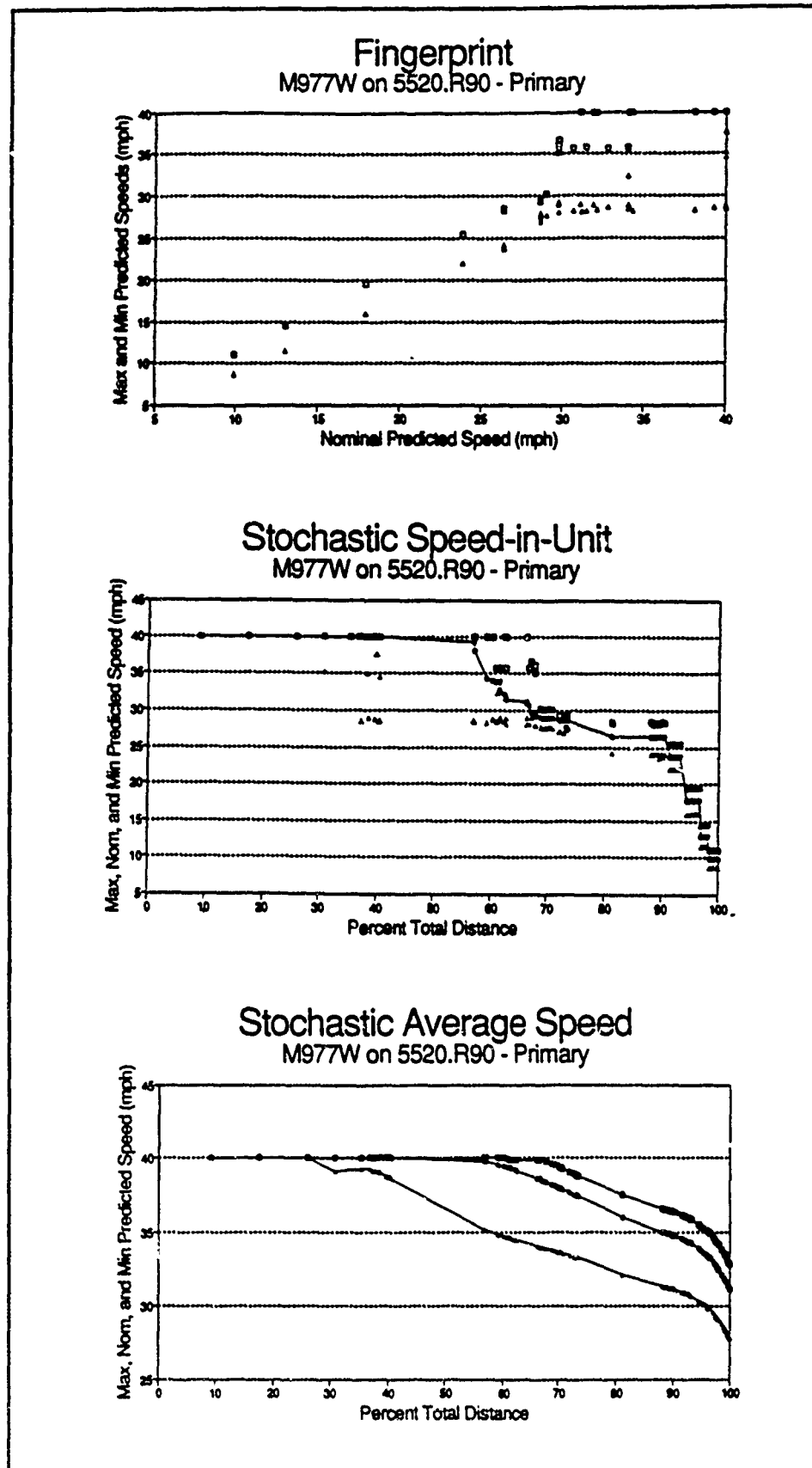
Figure 64. Fingerprint and profiles for M977 on WGe primary roads
