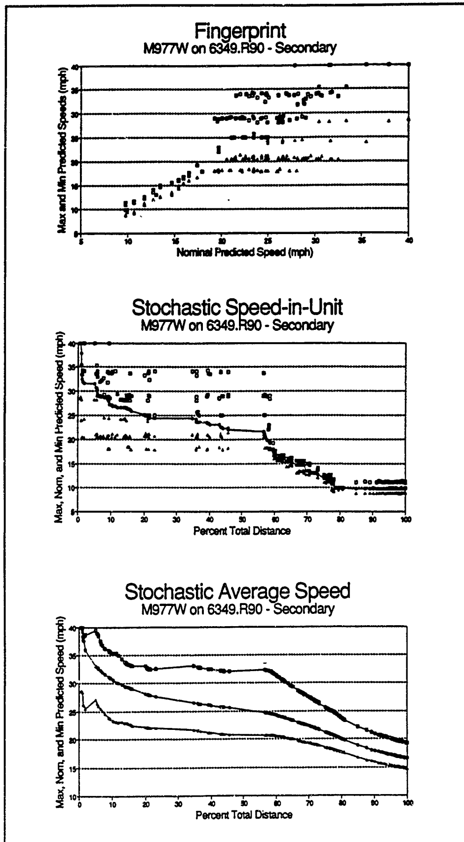
Figure 79. Fingerprint and profiles for M977 on SWA secondary roads
