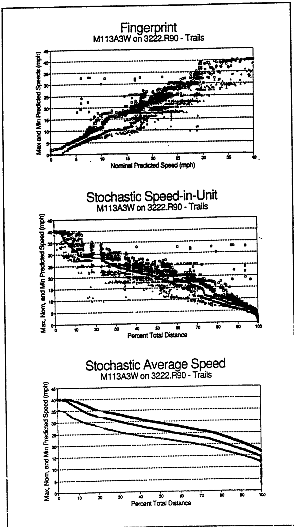
Figure 98. Fingerprint and profiles for M113A3 on ROK trails
