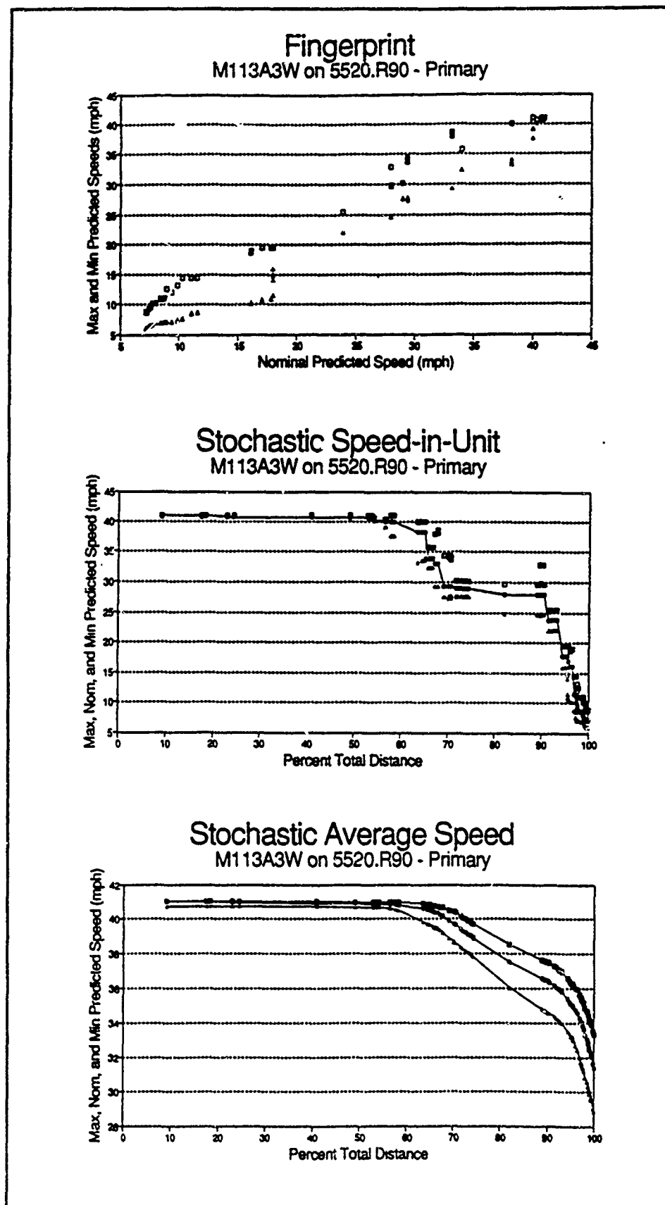
Figure 68. Fingerprint and profiles for M113A3 on WGe primary roads
