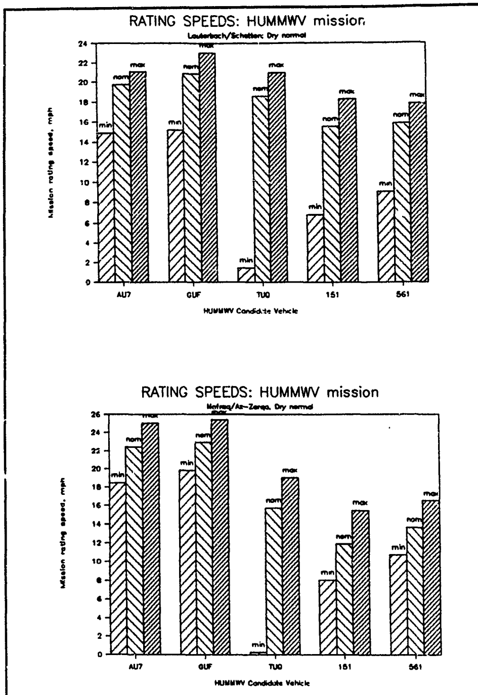
Figure 43. Mission rating speeds for the HUMMWV mission
