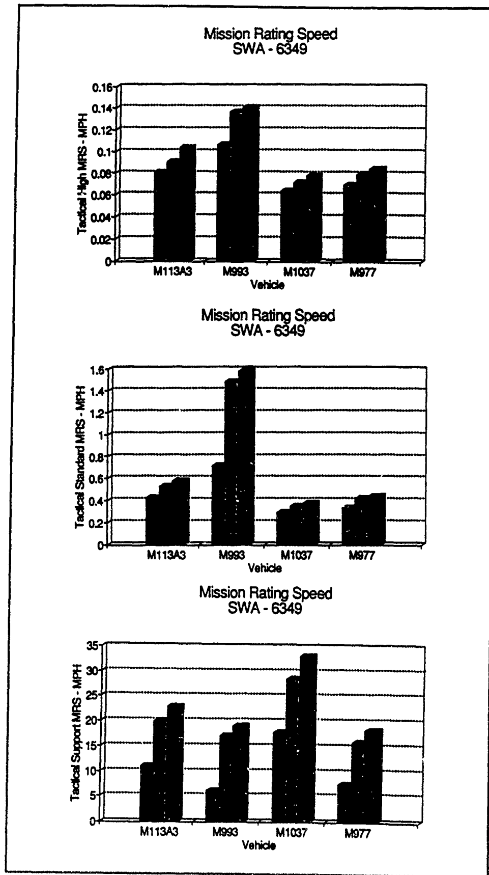
Figure 104. Mission rating speeds for SWA
