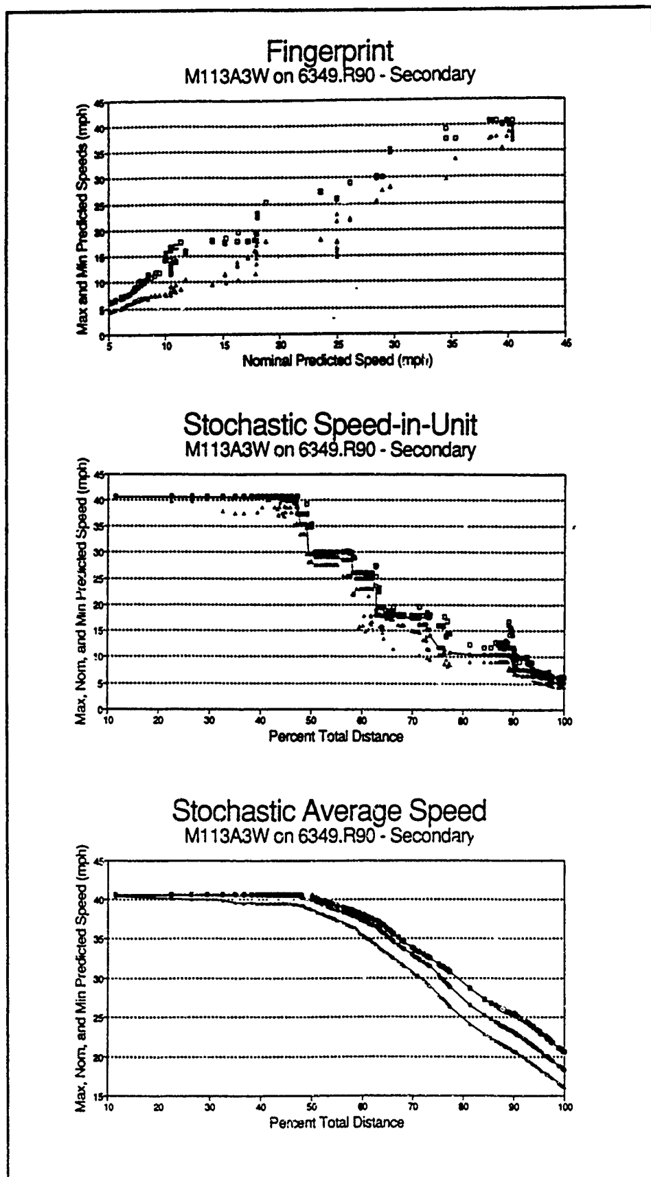
Figure 82. Fingerprint and profiles for M113A3 on SWA secondary roads
