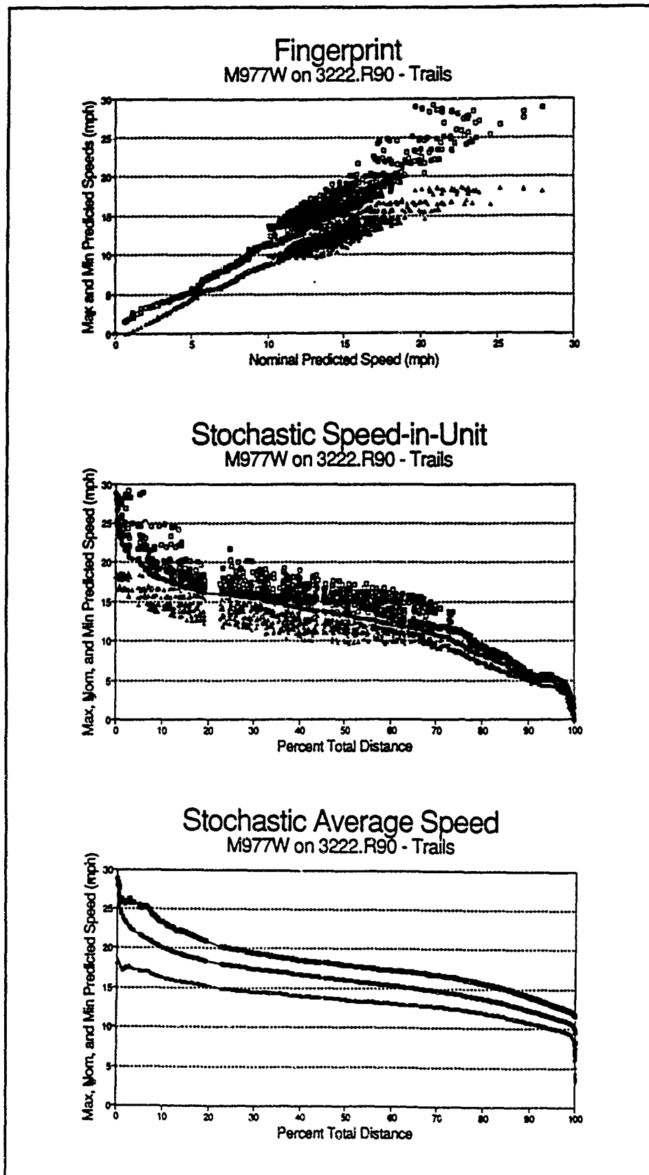
Figure 94. Fingerprint and profiles for M977 on ROK trails
