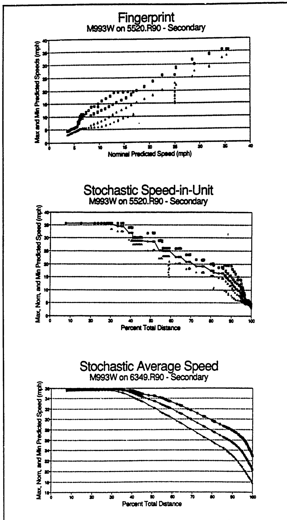
Figure 61. Fingerprint and profiles for M993 on WGe secondary roads
