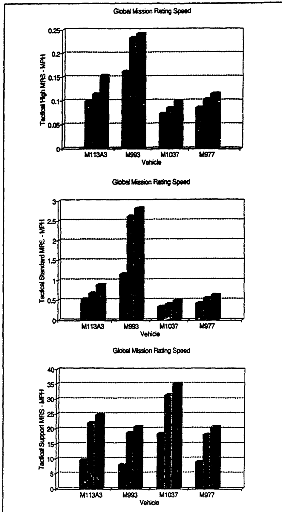
Figure 106. Global mission rating speeds
