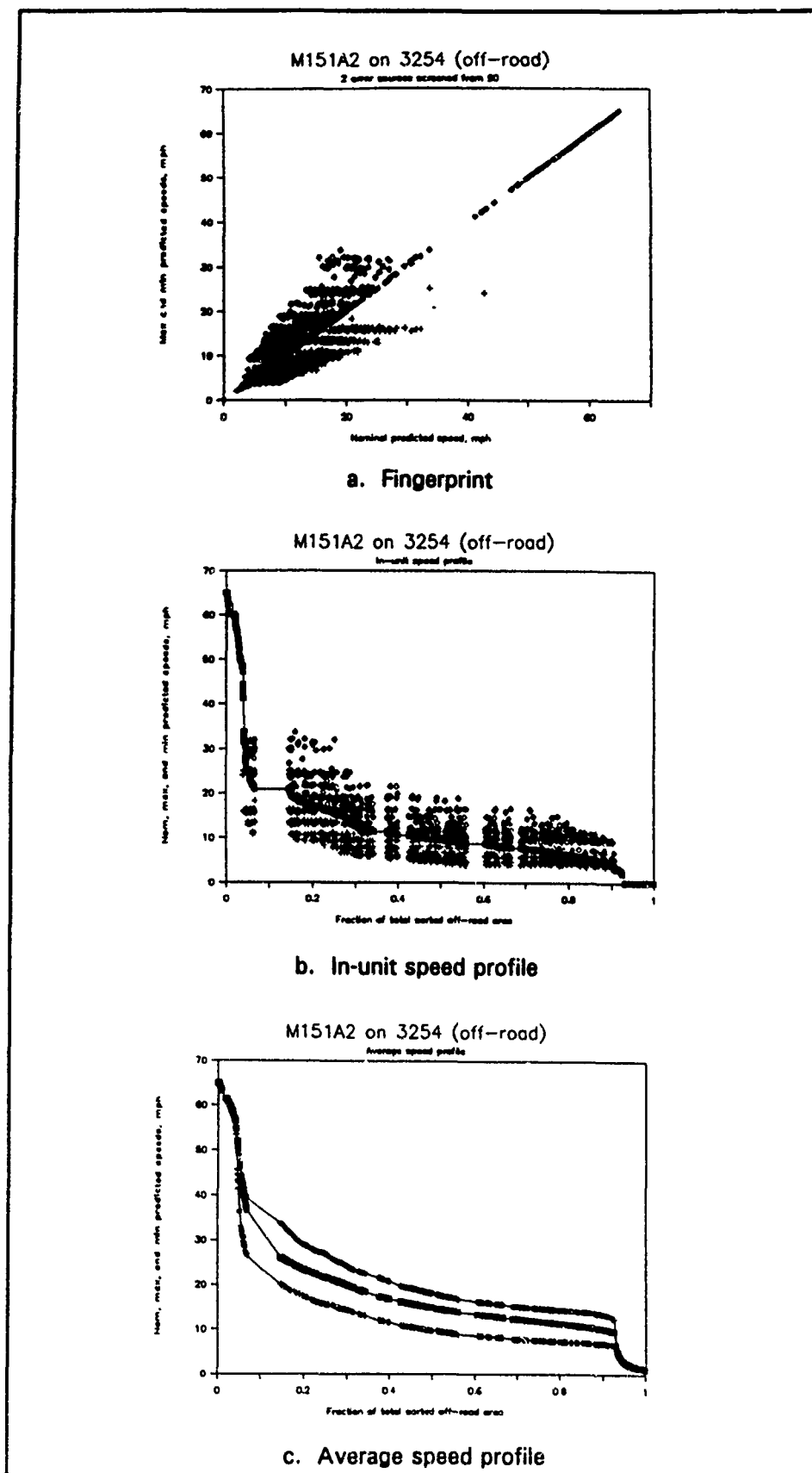
Figure 33. Fingerprints and speed profiles for M151 on Mafrag
