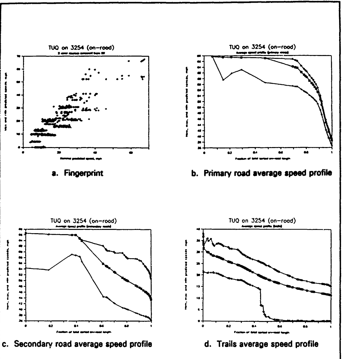
Figure 30. Fingerprint and speed profiles for TUQ on Az Zarqa
