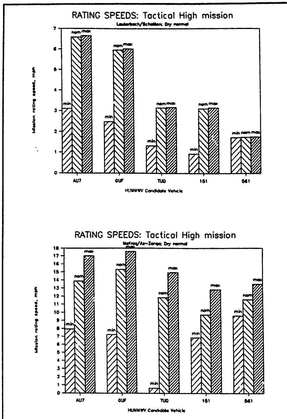
Figure 39. Mission rating speeds for the Tactical High mobility mission
