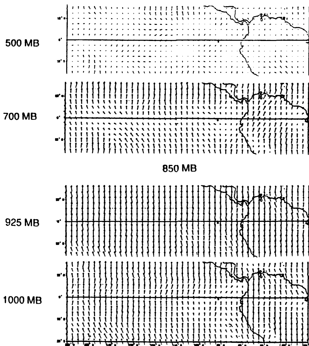
Figure 18b: Interlevel v850 comparison graph for 1990
