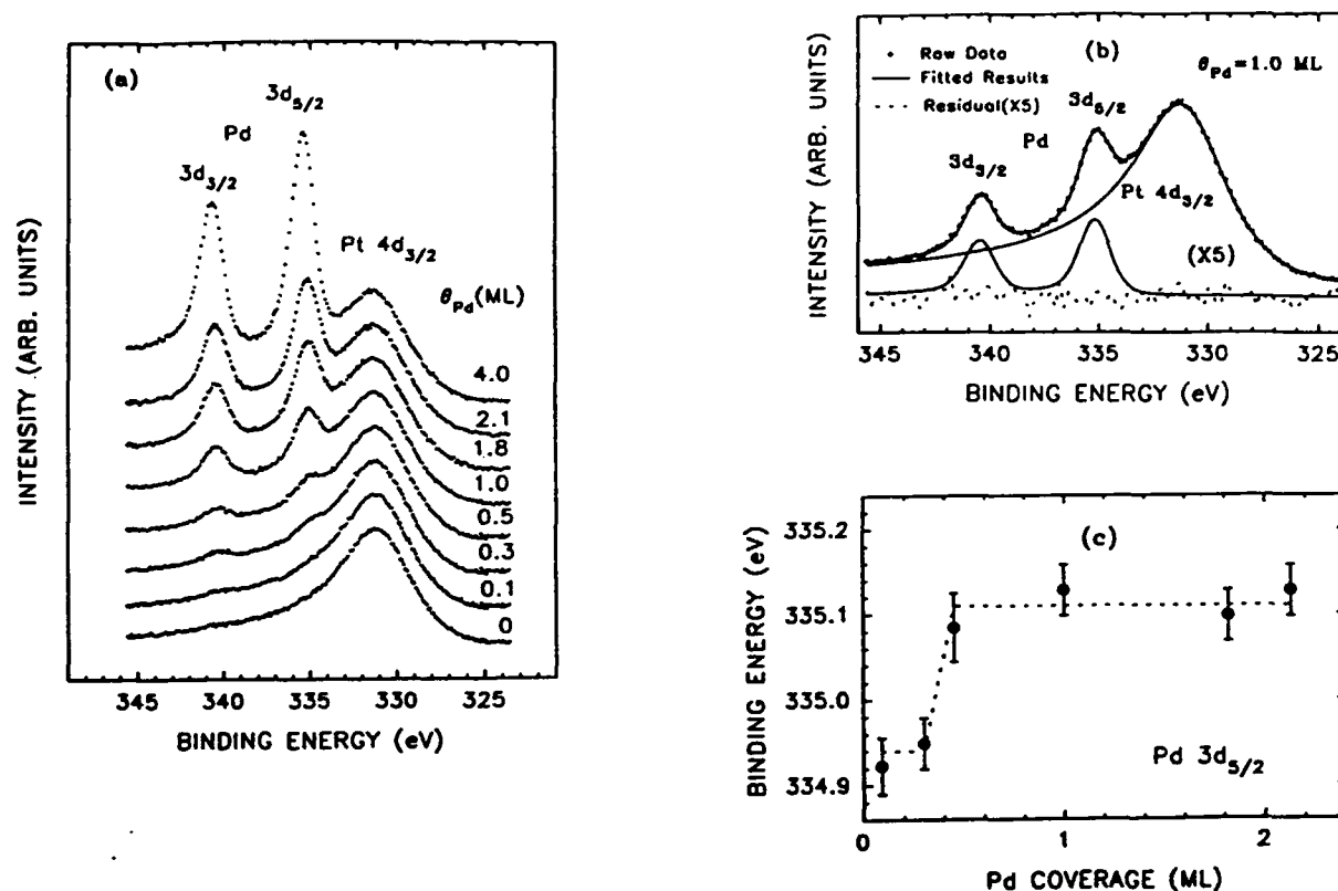
Figure 22. XPS results of Pd adlayers deposited in UHV on Pt(111): (a) Pd 3d and Pt 4d 3/2 core-level spectra, (b) the same as in (a) but at \theta_{Pd} = 1.0 ML and the fitted results. (c) - binding-energy shift of Pd the 3d 5/2 core-level as the Pd coverage varies.
