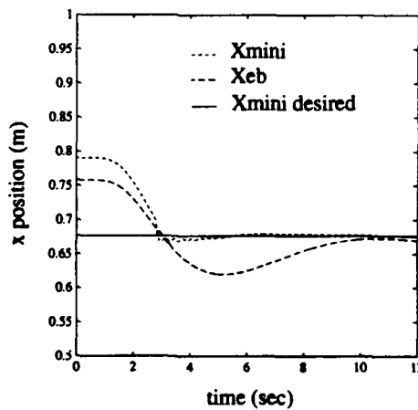
Figure 5: Coordinated Repositioning: x motion.
