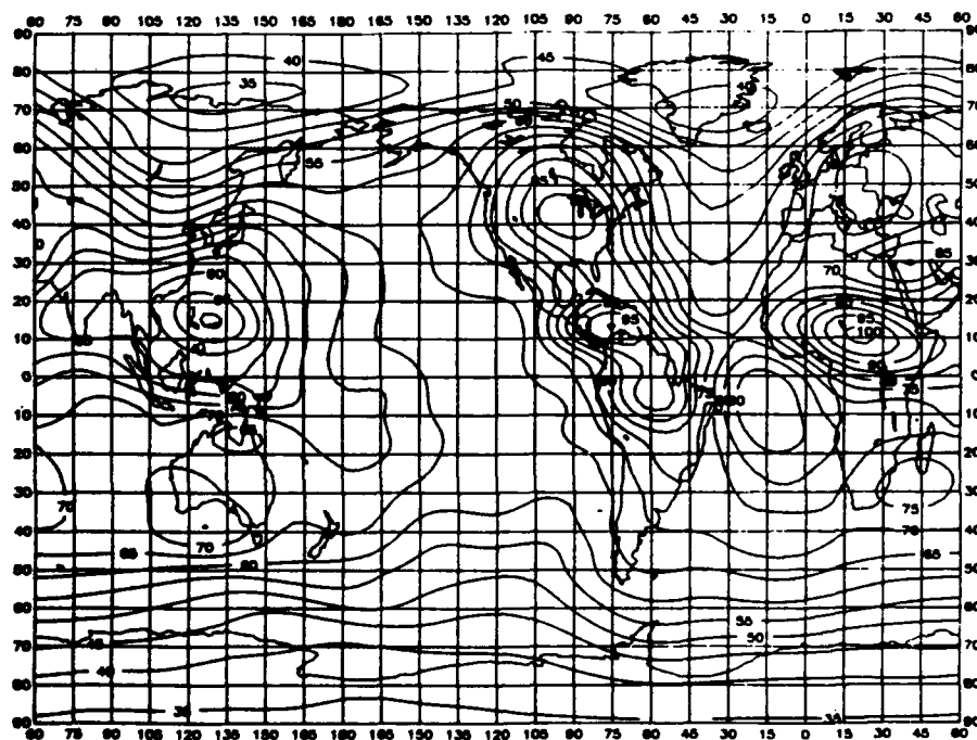
Figure 48. Expected values of atmospheric radio noise at 1 MHz, F_{am} (dB above kT_{0b} ), for June, July, August, 2000–2400 hours (Spaulding and Washburn, 1985).
