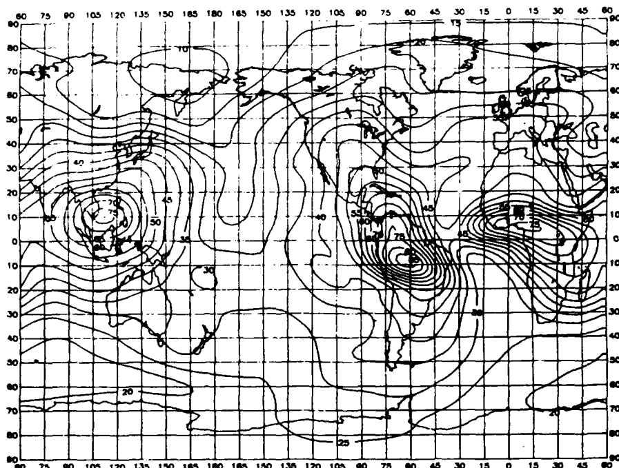
Figure 51. Expected values of atmospheric radio noise at 1 MHz, F_{am} (dB above kT_0b ), for September, October, November, 0800-1200 hours (Spaulding and Washburn, 1985).
