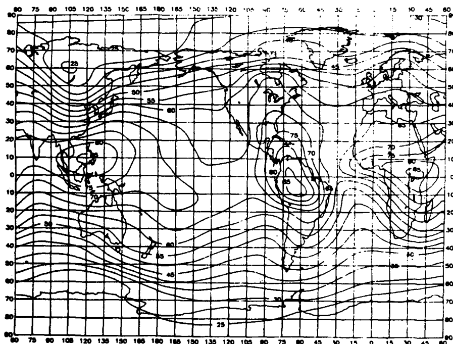
Figure 50. Expected values of atmospheric radio noise at 1 MHz, F_{am} (dB above kT_0b ), for September, October, November, 0400-0800 hours (Spaulding and Washburn, 1985).
