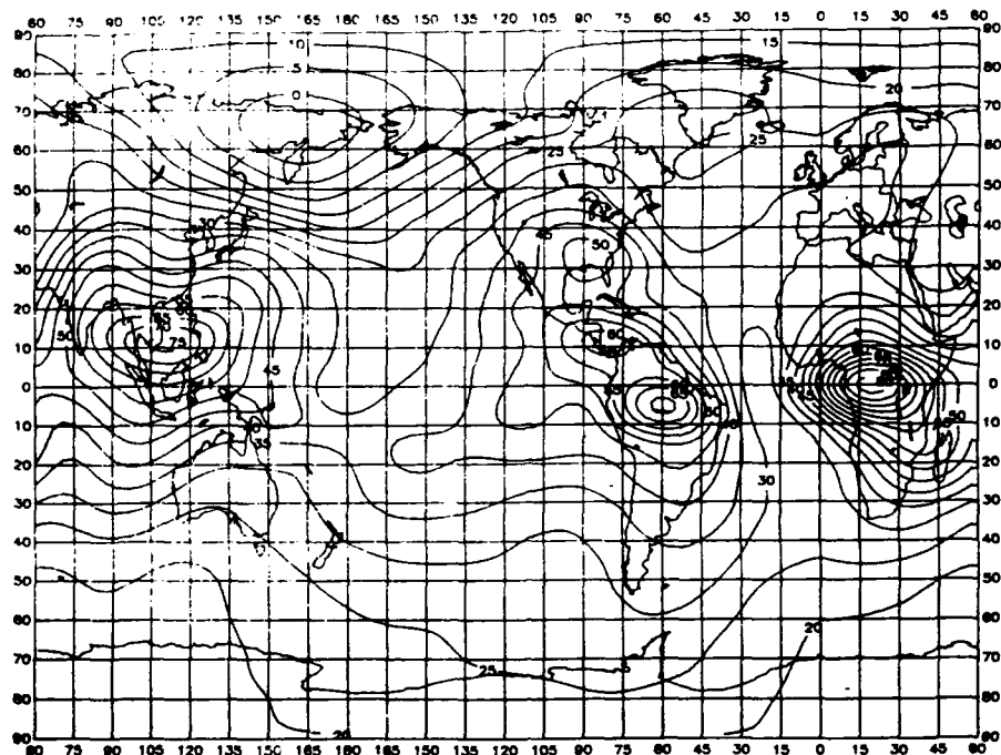
Figure 39. Expected values of atmospheric radio noise at 1 MHz, F_{am} (dB above kT_0b ), for March, April, May, 0800-1200 hours (Spaulding and Washburn, 1985).
