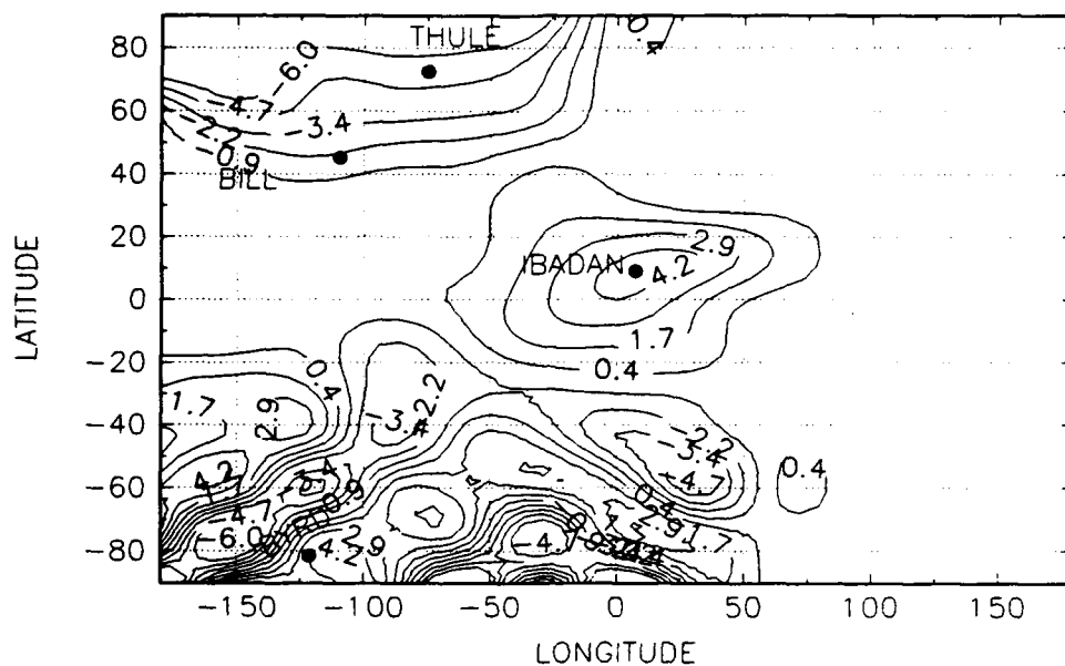
Figure 73. Geographical 1-MHz atmospheric noise model error, September, October, November, 0000-0400 hours.
