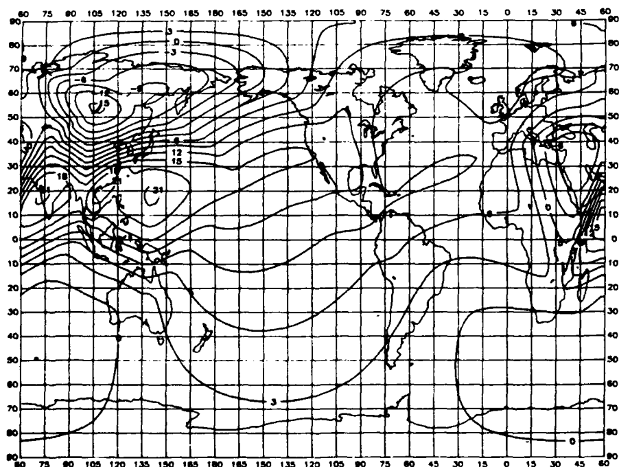
Figure 10. Corrections (dB) to original CCIR Report 322 1-MHz F_{am} estimates, December, January, February, 1200-1600 hours (Spaulding and Washburn, 1985).
