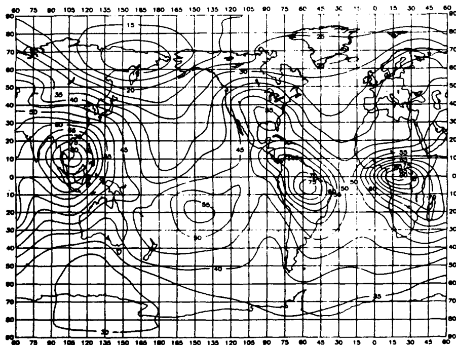
Figure 40. Expected values of atmospheric radio noise at 1 MHz, F_{am} (dB above kT_0b ), for March, April, May, 1200-1600 hours (Spaulding and Washburn, 1985).
