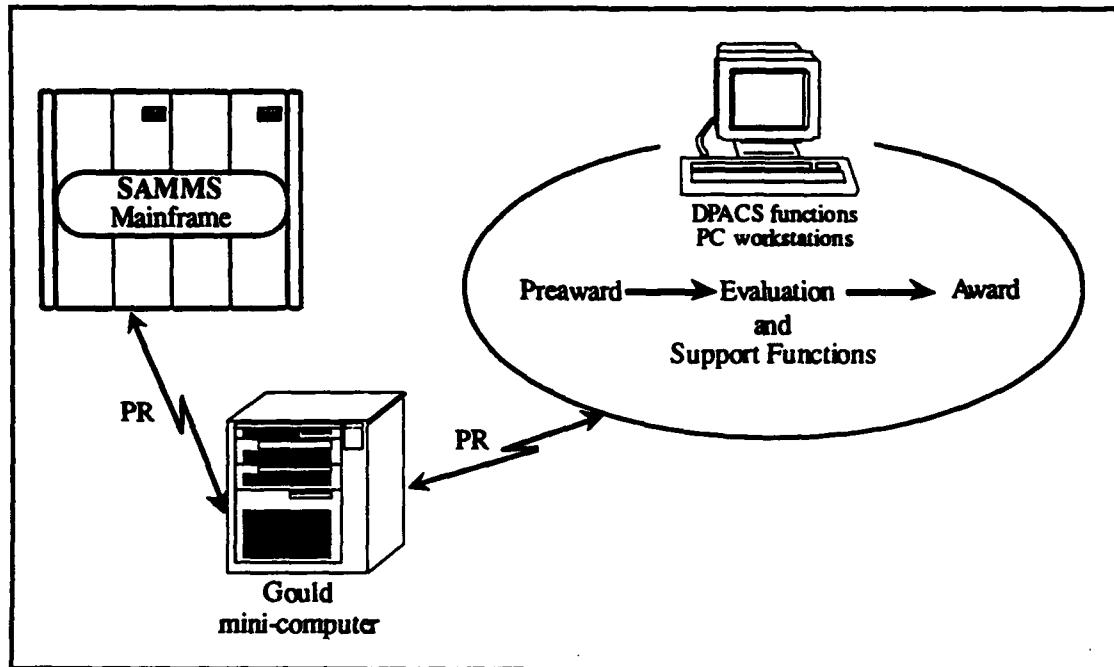
Exhibit 2-4 DPACS Configuration
