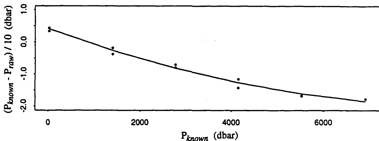
Figure 2. Pressure calibration data. Shown is the amount the pressure sensor drifted over the 5 months between the pre-cruise calibration and the post-cruise calibration ( P_{\Delta} = P_{known} - P_{raw} ) divided by ten (cruise occurred only one tenth of the way through that 5 months) as a function of pressure. The solid line shows the 2nd order polynomial fit to the drift.
