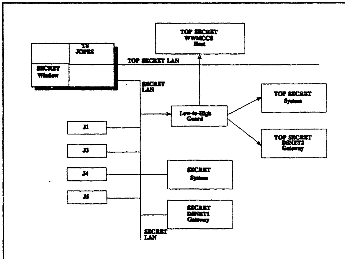
Figure 8 Workstation Architecture
