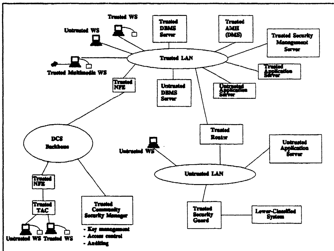
Figure 7 Target Architecture--2000
