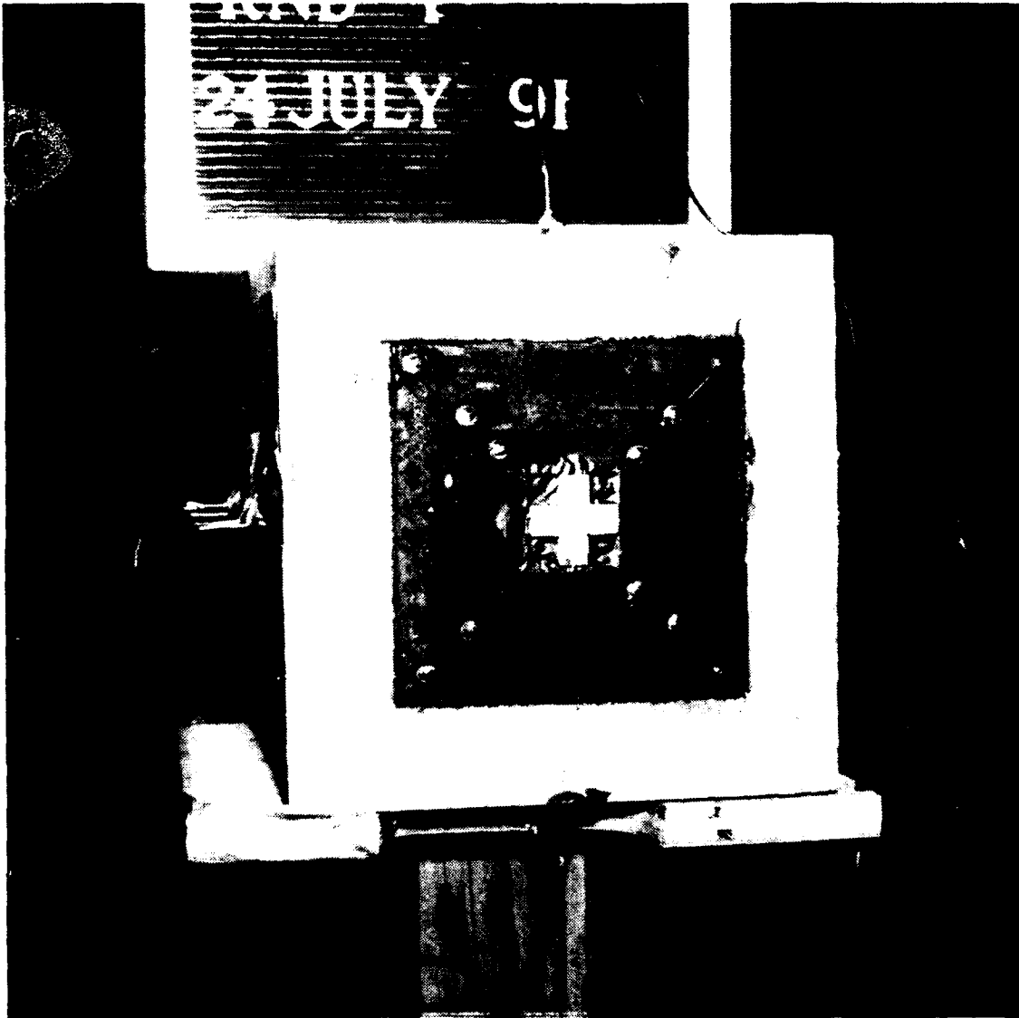
FIGURE 5. Five-Cube Fragment Confinement Frame.
