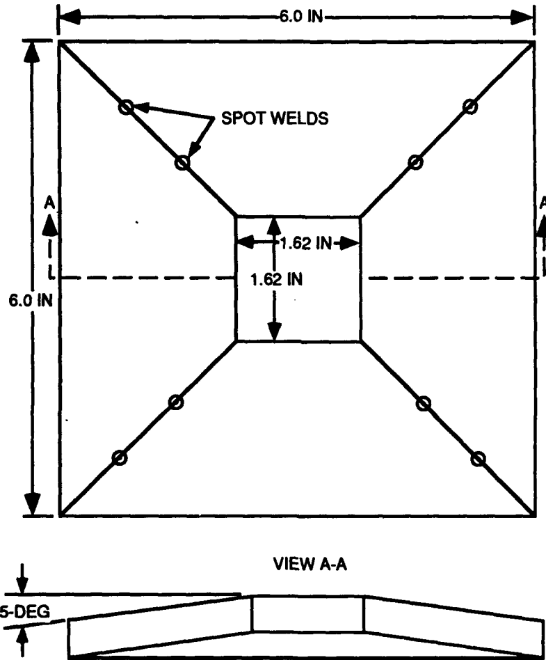
FIGURE B-2. Assembled Confinement Frame.
