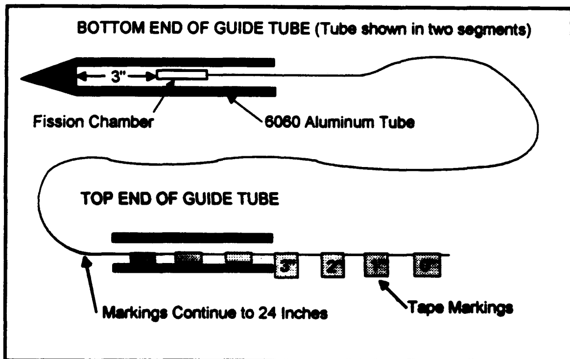
Figure 3.5.2-2: Detector Axial Position Keeping Scheme
