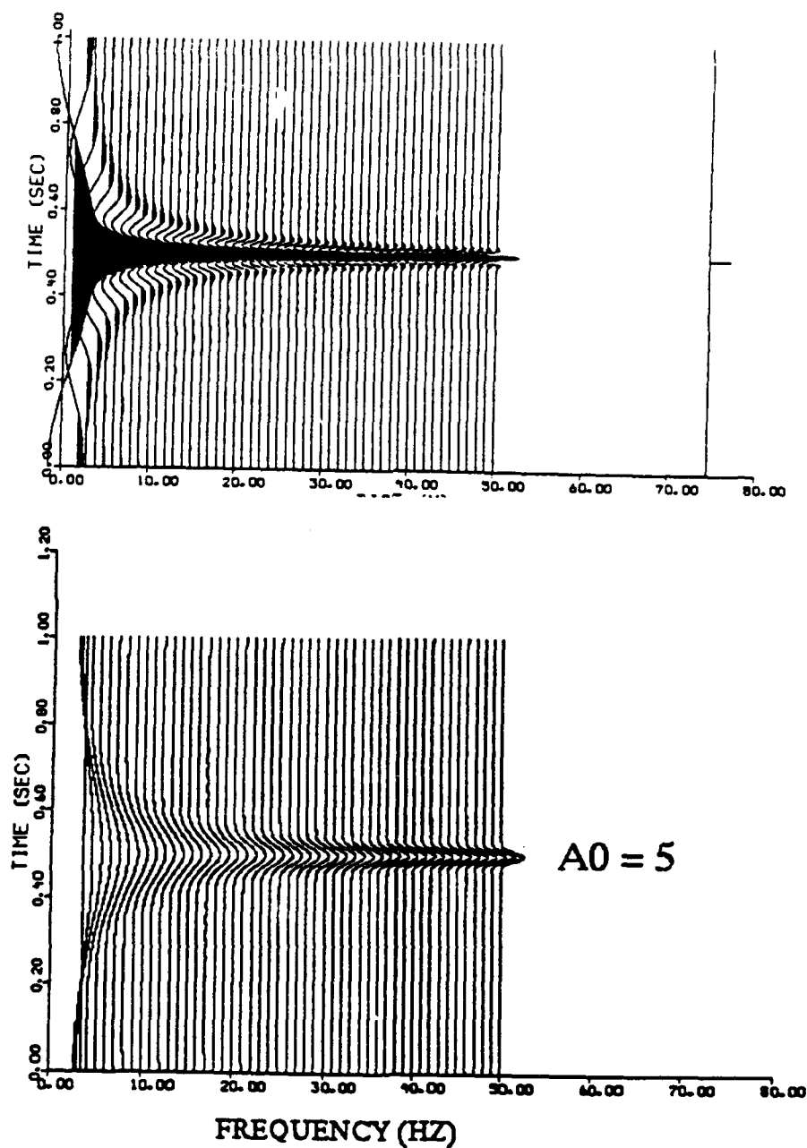
Figure 22. Impulse response in time domain of bandpass filters for different center frequencies. \alpha or A0 equals 5 in this case so bandwidth is 79%. Trace at approximately 75 Hz is input impulse trace. Bottom plot is envelope function of top plot.
