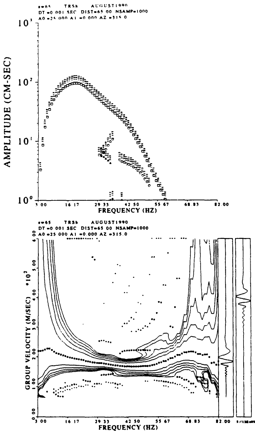
Figure 78. MFT processing of PMF stripped Love waves at 65 m. Upper plot is amplitude spectrums corresponding to lower plot group velocity dispersion. Largest amplitudes are squares, second are circles, third are triangles and fourth amplitude at a frequency is indicated by a plus sign.
