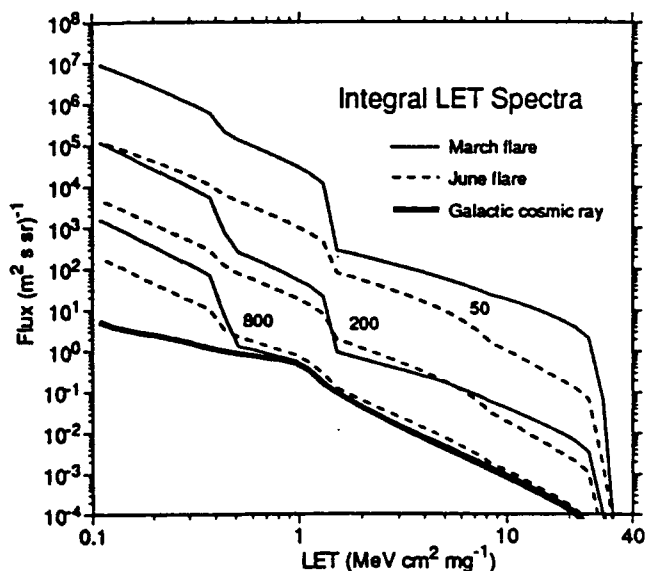
Figure 4: Integral LET spectra for the solar flares of March (solid line) and June 1991 (dashed line) are compared to the galactic cosmic ray LET spectrum (thick line). The flare LET spectra are presented for shield thicknesses corresponding to 50, 200, and 800 mils of aluminum.
