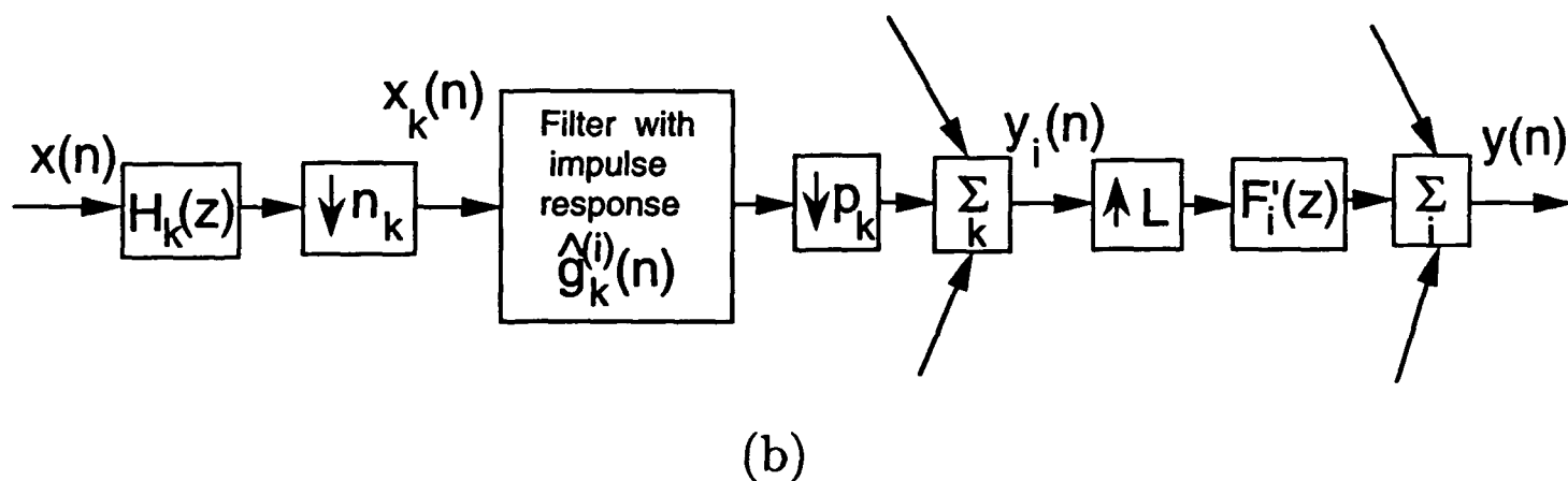
Fig. 4.1. The low sensitivity structures for FIR filters, (a) with one-level filter bank convolver, (b) with two-level filter bank convolver.
