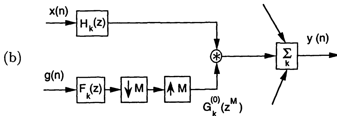
Fig. 8.1. Relationship between convolver and IFIR filter, (a) implementation of IFIR filter, (b) implementation of convolver.
