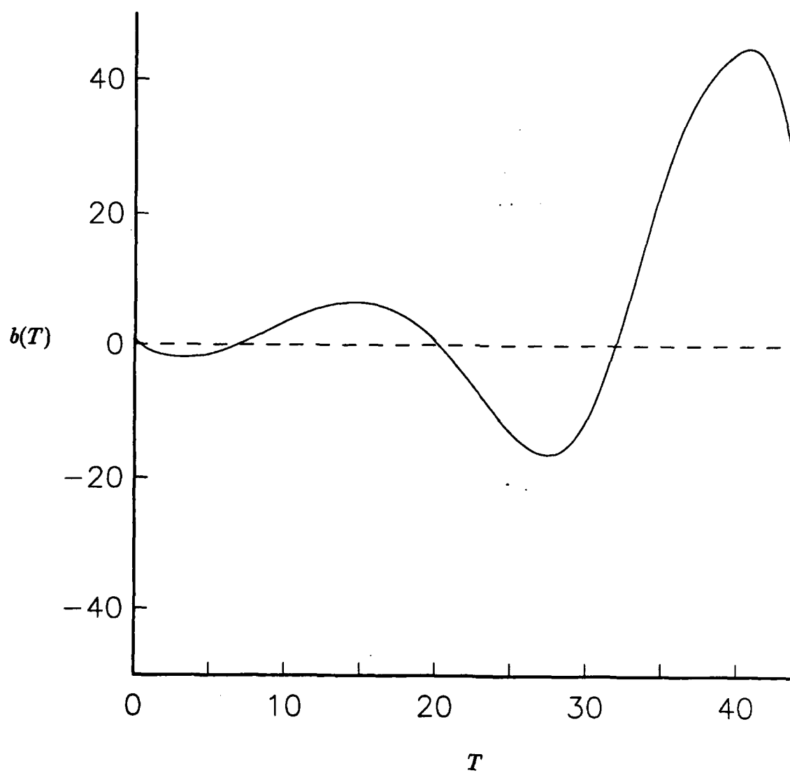
Figure 5.4a Solution of the J_1 evolution equation for \nu = -0.4 .
