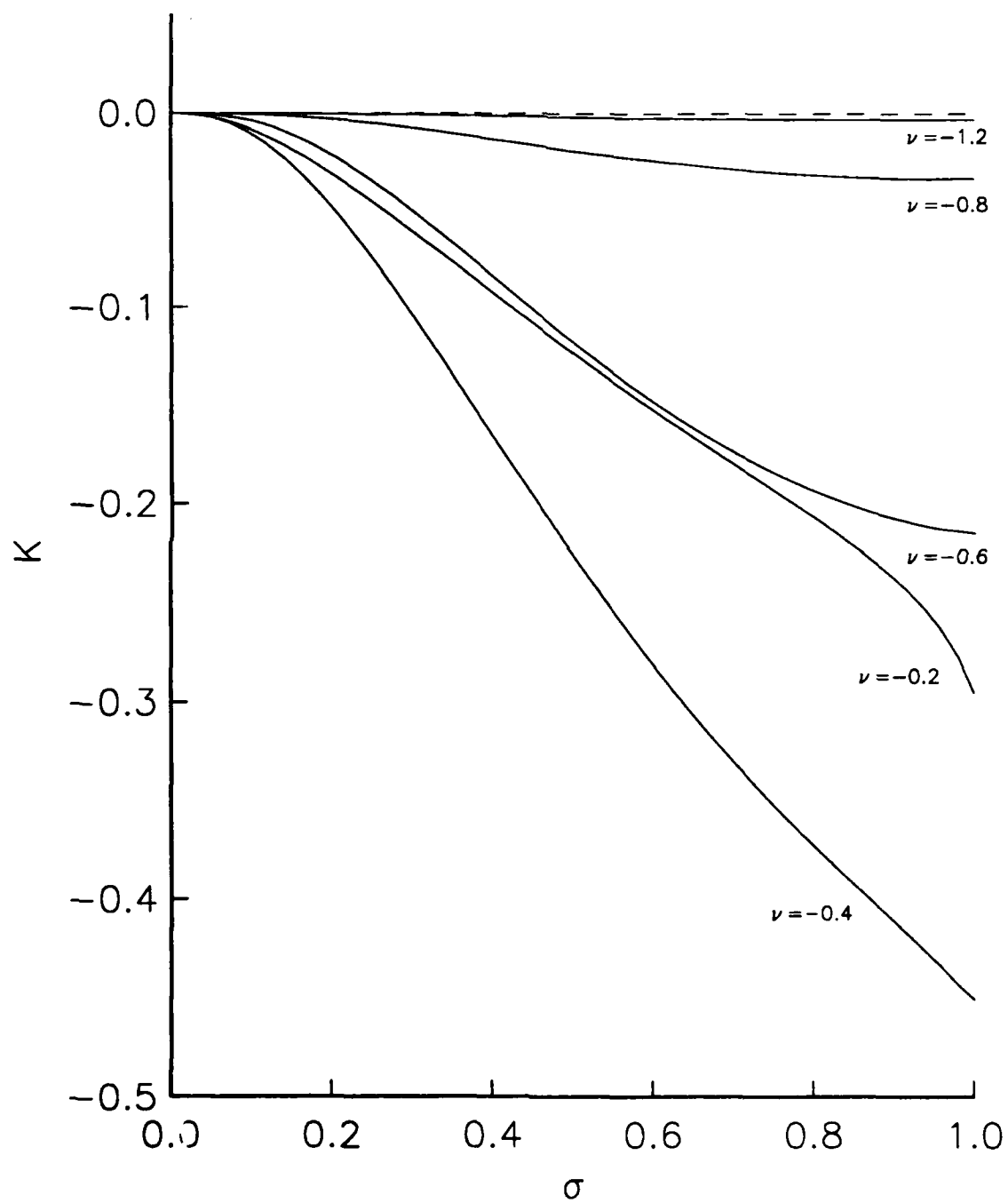
Figure 5.3 The kernel K for various values of \nu .
