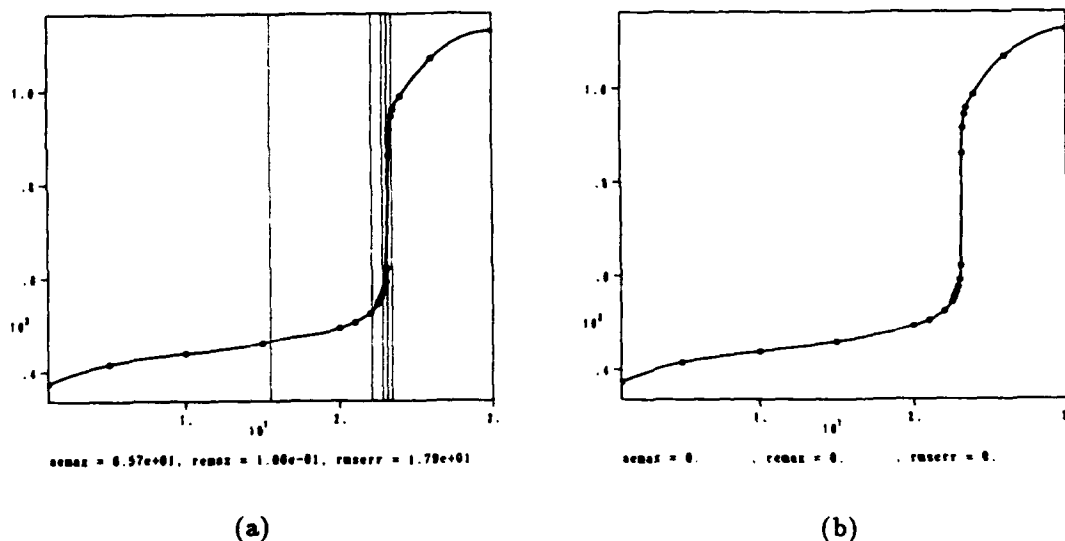
Figure 5. Two approximations to potentiometric titration data. (a) The PCHLS fit with n=7 and equidistributed breakpoints. (b) The PCHIP interpolant.
