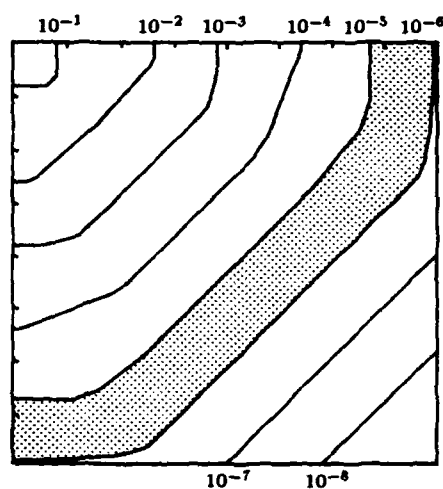
Figure 4 Convex hulls: \phi(r) = r^2 \log r
