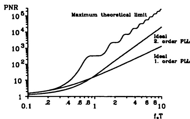
Figure 2: Phase noise reduction as a function of normalized loop bandwidth f_z T .
