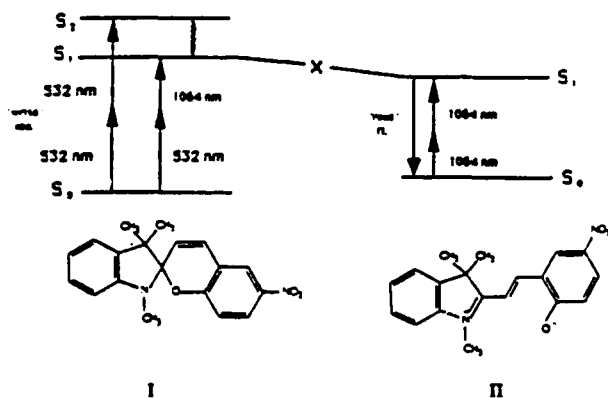
Fig. 1. Schematic energy level diagram of the write and read forms of the photochromic molecule. "X" is an intermediate to the isomerization of the spirobenzopyran. The structures of the two forms of SP as well as the laser wavelengths used for writing and reading are shown also.
