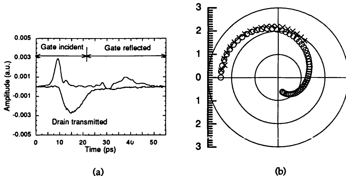
Fig. 1 (a) Electrical transients input to and reflected from the gate and output from the drain of a HEMT device, as measured on a coplanar-stripline test fixture via external electro-optic sampling. These are the waveforms necessary to determine both forward S -parameters of the device. Similar waveforms have been measured in order to acquire the reverse characteristics. (b) A polar plot of the S_{21} transmission coefficient for the HEMT, extracted from electro-optic data to 100 GHz (O) and conventional rf network analysis to 40 GHz (X). Without extrapolation, one can observe from the electro-optic network analysis the point where the transmission coefficient crosses the unity circle and becomes less than one.
