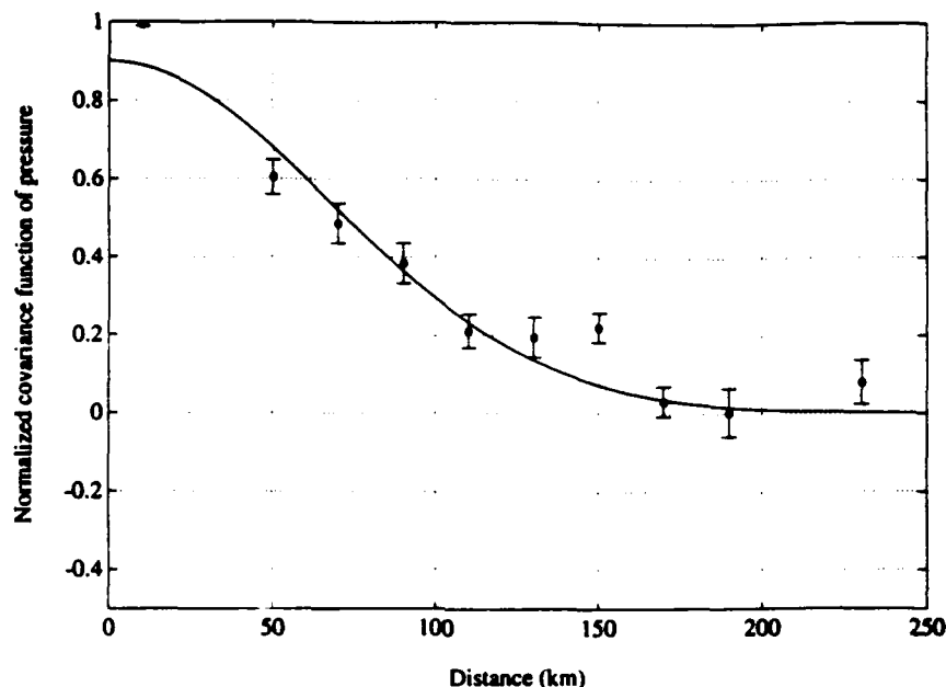
Figure 3: Spatial correlation function of the pressure fields.
