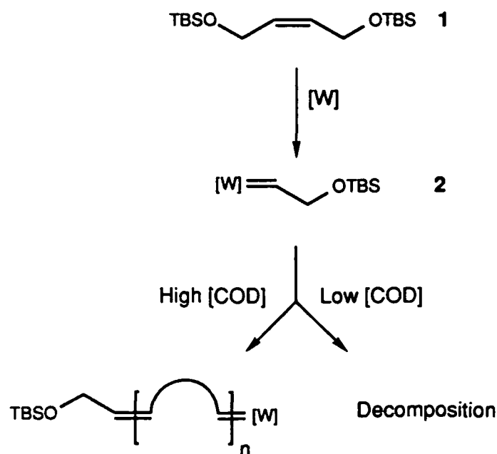
Figure 1. Fate of metal alkylidene fragment (2) in the preparation of HTPB by the ROMP of COD in the presence of 1.
