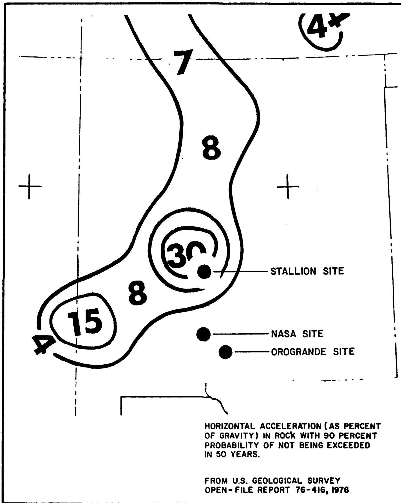
Figure III-6. Site Area Horizontal Components of Acceleration Caused by Earthquakes.
