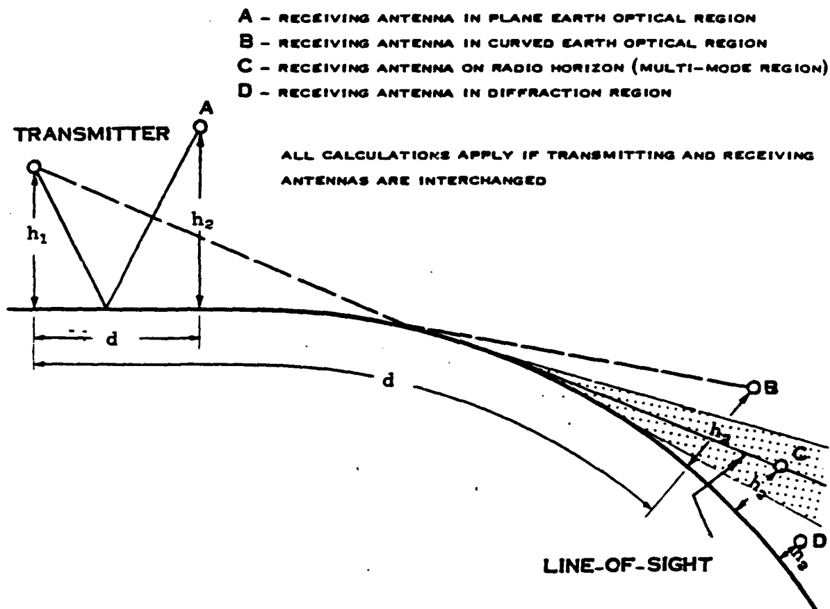
Figure 3-1 Diagram of Propagation Regions
