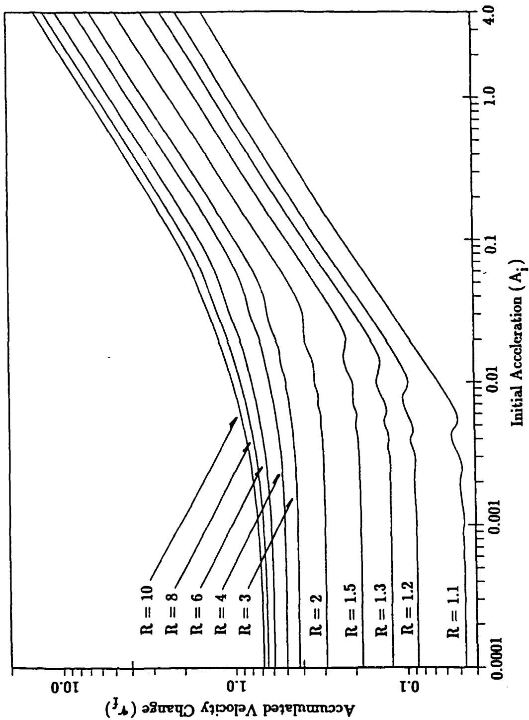
FIG. 3 v_f contours for various orbit ratios R ( m_p = 0.5 )
