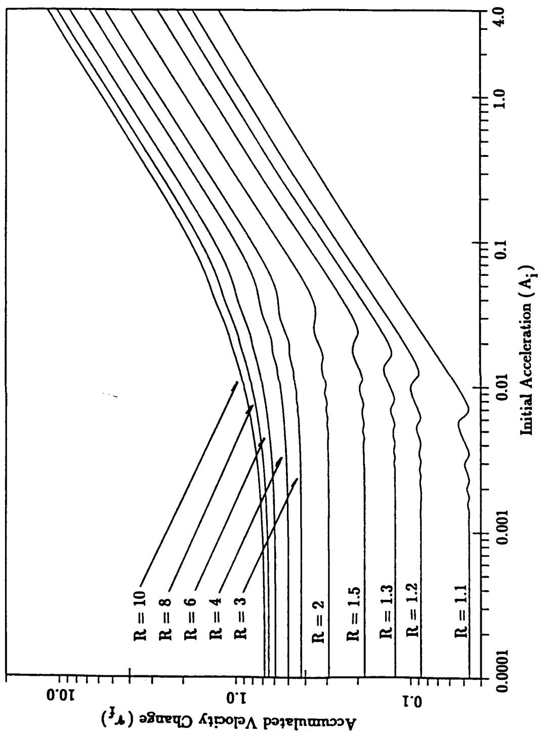
FIG. 1 v_f contours for various orbit ratios R ( m_p = 0 )
