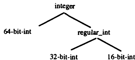
Figure 14: Integer Family
