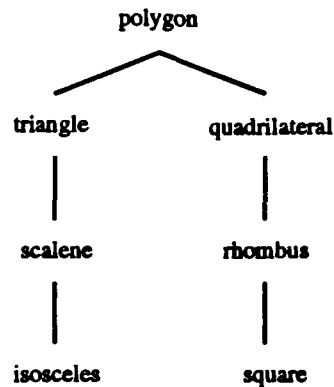
Figure 10: Polygon Hierarchy
