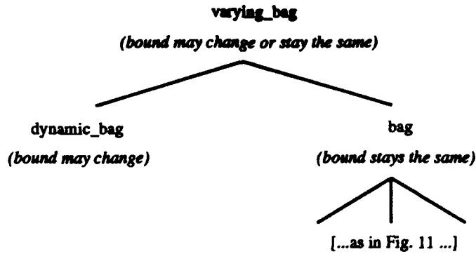
Figure 12: Another Type Family for Bags
