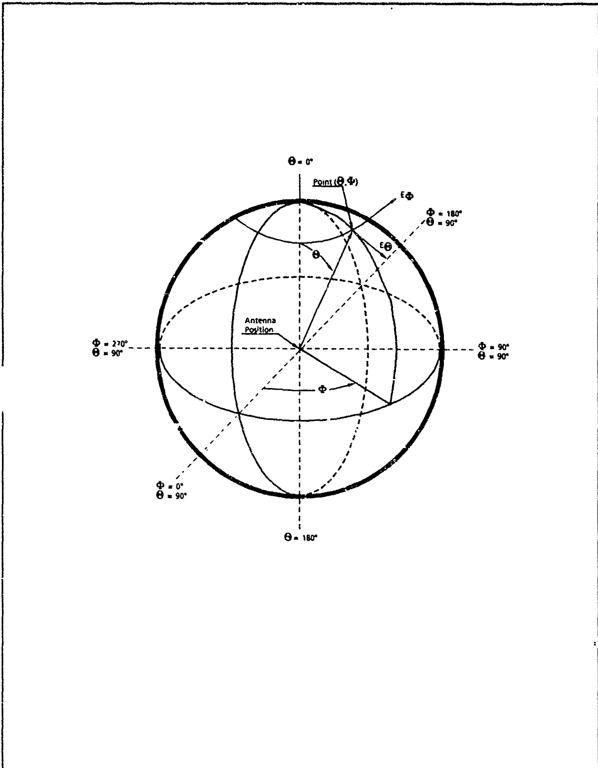
Figure 3-2. Spherical Antenna Coordinate System.
