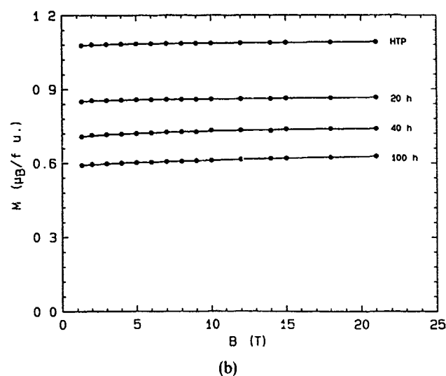
Fig. 3. Magnetization at 4.2 K of CrFe after different milling times. The magnetization at 4.2 K of the quenched CrFe sample (from 880°C) is also included for comparison (marked as HTP).
