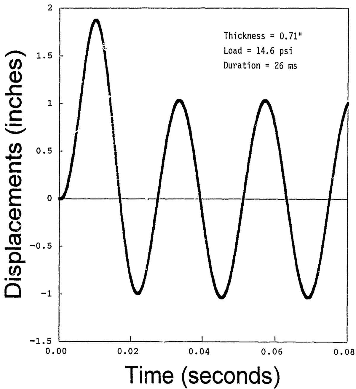
Figure 5-2. Displacements of a 72" x 72" Window Plate
