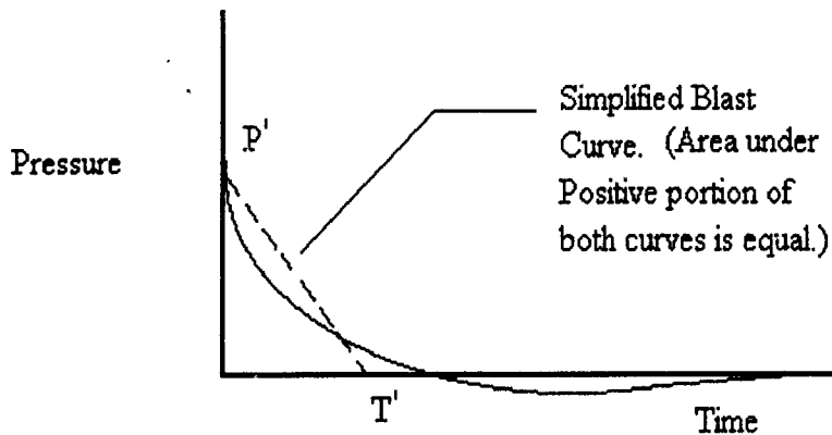
Figure 3-2. Simplified Blast Curve
