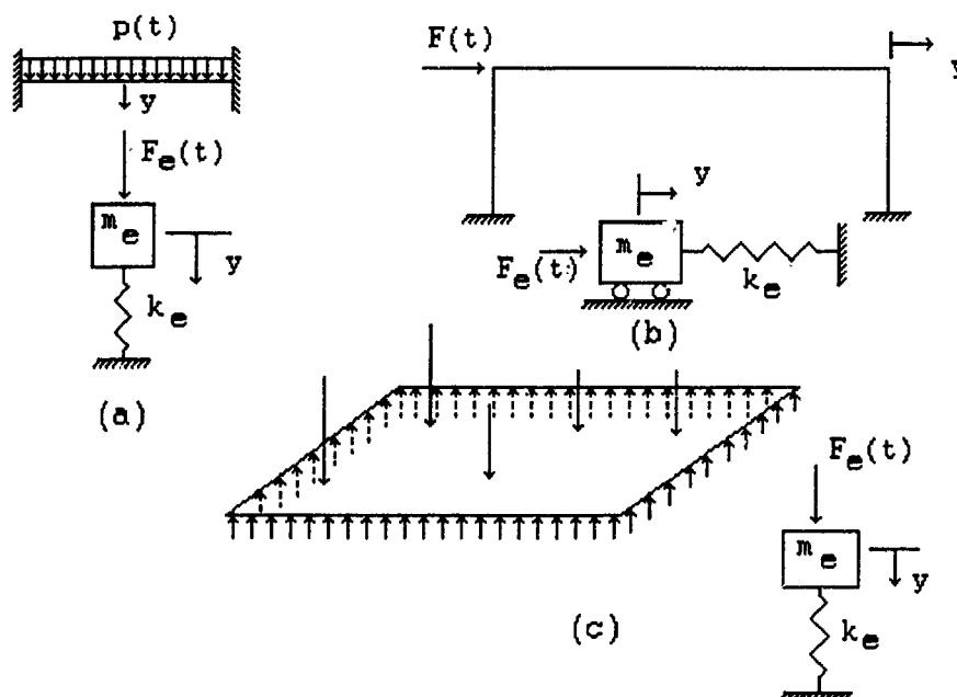
Figure 3-5. Equivalent one-degree systems.
