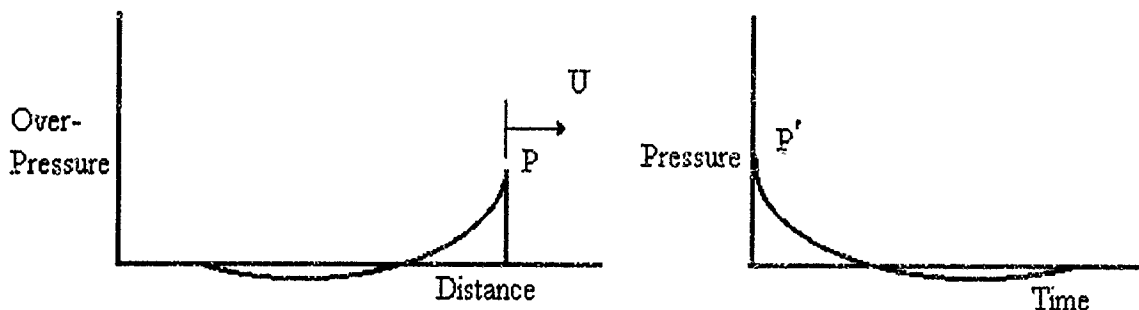
Figure 3-1. Blast Shapes
