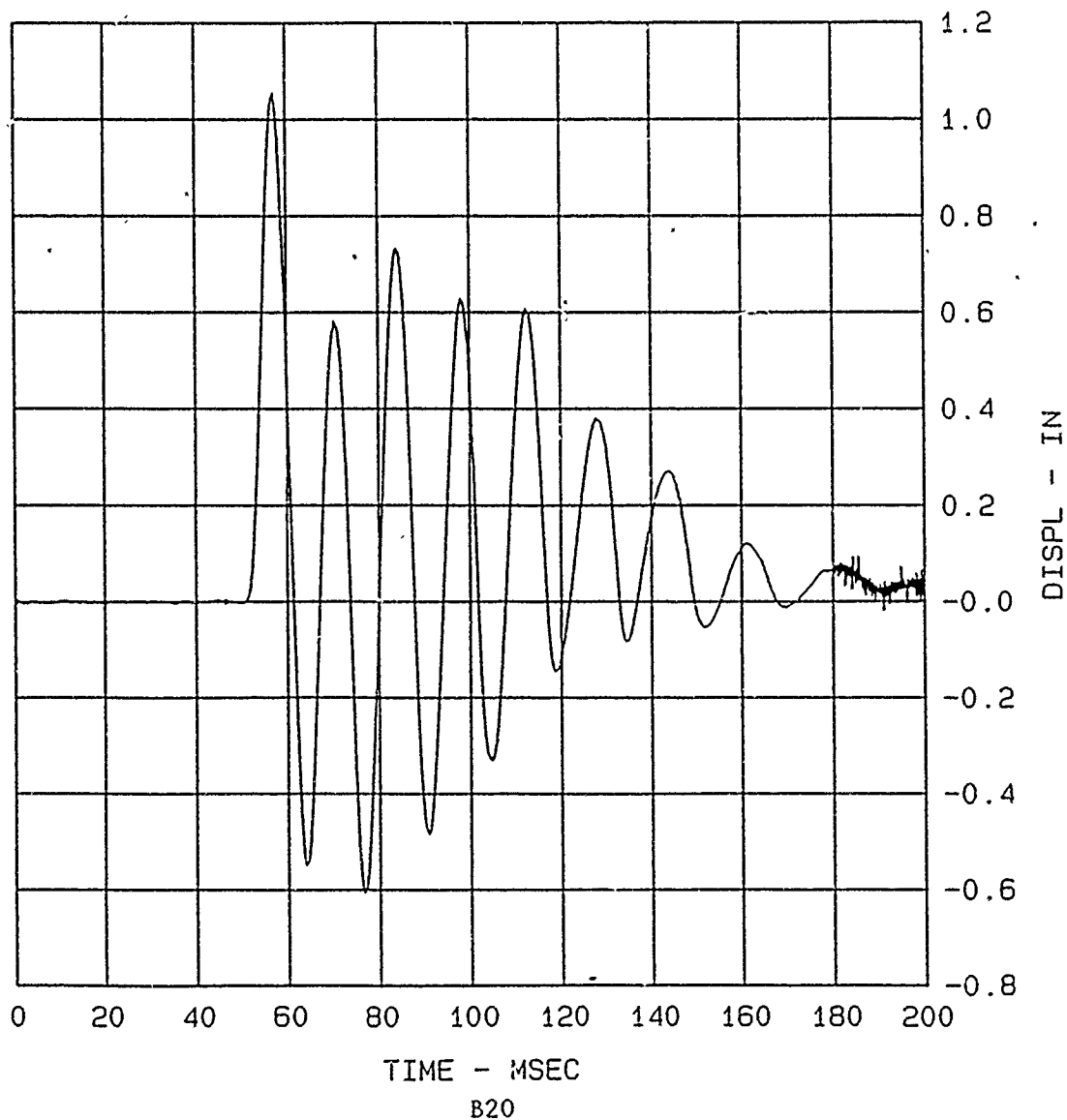
Figure 5-8. Sample Graphical Output of Experimental Data
