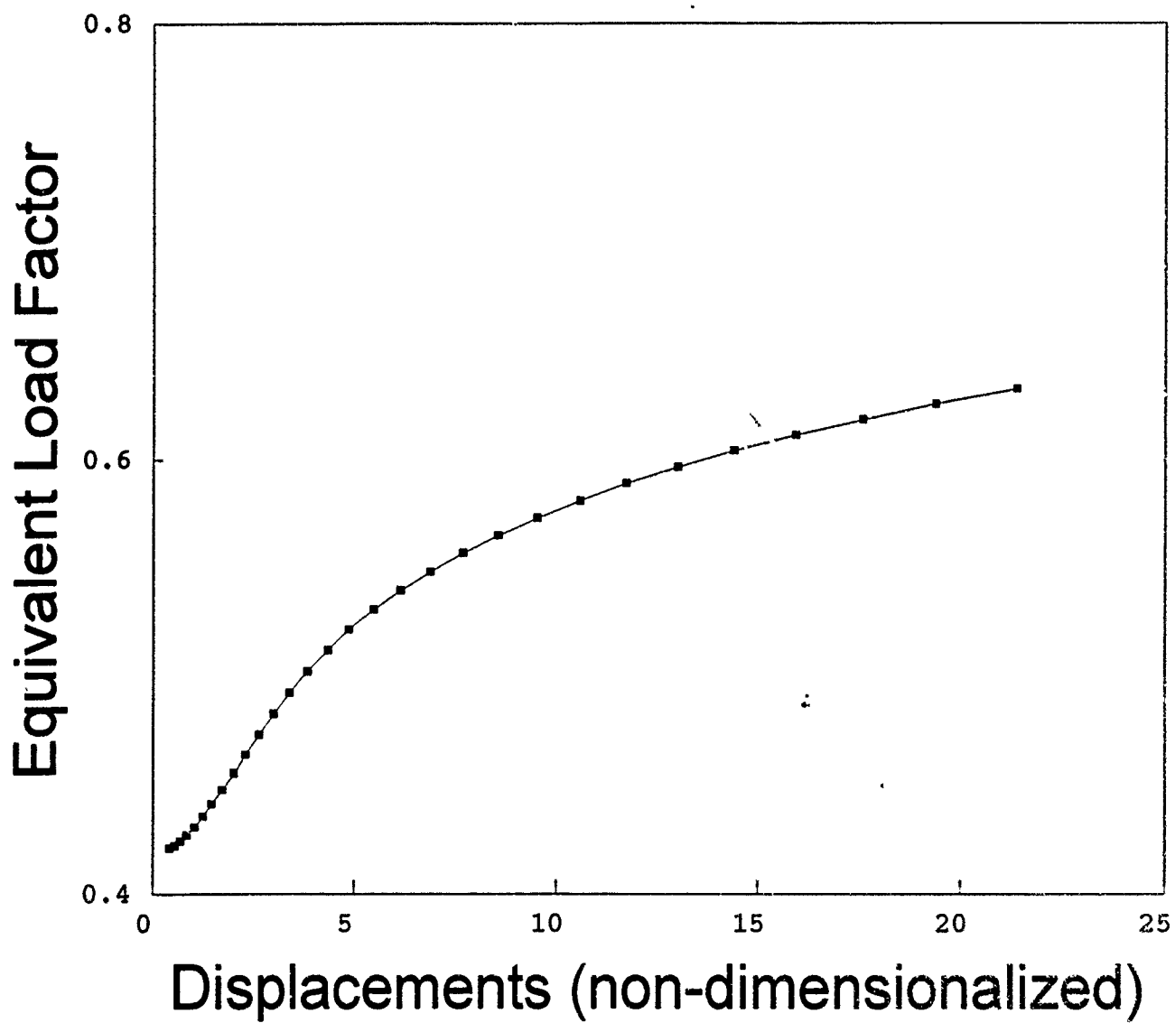
Figure 4-3. Equivalent Load Factor (Square Glass Plates)
