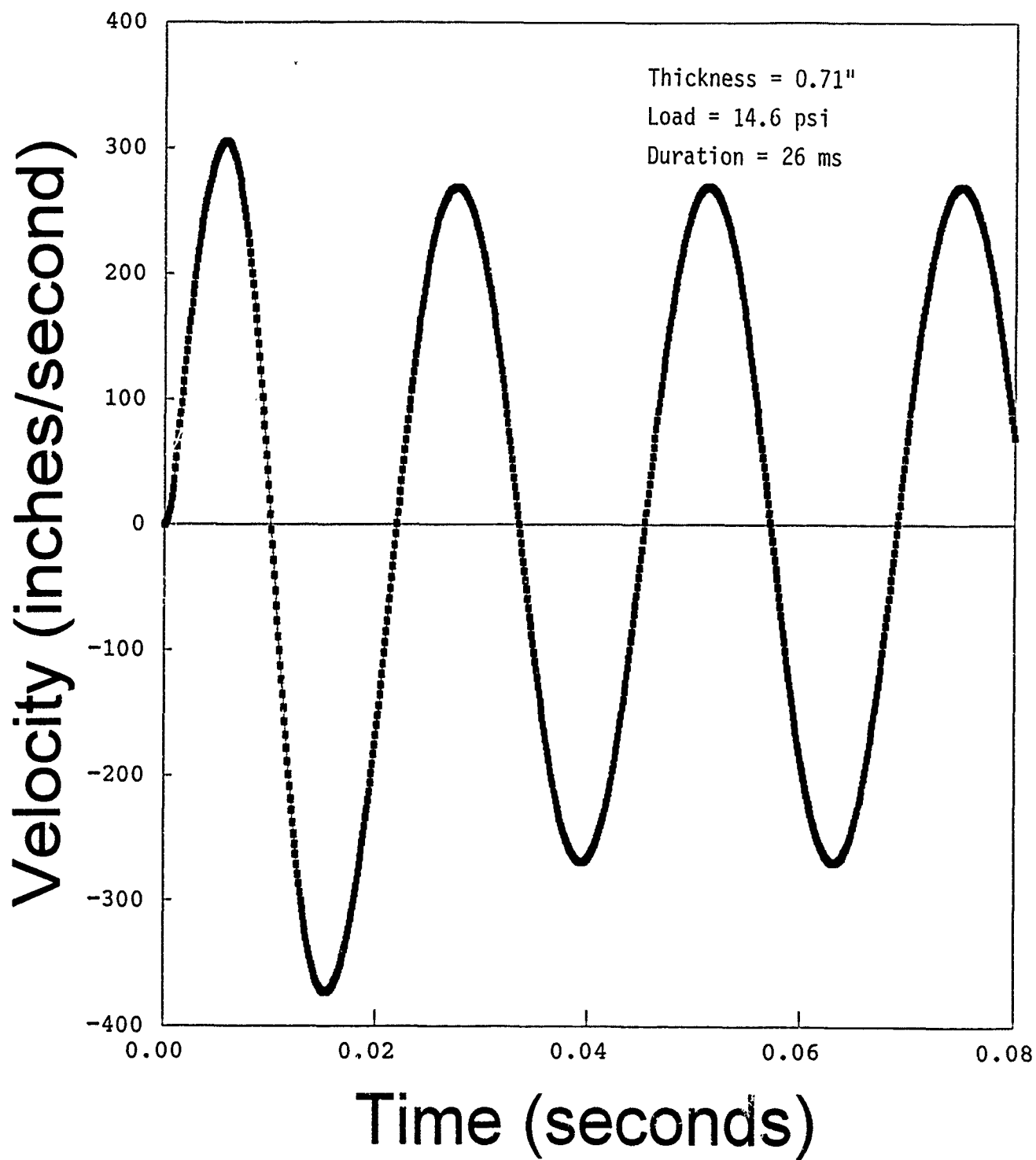
Figure 5-3. Velocity of a 72" x 72" Window Plate
