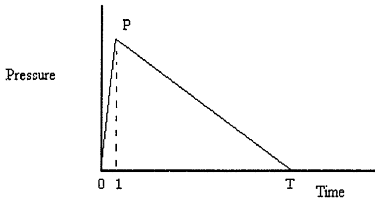
Figure 3-3. Modified Blast Curve
