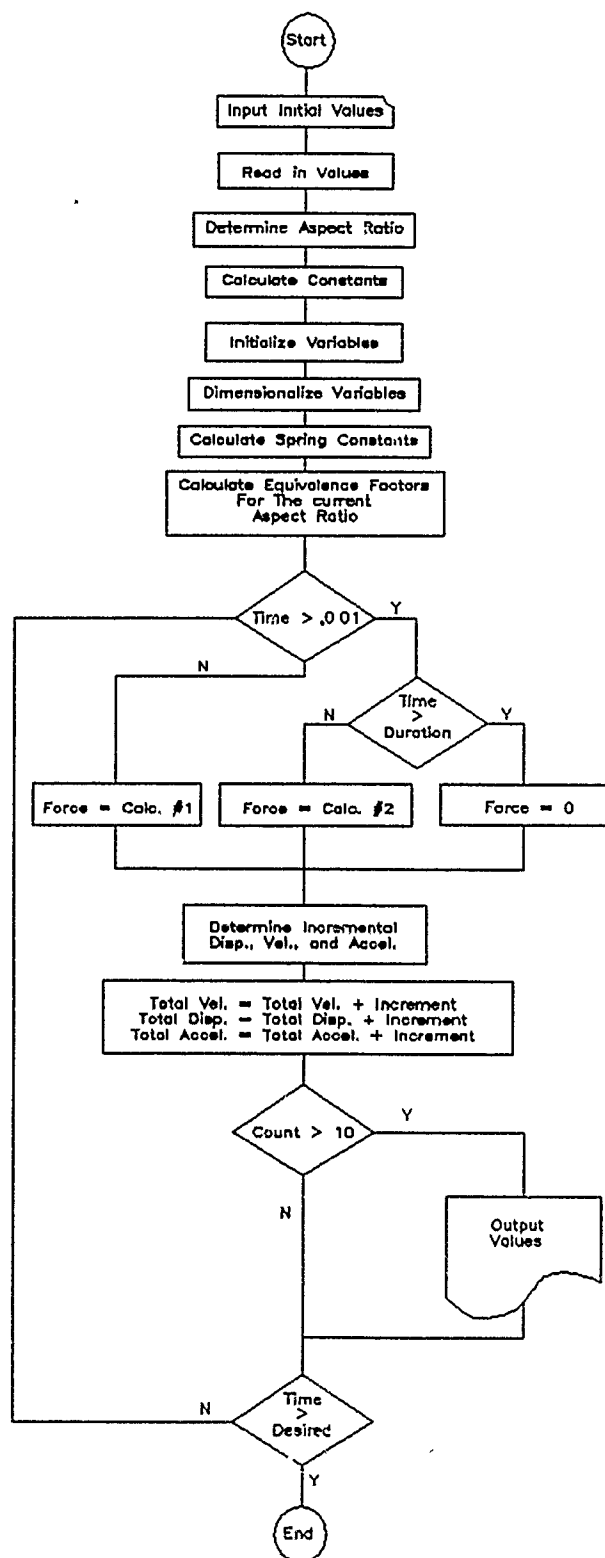
Figure 4-5. Flowchart for WINBLAST
