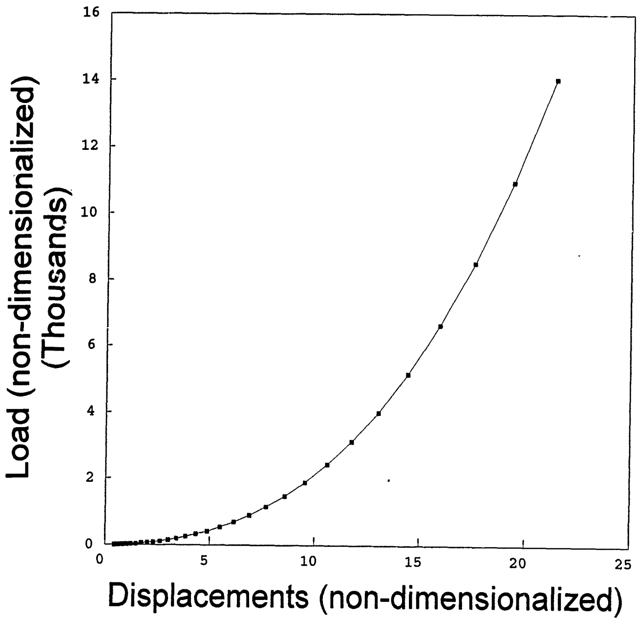
Figure 4-1. Displacements -vs- Load (Square Glass Plates)
