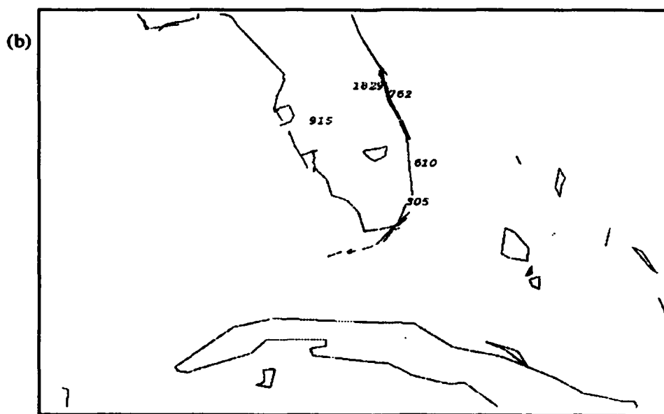
Figure 23 GEMPAK plots of West Palm Beach sounding data at 1200 UTC 24 August 1992 (a) and observed low cloud bases (m) at the same time (b).
