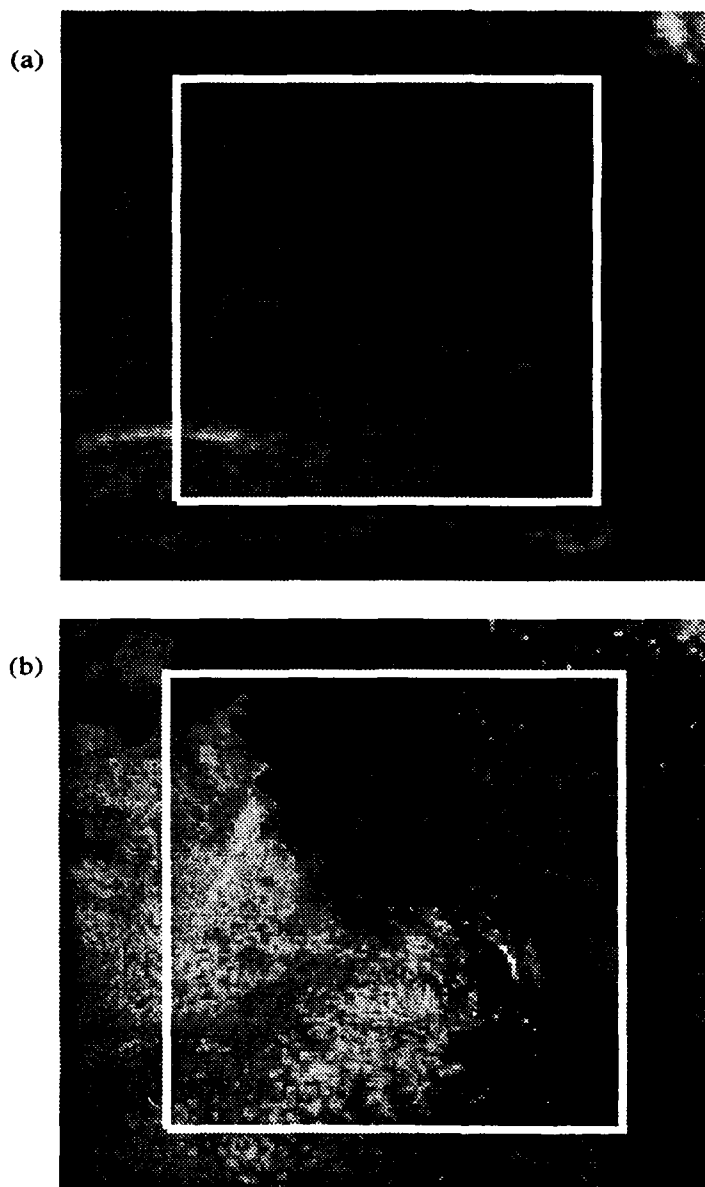
Figure 10 Enlarged views of the GOES IR (a) and visible (b) subimages of the California coastline at 1801 UTC 31 August 1992. Area to be displayed in 3-D indicated by box.
