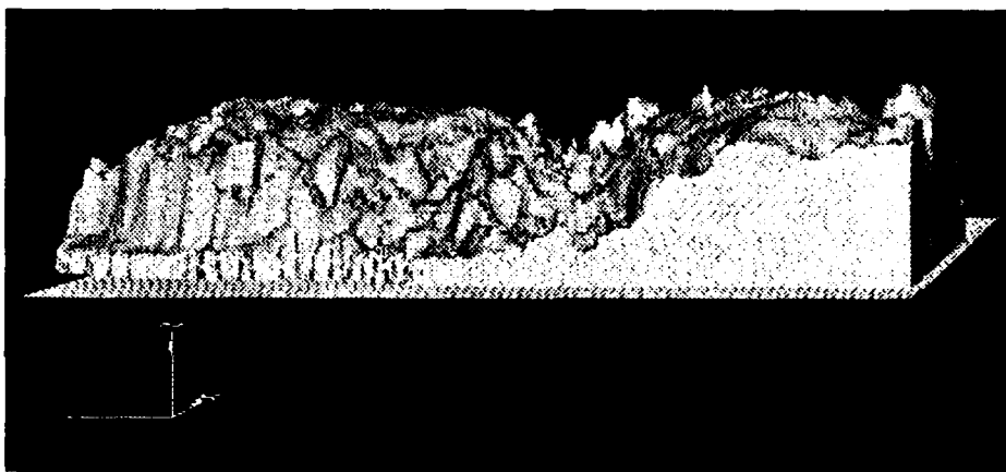
Figure 2 View from the north (a) and from the south (b) of a 3-D cloud display constructed from GOES IR imagery using techniques described by Owen.
