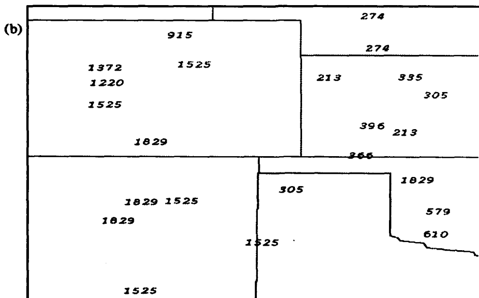
Figure 13 GEMPAK plots of Dodge City sounding data at 0000 UTC 31 October 1992 (a) and observed low cloud bases (m) at 2200 UTC 30 October 1992 (b).
