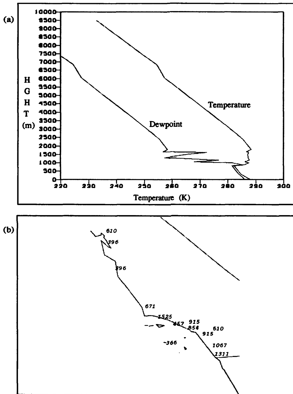
Figure 6 GEMPAK plots of Oakland sounding data at 1200 UTC 31 August 1992 (a) and observed low cloud bases (m) at 1800 UTC 31 August 1992 (b).
