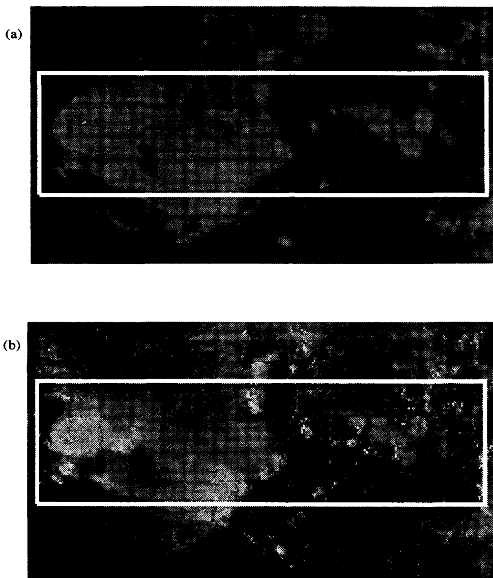
Figure 20 Enlarged views of the GOES IR (a) and visible (b) subimages covering the Gulf Coast region at 2101 UTC 3 September 1992. Area to be displayed in 3-D indicated by box.
