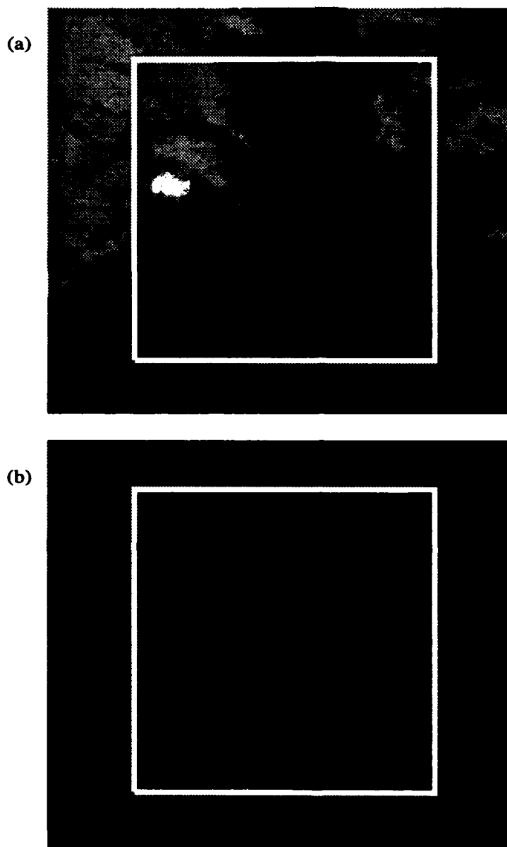
Figure 15 Enlarged views of the GOES IR (a) and visible (b) subimages covering the eastern Rocky Mountains and western Great Plains at 2201 UTC 30 October 1992. Area to be displayed in 3-D indicated by box.
