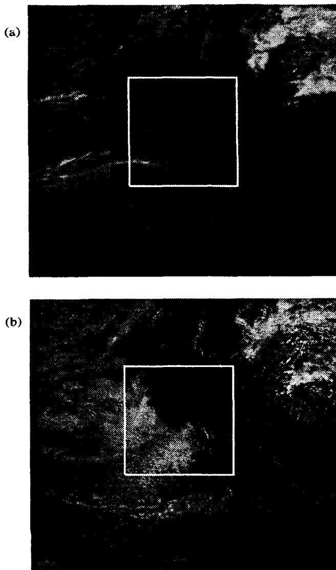
Figure 5 Sectors of GOES IR (a) and visible (b) images covering the western U.S. at 1801 UTC 31 August 1992. Area to be displayed in 3-D indicated by box.
