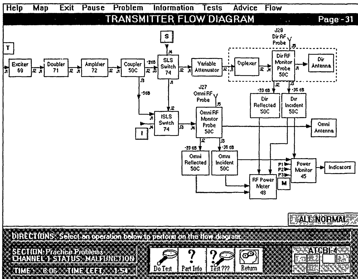
FIGURE 8. EXAMPLE FUNCTIONAL FLOW DIAGRAM SCREEN
