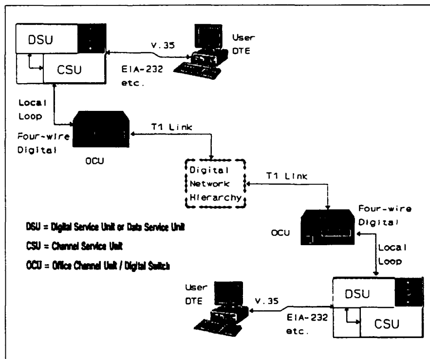
Figure 1: Digital Circuit Structure
