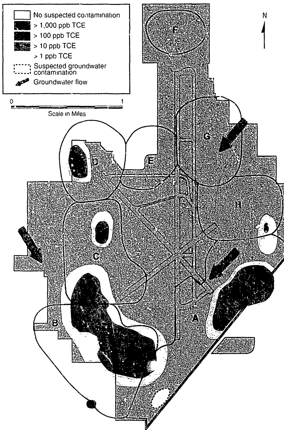
Figure 2-2 Groundwater Contamination at MCAF B
