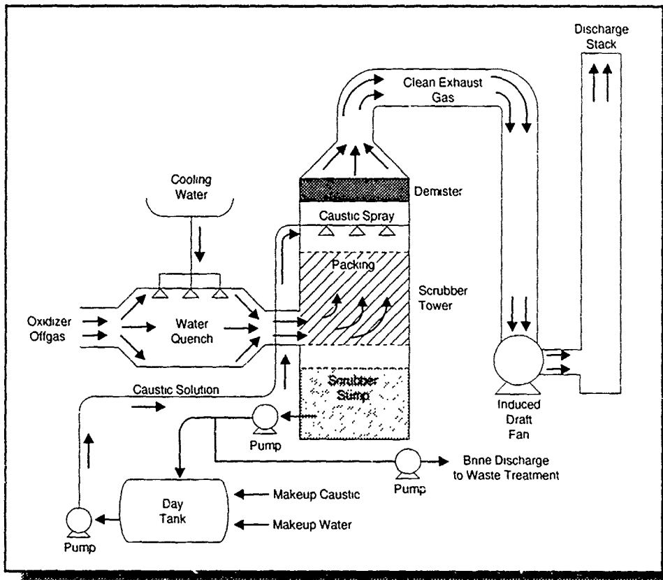
Figure 6-2 Scrubber System Schematic
