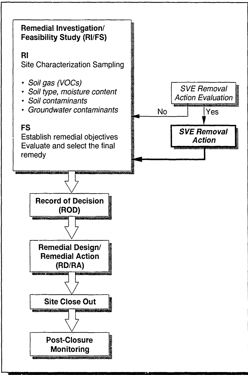
Figure 1-2 SVE Removal Action and IRP
