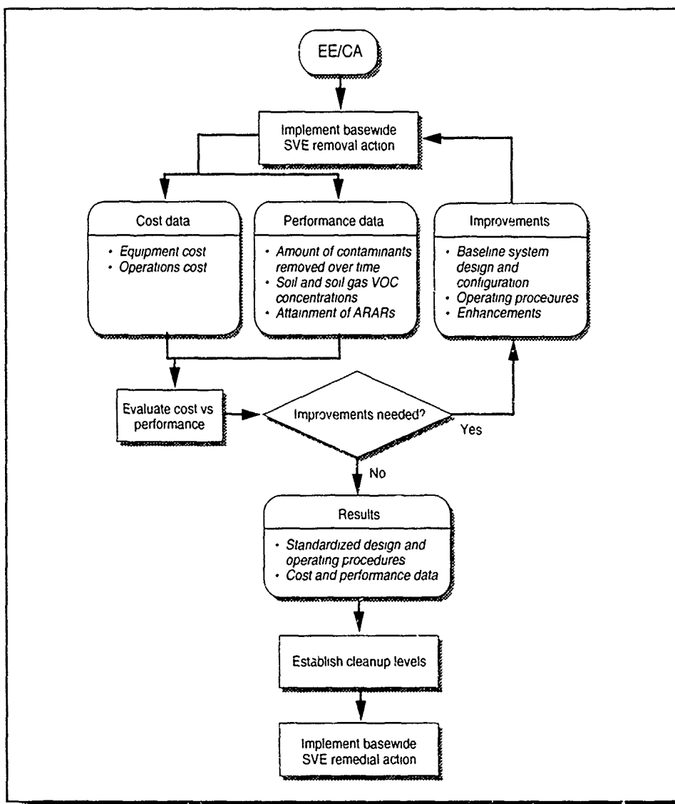
Figure 8-1 Basewide SVE Removal Action: Laying the Foundation for Basewide SVE Remediation
