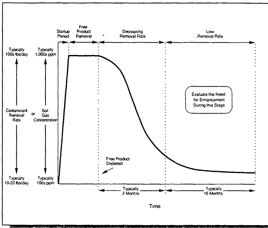
Figure 8-2 Typical Mass Removal Rate During Operation of SVE Systems (Not to Scale)
