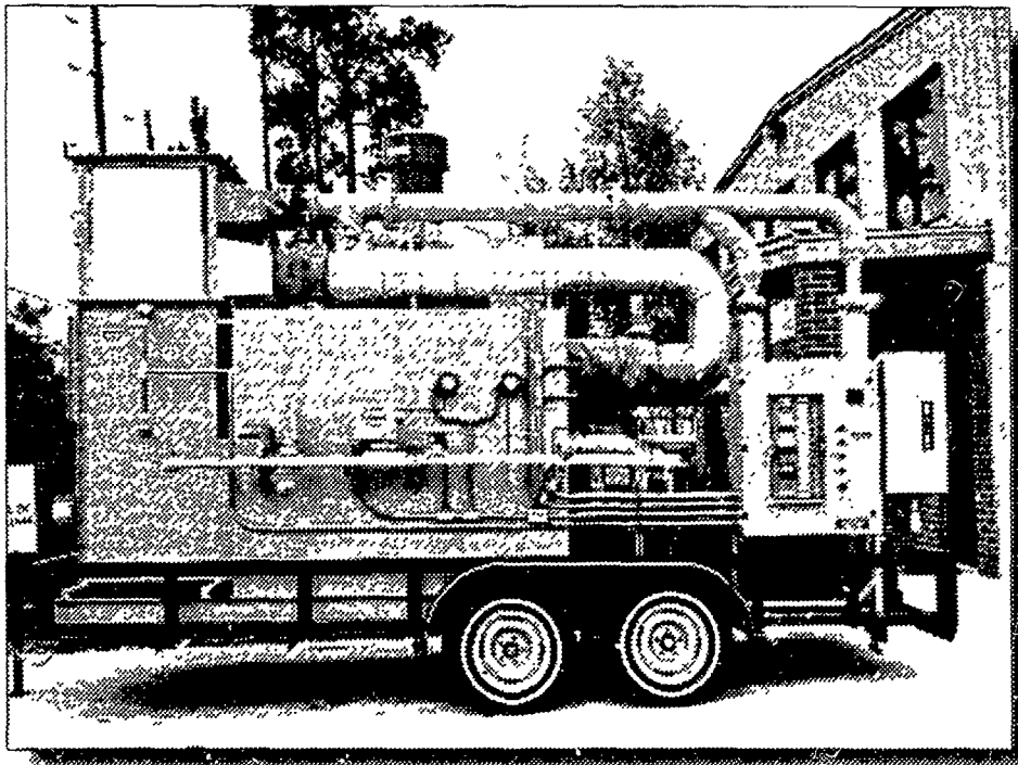
Figure 6-3 Trailer- Mounted SVE Unit
