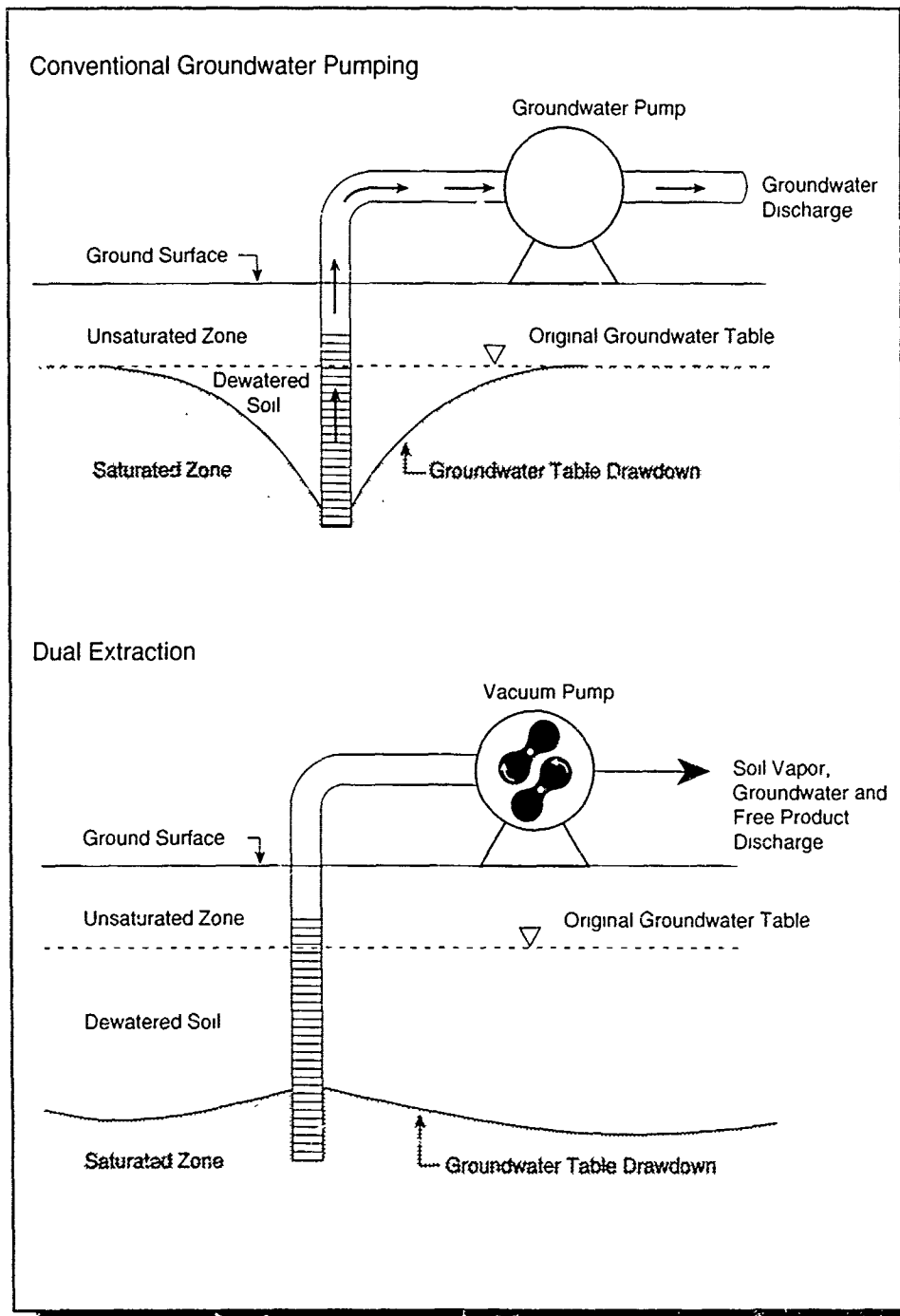
Figure 7-1 Principle of Dual Extraction
