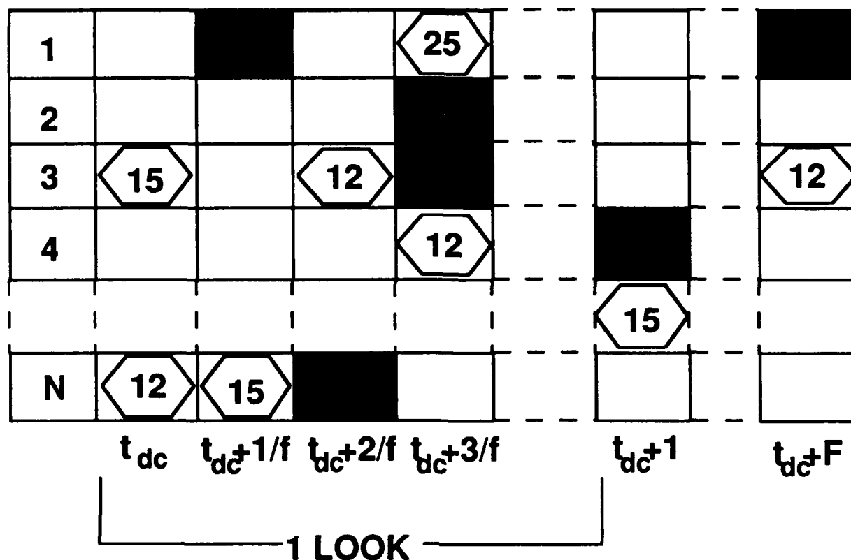
Figure 2: SCHEMER "Movie"
