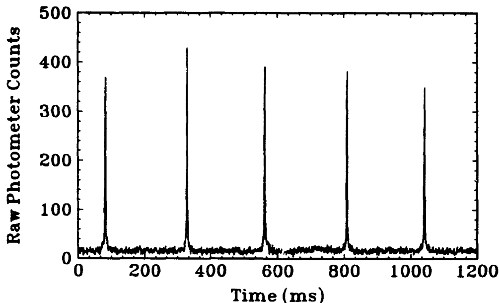
Figure 6. High speed photometry of object ETS 97034.
