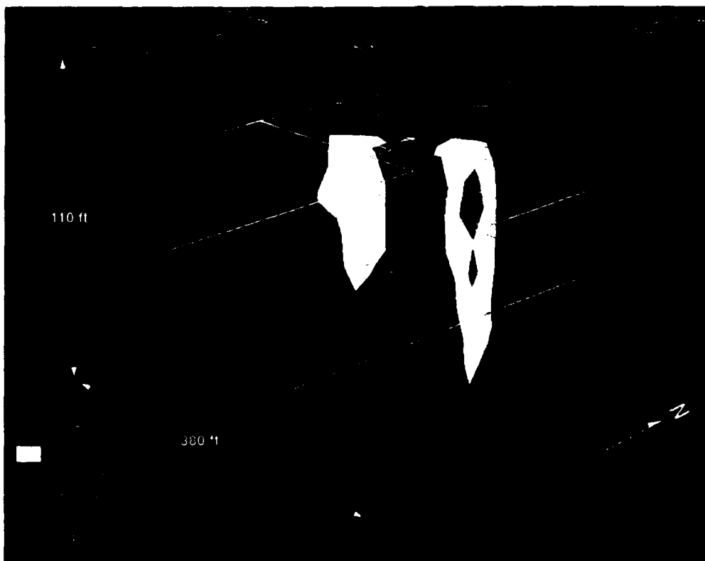
Figure 2-7 IC 7—Three-Dimensional Model of TCE Plumes (Left Plume at Washrack Right Plume at TWT)
