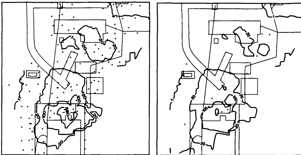
Figure 2-4c Distribution of DCE12C (ppmv) in Soil Gas Regardless of Soil Type
