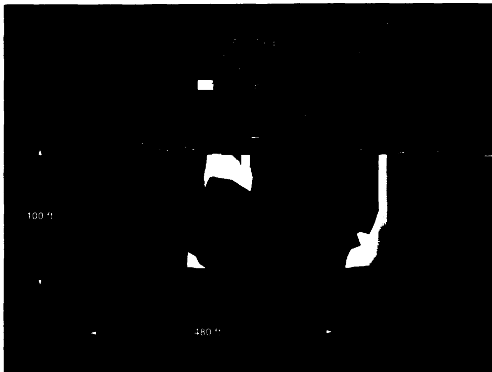
Figure 2-8 PRL-S-35 Plume. Distribution of TCE in an East-West Cross Section
