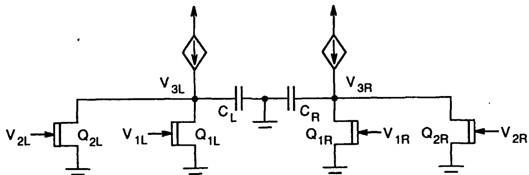
Figure 3.4. Integrating stage of the integrator.
