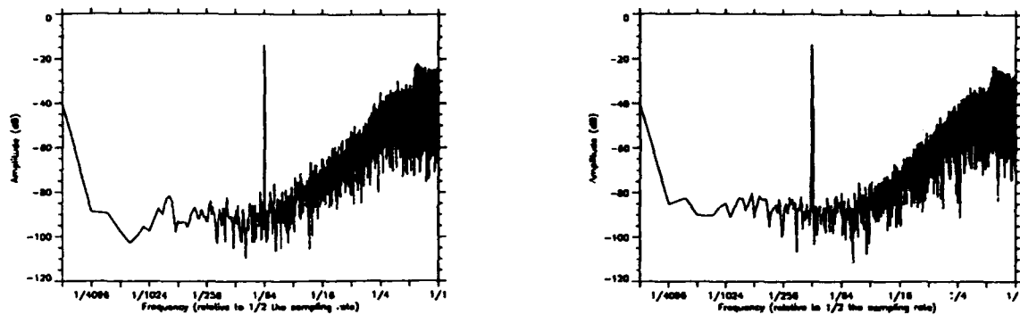
Figure 4.20. Frequency spectrums of half-scale 4 MHz and 2 MHz inputs.
