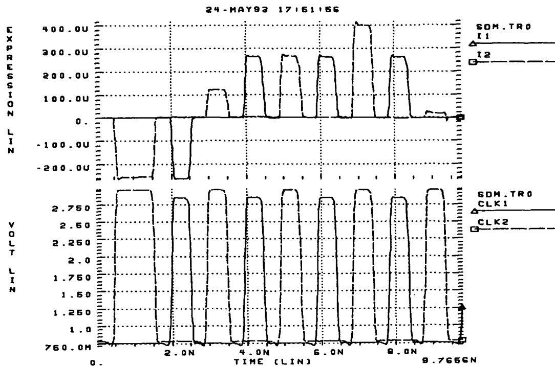
Figure 3.3. Currents through the integrating capacitors of the both integrators.
