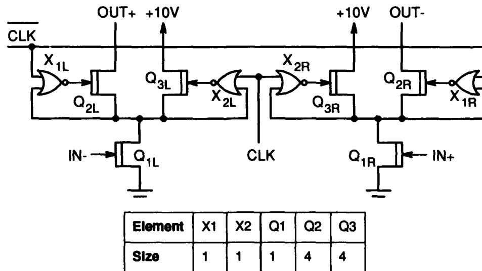
Figure 3.11. Clocked delta transconductor.
