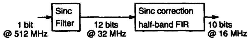
Figure 5.1. Stages of the filter.
