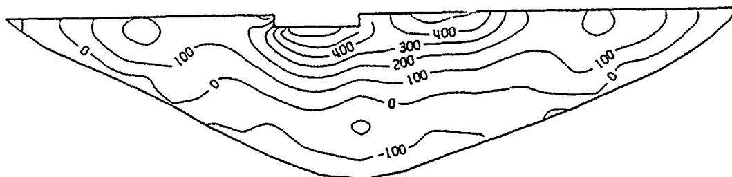
D/S ARCH STRESSES
