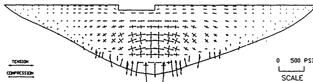
U/S Principal Stresses
