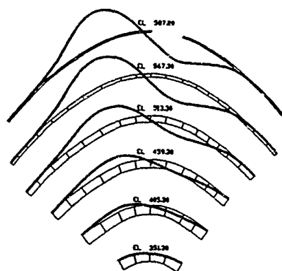
MODE-1 2.44 HZ
