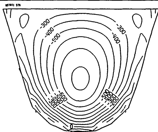
U/S Arch Stresses
