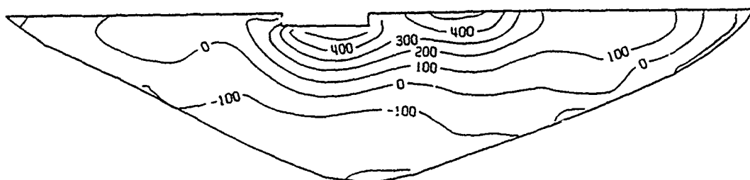
D/S ARCH STRESSES
