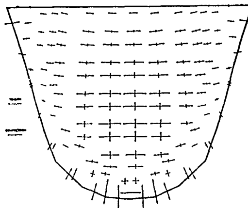
U/S Principal Stresses
