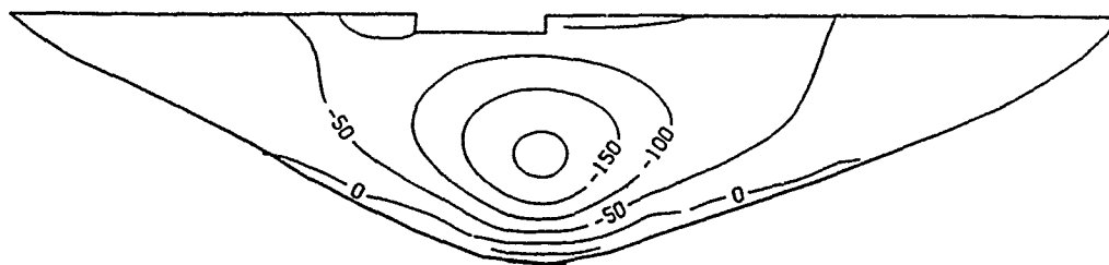
U/S ARCH STRESSES
