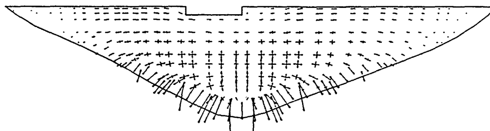
D/S Principal Stresses
