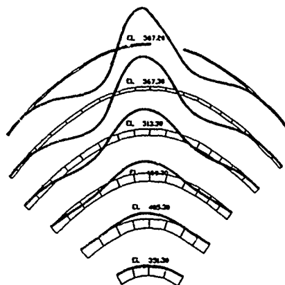
MODE-2 2.89 HZ
