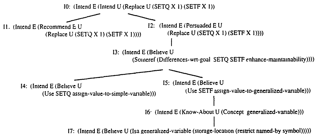
Figure 5: Intentional Structure of System's Utterance
