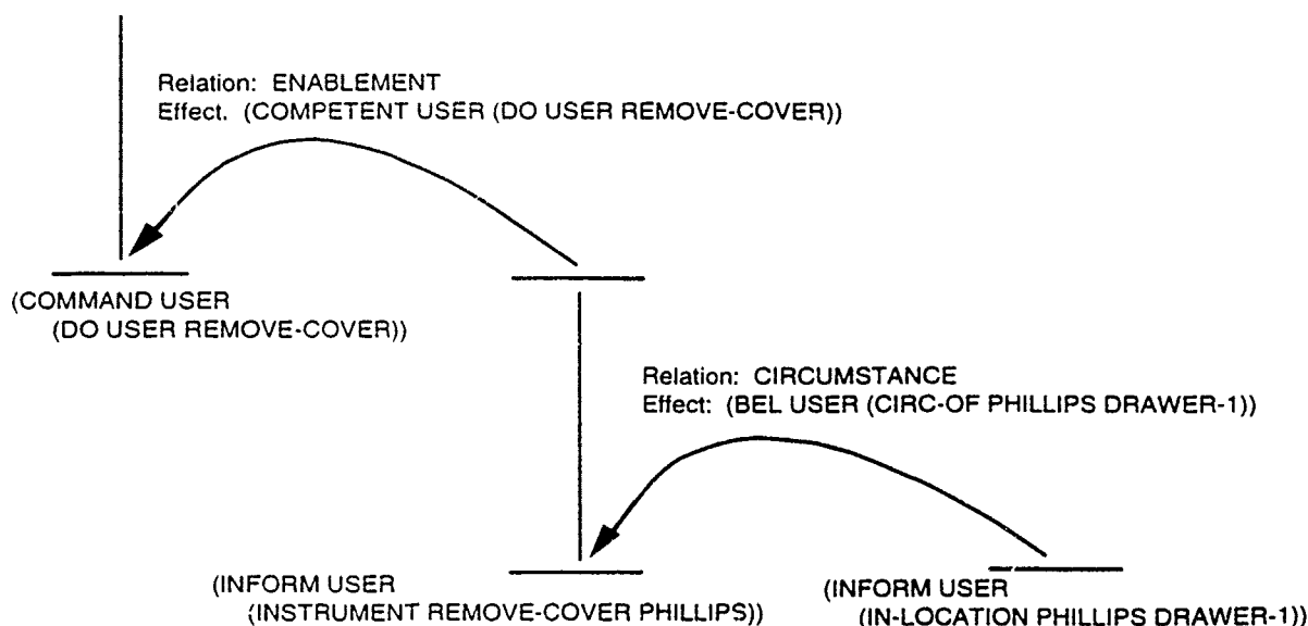
Figure 11: RST Tree for System's Utterance
