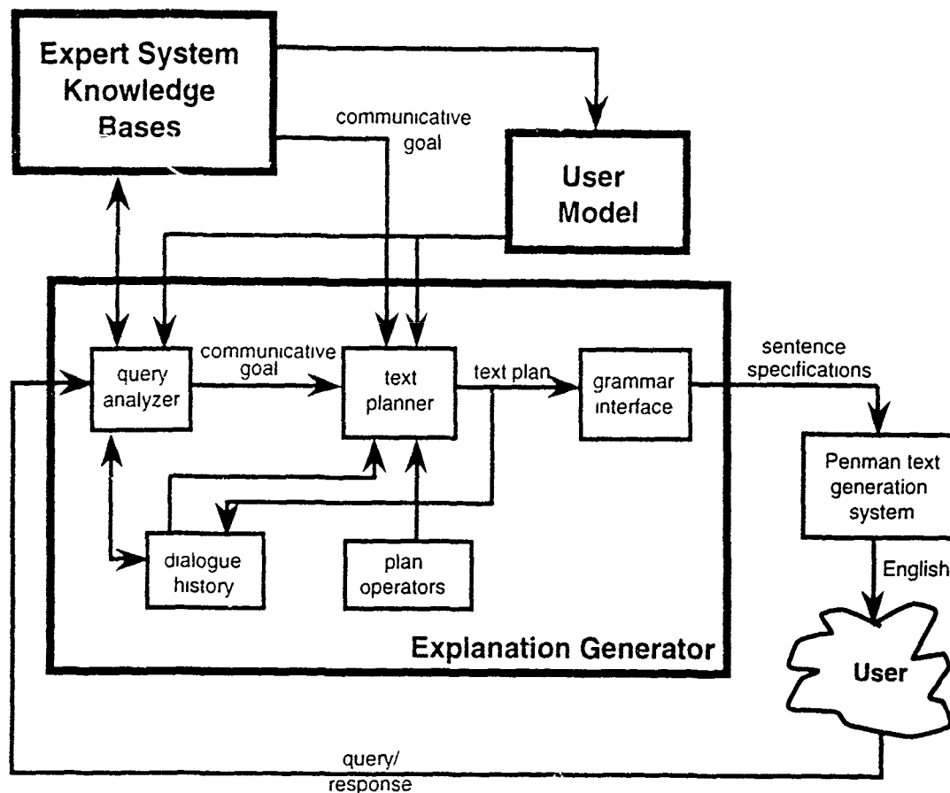
Figure 17: Architecture of Explanation System
