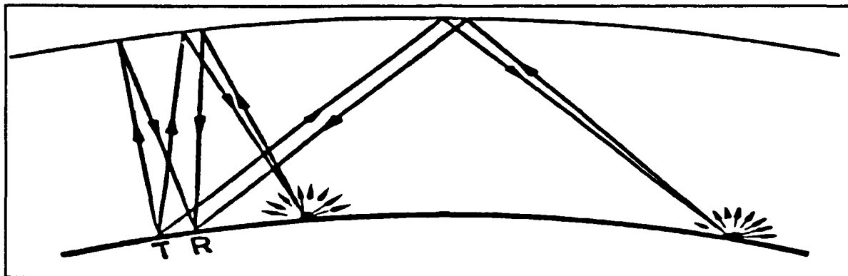
Figure 12 Example raypaths of the backscatter signal
