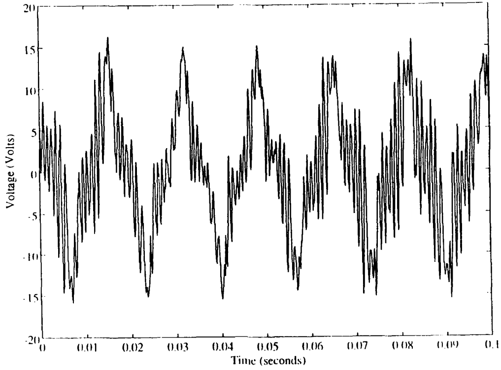
Figure 12a. Filter Voltage Without ASD.
