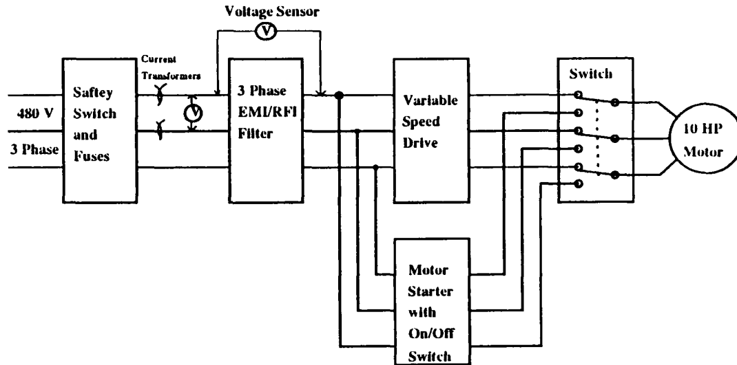
Figure 7. Experimental Apparatus.
