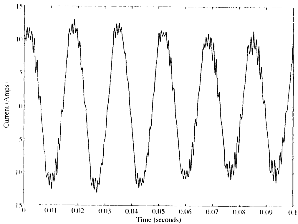
Figure 11a. Filter Current Without ASD.
