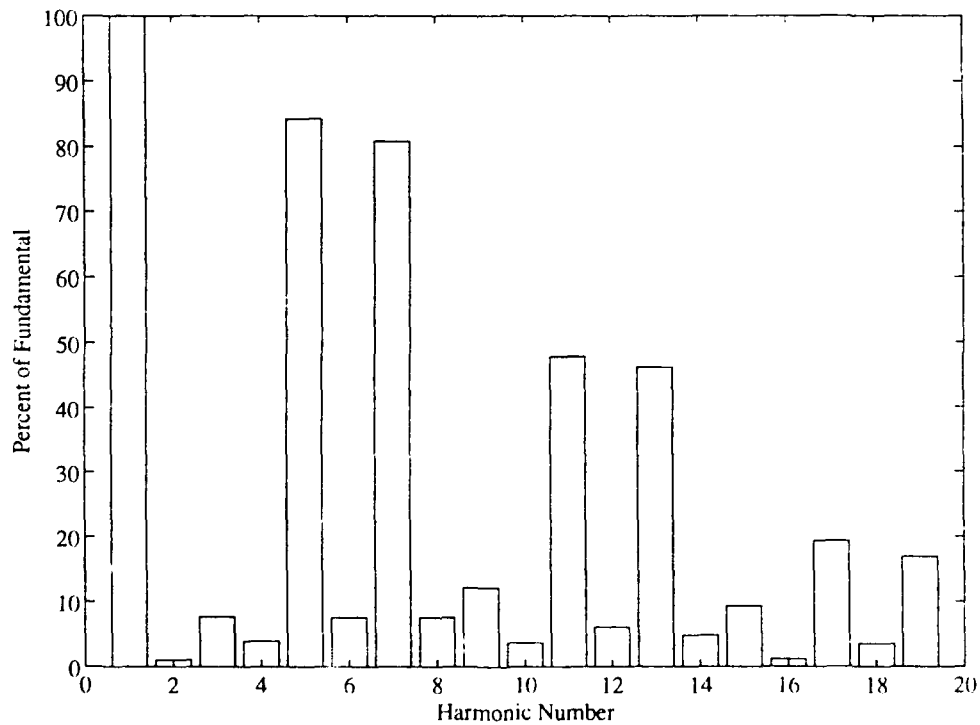
Figure 4. Current Harmonics From ASD.
