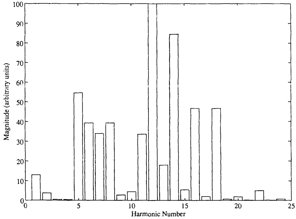
Figure 15. Filter Voltage Spectrum With ASD.
