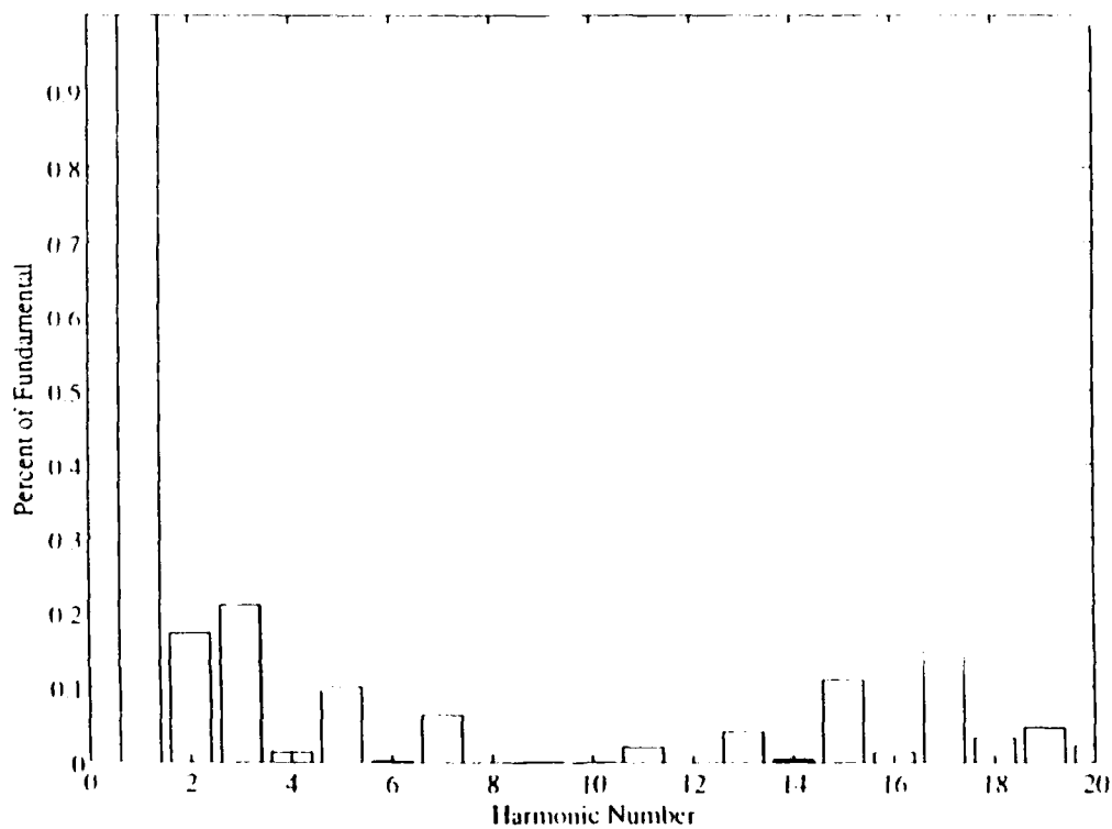
Figure 11b. Filter Current Spectrum Without ASD.
