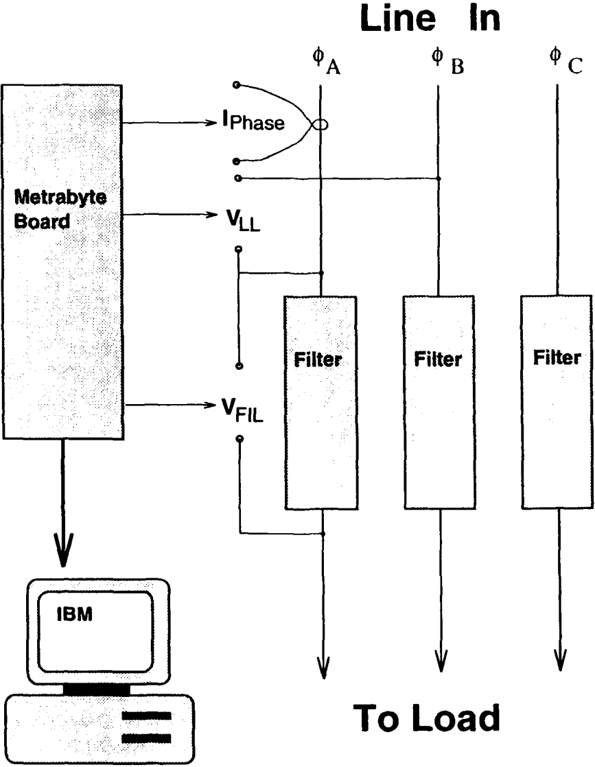
Figure 8. Data Acquisition System.
