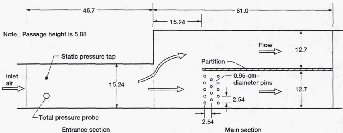
Figure 2.—Test section. (All dimensions given in centimeters.)
