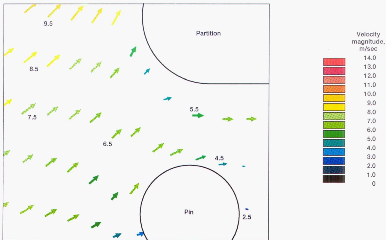
Figure 18.—Computational flow field map; Reynolds number, 45,000. Close-up. (Velocities given in m/sec.)
