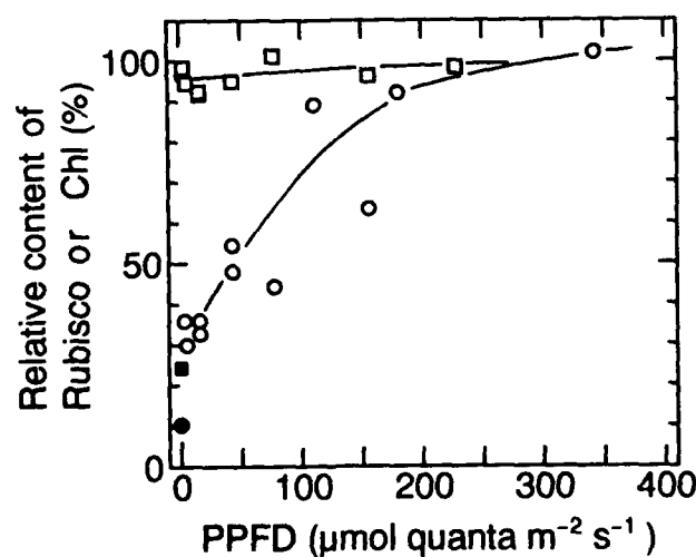
Figure 7. Effects of PPFD during the continuous illumination for 96 h on the degradations of Chl and Rubisco in attached 3rd leaves of Oryza sativa . At the onset of treatments, 3rd leaves were fully expanded. Original levels of Rubisco and Chl at the onset of the treatments are taken as 100%. Open and closed circles denote contents of Rubisco after the treatment for 96 h under continuous illumination, and in the dark respectively. Open and closed squares are for the data of Chl. Each symbol denotes a mean content of Chl or Rubisco measured in three leaves.
