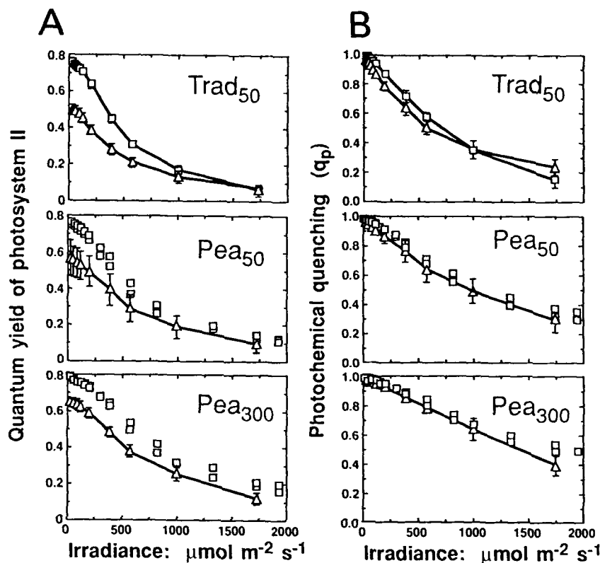
Figure 2. A. The quantum yield of PSII electron transport of non-inhibited ( \square ) and photoinhibited ( \Delta ) leaf discs, expressed as q_p \times F'_v/F'_m according to Genty et al. (16) plotted as a function of incident irradiance B. Photochemical quenching, q_p , of non-inhibited ( \square ) and photoinhibited ( \Delta ) leaf discs as a function of incident irradiance. Plants and photoinhibitory treatment as in Fig. 1. Redrawn from Öquist et al. (24).
