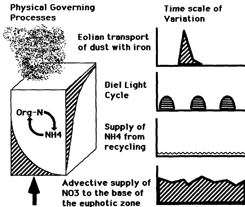
Figure 1. Variation of light, nitrogen sources and iron input to an open ocean water column.
