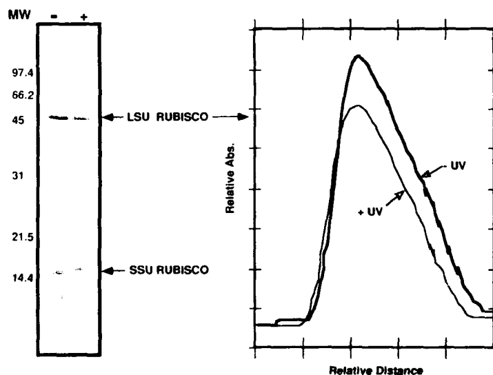
Figure 6. Comparisons of proteins isolated from microalgal samples from the UV exposed (+) and UV protected (-) tanks. Each lane was loaded with proteins from 0.5 \mu g Chl a of algal sample. Left Panel SDS-PAGE gel stained with Coomassie. Bands at 53 and 15 kD were identified as the LSU and SSU of Rubisco. Right Panel Densitometric scan of the gel LSU bands for samples from UV exposed (+UV) and UV protected (-UV) tanks. The integrated area under the curve is a relative measure of LSU protein per unit Chl, it is 20% less for sample from the UV exposed tank (From 39).
