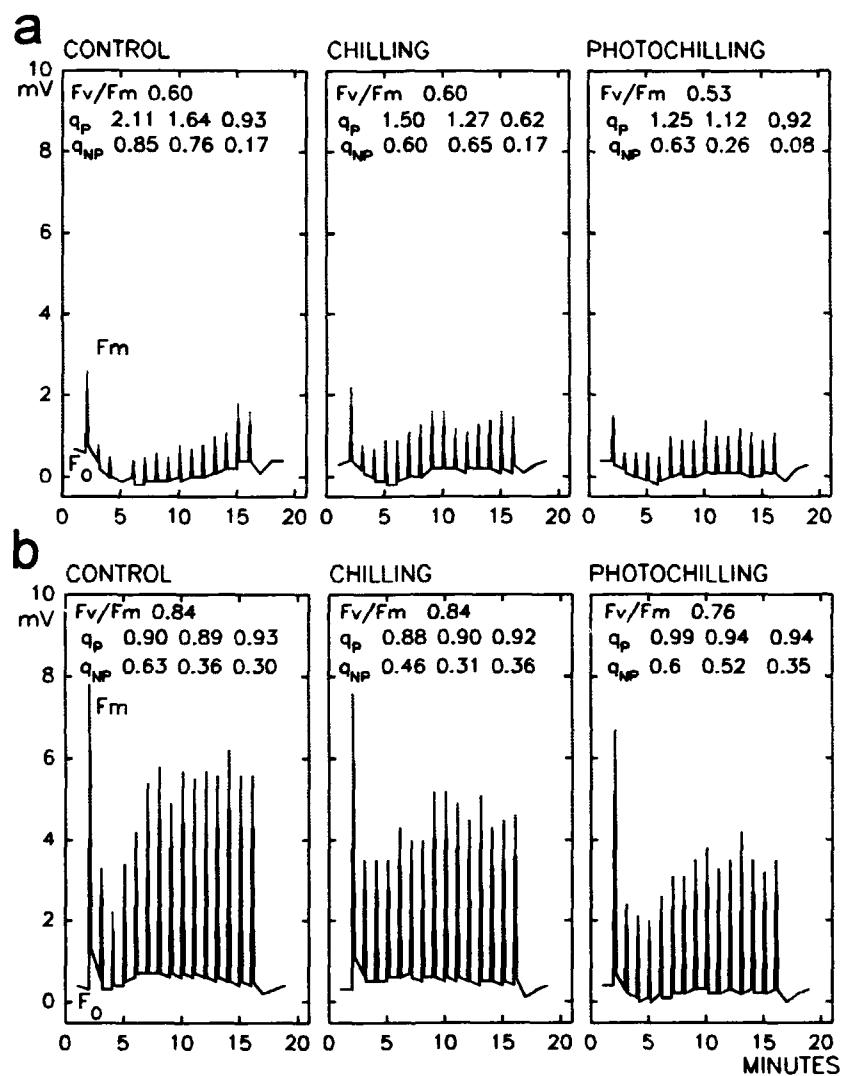
Figure 3. Quenching analyses, upper surface: F_v/F_m , photochemical capacity; F_0 , minimal fluorescence; F_m , maximal fluorescence; 3rd, 7th and 15th flash: q_p , photochemical quenching; q_{NP} , non-photochemical quenching. (a) February 1990; (b) April 1990
