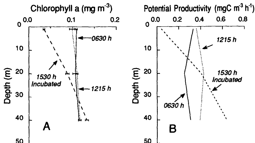
Figure 6. The artifacts associated with fixed-depth incubations during vertical mixing of the water column to about 50 m. These data are from a cruise in the equatorial Pacific Ocean (WEC88, 10°N, 150°W; Cullen and Lewis, unpublished). Solid lines are for samples from the morning bottle cast, dotted lines are for the midday cast, and the dashed lines are for samples from the morning cast, held in simulated in situ incubators until 1530 h in UVB-opaque polycarbonate bottles. Concentration of Chl (A); Potential productivity (B). Potential productivity was determined from short-term P-I measurements: it is maximal photosynthesis per unit Chl times the Chl concentration. When photoinhibition of photosynthesis occurs, potential productivity declines. If incubations mimicked nature, the incubated samples would show the same vertical patterns as the fresh afternoon samples. They don't. Instead, these data show severe photoinhibition during conventional incubations near the surface, resulting in massive net destruction of chlorophyll, even though UVB was excluded. Midday measurements on fresh samples suggest that vertical mixing moved the phytoplankton through the light gradient fast enough to protect them from such damage. This inference is supported by a calculation of photosynthesis in the mixed layer from P-I, Chl and PAR measurements: modeled productivity for incubated samples was 35% lower than for fresh samples. A conventional half-day experiment for assessing the effects of UV on photosynthesis under these conditions would be grossly compromised. It is possible that some inhibition of photosynthesis occurred near the surface and was averaged in by mixing. An upper bound to that process can be specified if the kinetics of damage and repair are known. Although the kinetics of photoinhibition and recovery have been incorporated into recent models of photosynthesis (13, 43, 45), neither the BWF/P-I model nor any other model of UV effects incorporates time-dependence in UV responses.
