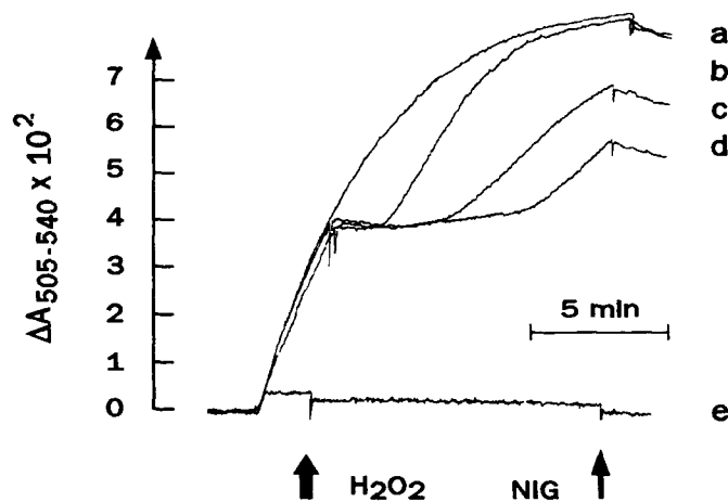
Figure 3. Effect of ascorbate and hydrogen peroxide ( H_2O_2 ) on light-induced 505-540 nm absorbance change. Ascorbate was present (30 mM; a-d) or absent (e) during actinic illumination; b, c, and d, addition of 0.1, 0.5 and 1.0 mM H_2O_2 , respectively. For further conditions see Fig. 1 and materials and methods.
