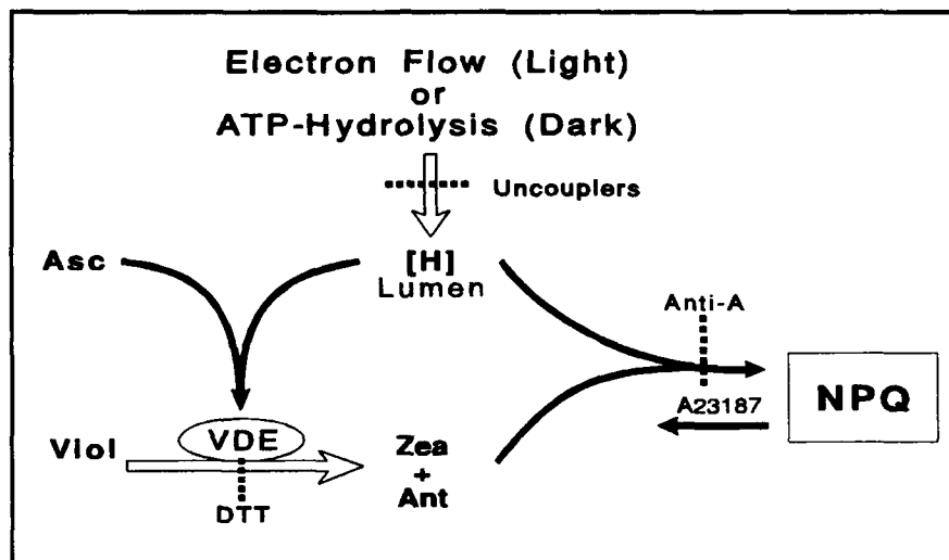
Figure 3. Schematic of the relationships of lumen pH, xanthophyll cycle, NPQ and the sites of inhibitor action.
