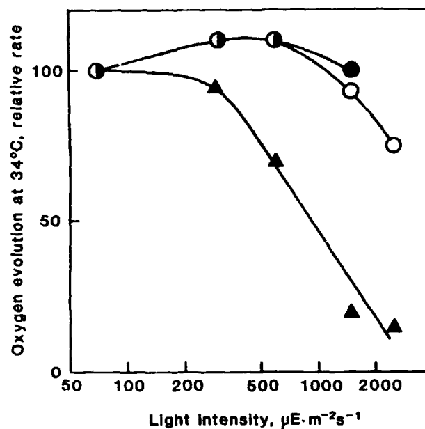
Figure 3. The effect of light intensity on photoinhibition of photosynthesis in wild type, Fad6 and Fad6/desA::Kmʳ of Synechocystis PCC6803. Cells were grown at 34°C. The symbols indicate wild type (O), Fad6 (●) and Fad6/desA::Kmʳ (Δ). The activity of photosynthesis was measured at 34°C and the activity of 100% corresponded to 320, 330 and 310 \mu\text{mol O}_2 \text{ mg Chl}^{-1} \text{ h}^{-1} in wild type, Fad6 and Fad6/desA::Kmʳ, respectively.
