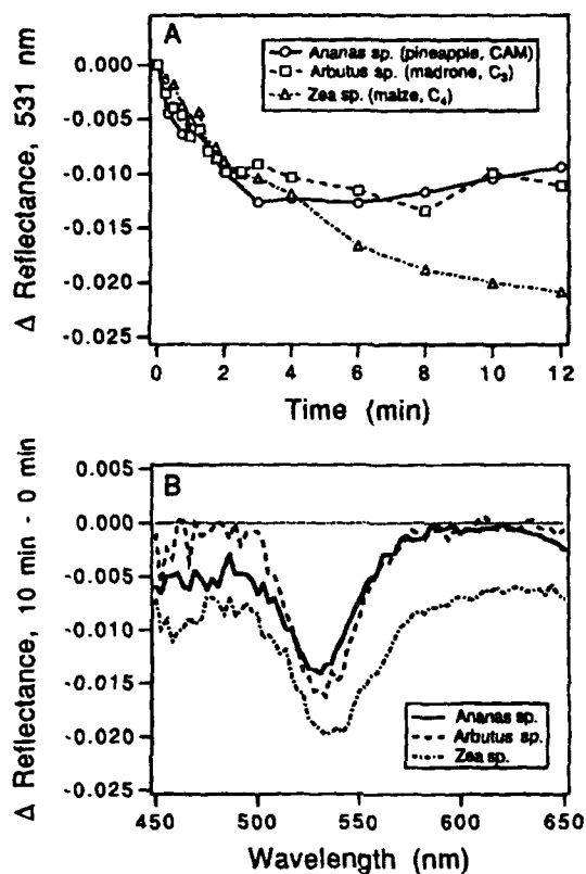
Figure 1. A. Time course of \Delta reflectance upon sudden high-light exposure of dark-adapted leaves representing 3 photosynthetic pathways ( C_3 , C_4 and CAM). Reflectance has been normalized to reflectance at time zero. Each curve represents measurements of a single leaf. B. The spectral dependence of the \Delta reflectance signal (calculated by subtracting reflectance at time zero from reflectance at 10 minutes). Each spectrum represents the mean of 3 leaves. Note the shift in "background reflectance" in Zea mays , possibly due to chloroplast movement.
