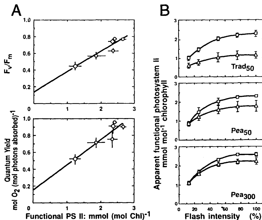
Figure 1. A. Correlation of the maximum efficiency of PSII photochemistry ( F_v/F_m ) with the quantum yield of \text{O}_2 evolution and numbers of functional PSII reaction centers in non-inhibited and photoinhibited leaves. B. The apparent number of functional PSII reaction centers ( \text{mmol mol}^{-1} \text{Chl} ) as a function of relative flash intensity in non-inhibited and photoinhibited leaf discs. Tradescantia albiflora (Trad 50 ) and peas (Pea 50 ) were grown at 50 \mu\text{mol photon m}^{-2} \text{s}^{-1} and peas (Pea 300 ) at 300 \mu\text{mol photons m}^{-2} \text{s}^{-1} . Standard photoinhibitory treatments were given to leaf discs floating on water at 22°C under 1,700 \mu\text{mol photons m}^{-2} \text{s}^{-1} for 4 h. Replotted from Öquist et al. (24).
