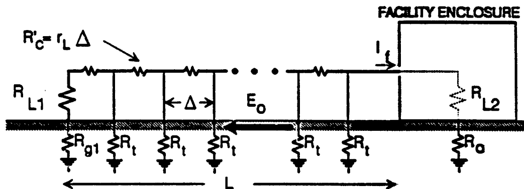
Figure 4-5. Configuration of a single line periodically connected to earth.
