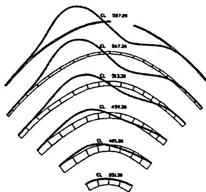
MODE-1 2.44 HZ
