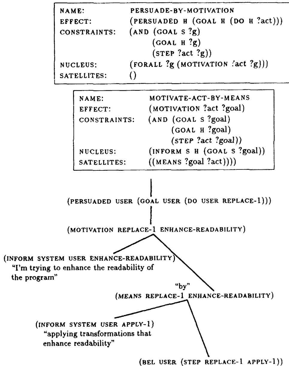
Figure 6: Example text plans and discourse structure fragment from the EES planner, [Moore 89].
