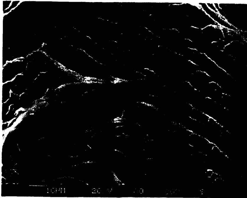
Figure 42. Micrograph showing fatigue striations in the central region of the fracture surface.
