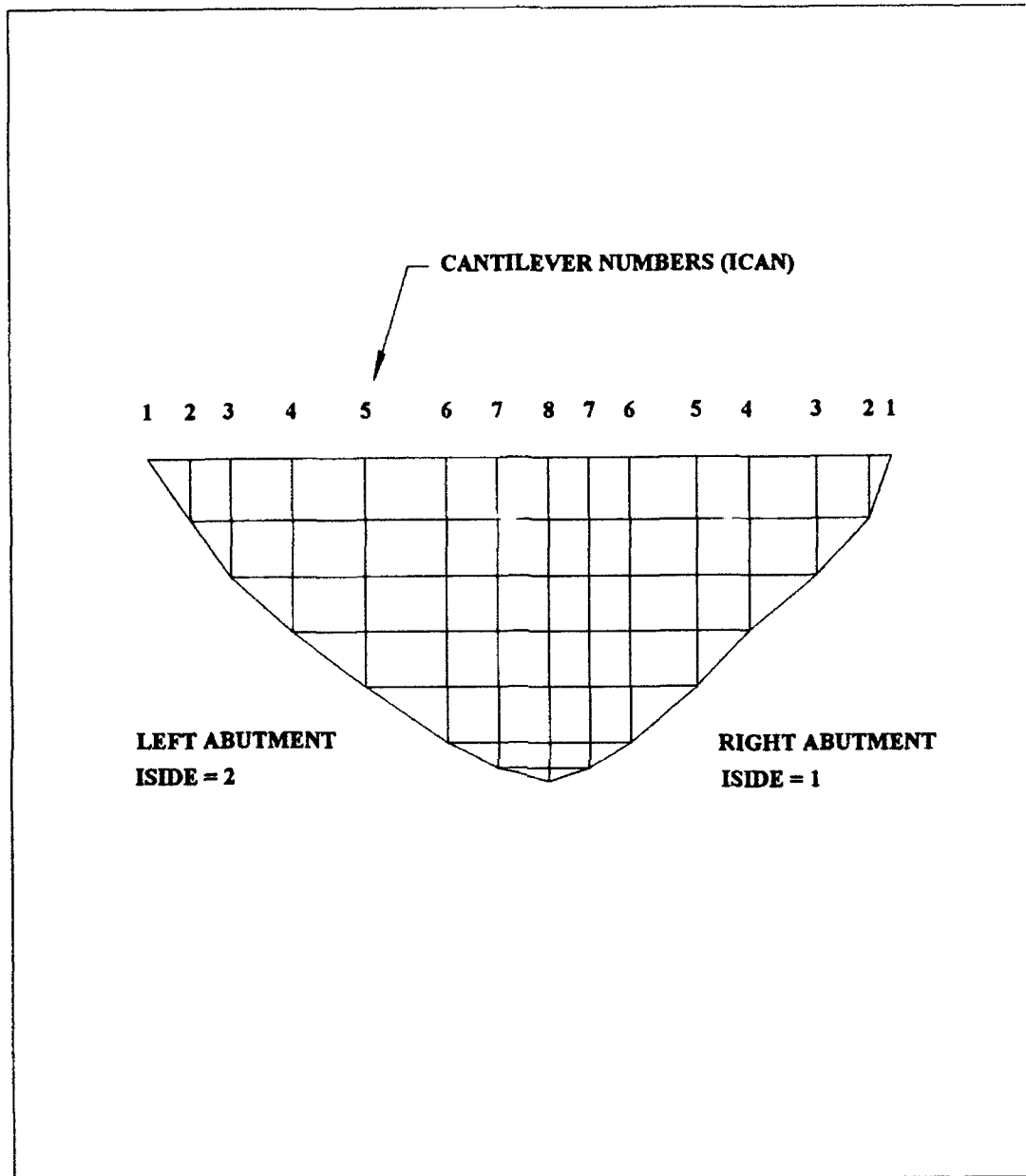
Figure 6.6 Cantilever Numbers
