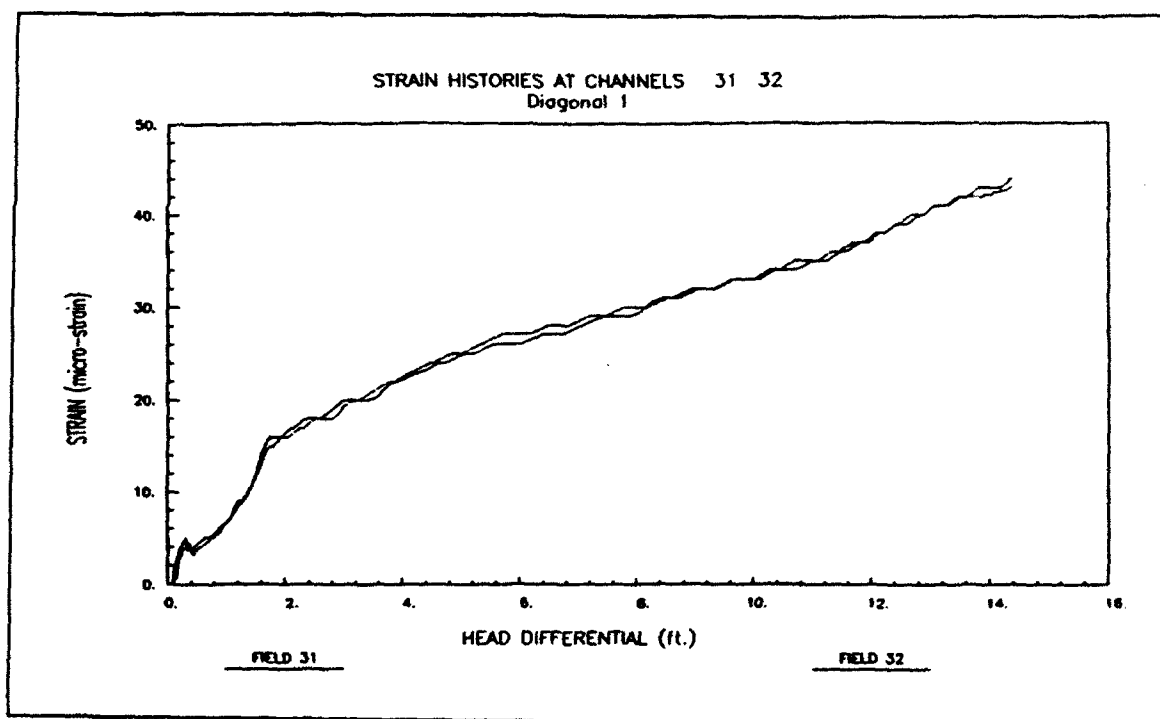
Figure A16. Head differential test strain: diagonal 1
