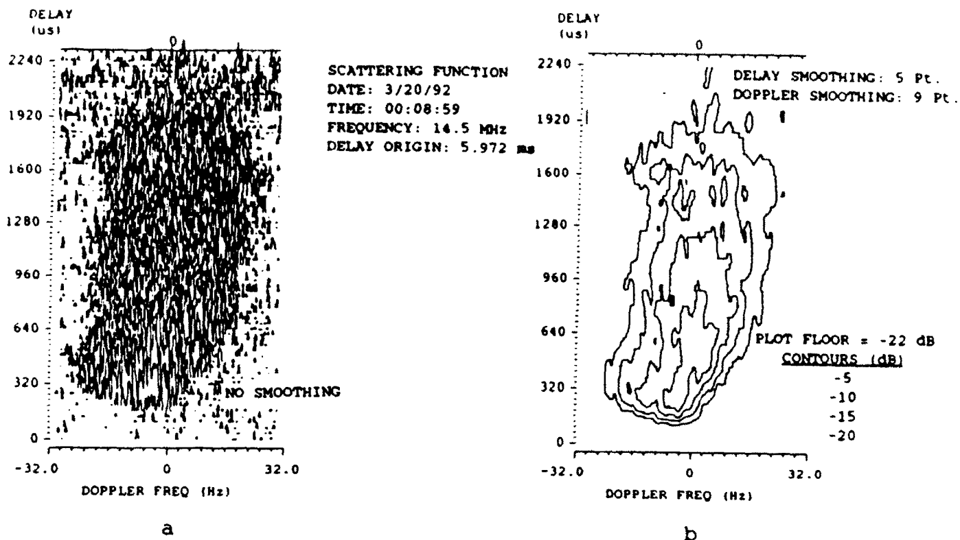
Fig. 7 - scattering function for midnight slant F scatter signal; trans-auroral channel; 14.5 MHz.
