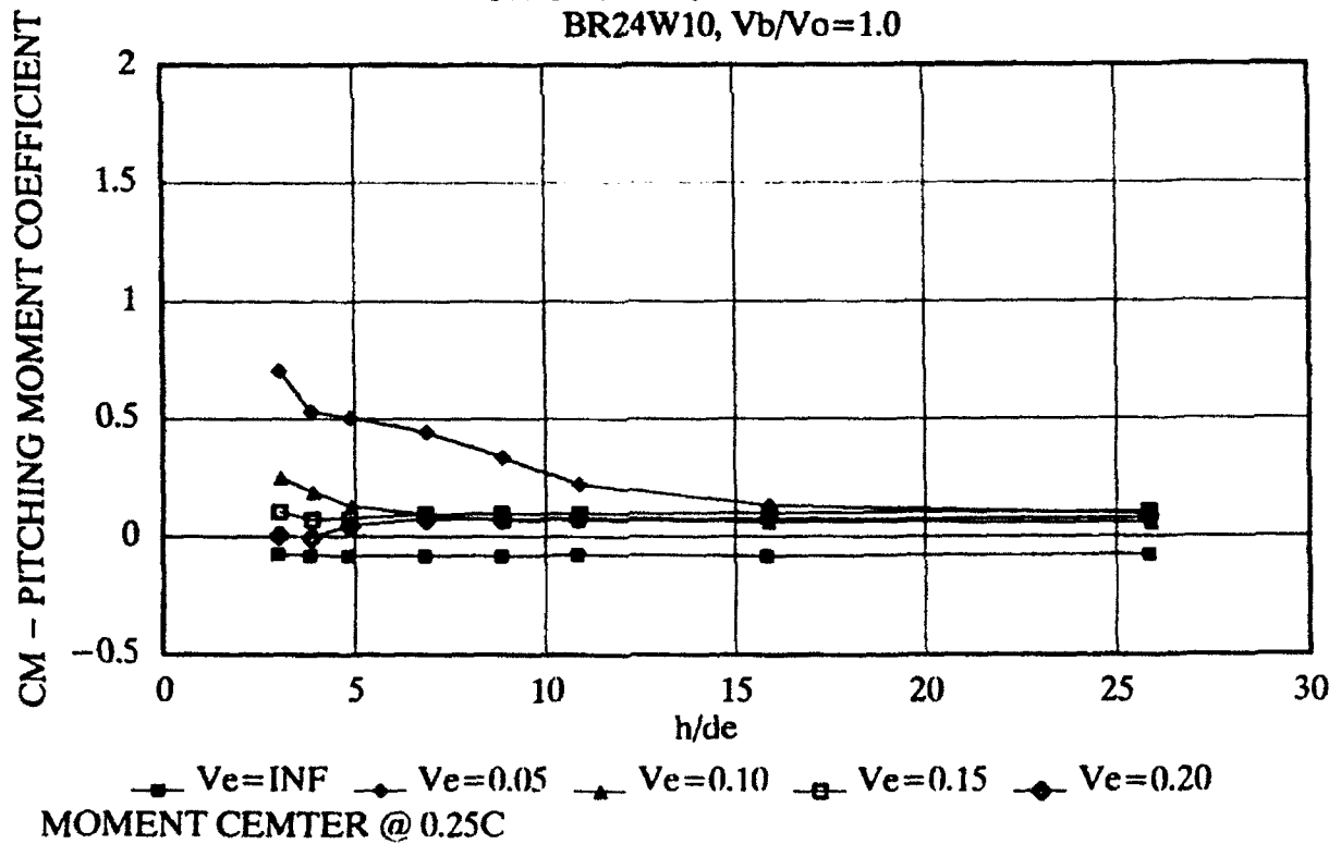
Figure 35. Variation of Aerodynamic Characteristics with Height, BR24W10, V_b/V_o=1.0
