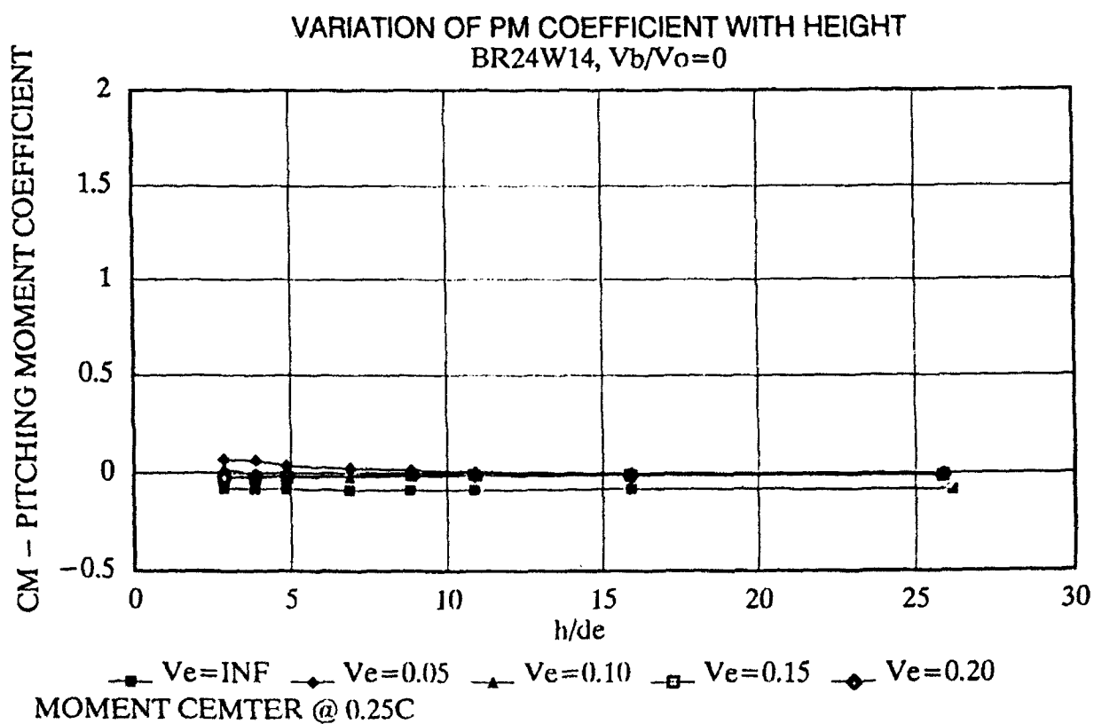
Figure 36. Variation of Aerodynamic Characteristics with Height, BR24W14, V_b/V_o=0
