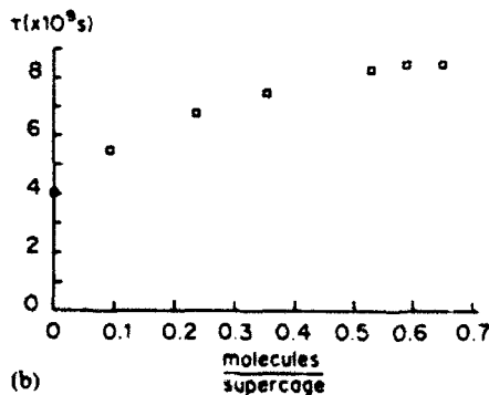
Fig. 7. (a) Experimental (full lines) and computed (dashed lines) EPR spectra of 0.011 TEMPO molecules per supercage adsorbed into NaX zeolite (hydrated at about 15 water molecules per supercage) at different loadings of DummyT (see text), indicated as molecules per supercage. (b) Correlation time for motion as obtained from computation of the spectra as a function of DummyT loading in molecules per supercage.
