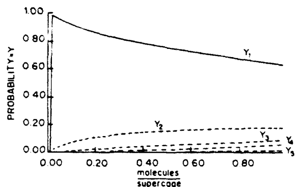
Fig. 6. Relative averaged probabilities that TEMPO molecules occupy isolated cavities or two, three, four, and five close cavities (these probabilities are indicated as y_1, y_2, y_3, y_4, and y_5 respectively) as a function of the occupancy (molecules per supercage).
