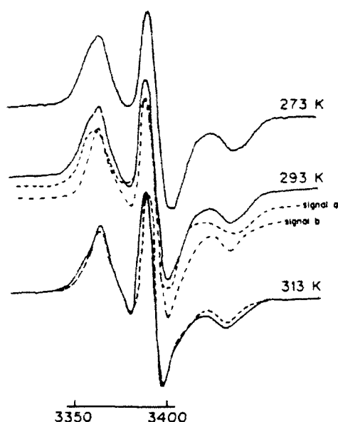
Fig. 1. Experimental (full lines) and computed (dashed and dotted-dashed lines) EPR spectra of 0.011 TEMPO molecules per supercage adsorbed into dehydrated NaX zeolite at different temperatures.
