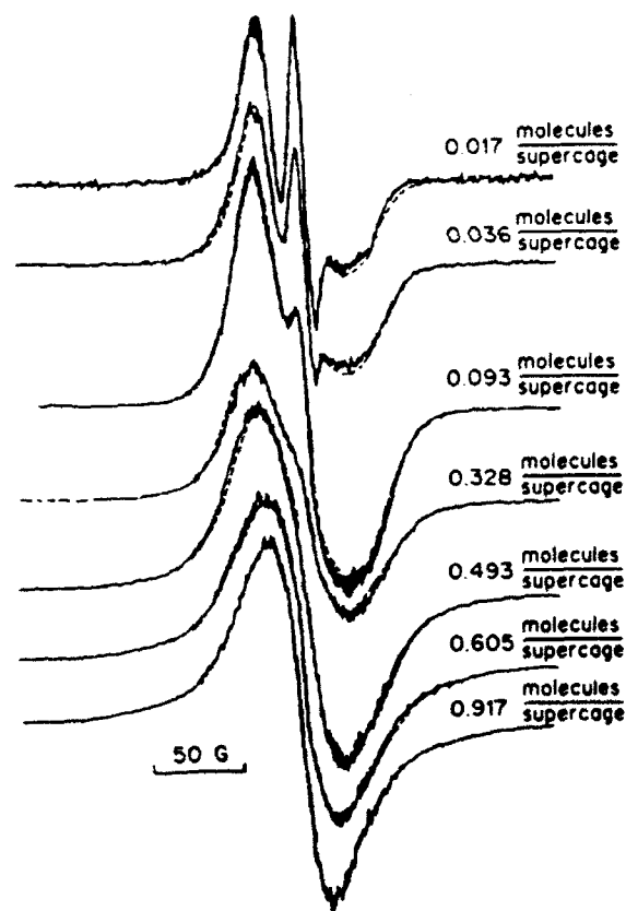
Fig. 4. Experimental (full lines) and computed (dashed lines) EPR spectra of NaX zeolites (hydrated at about 15 water molecules per supercage) at different TEMPO loadings, indicated as TEMPO molecules per supercage.
